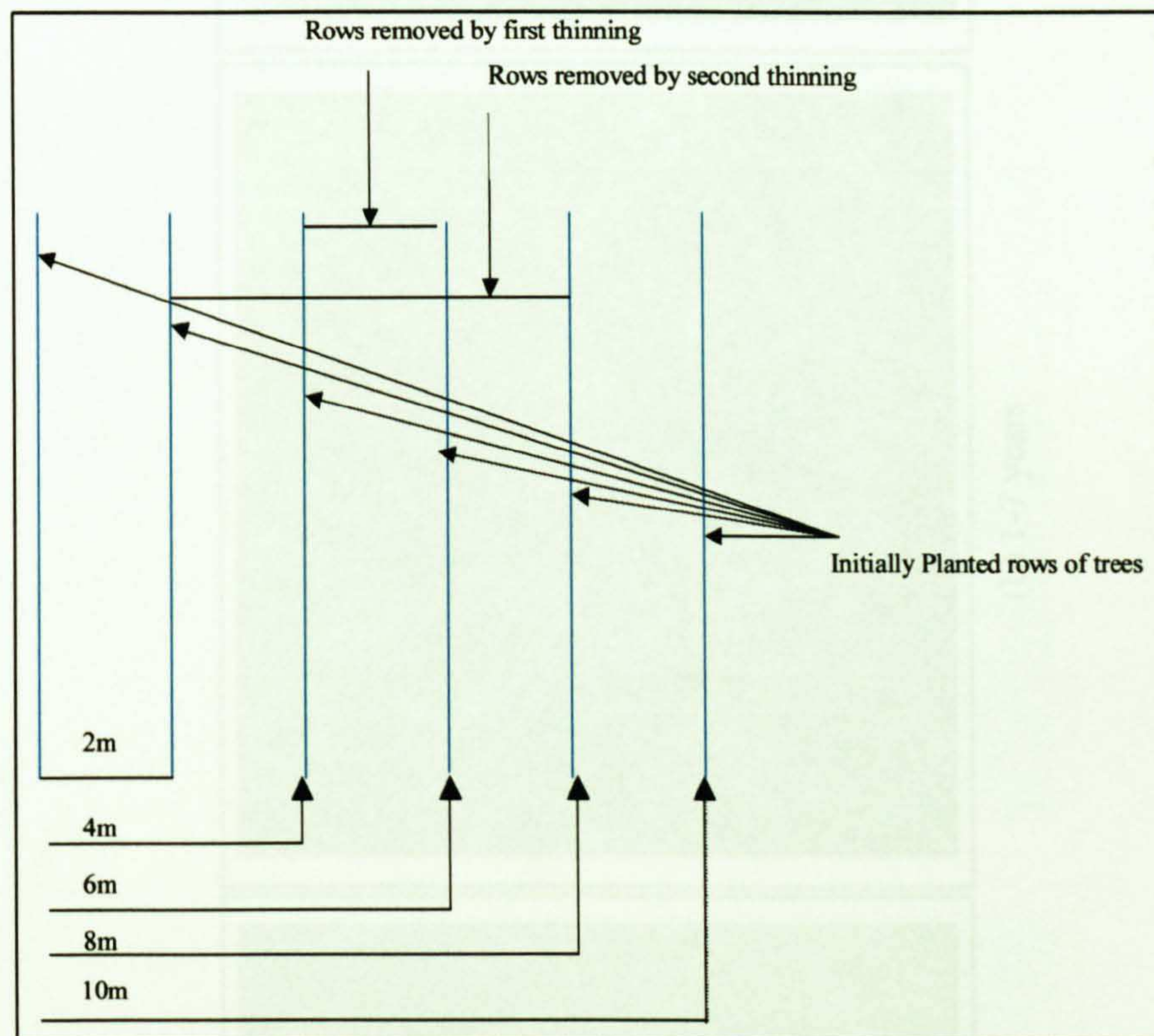
Figure 5.11 Systematic way of removal of rows of trees in thinning operations in the study site (created information gathered from forest manages)
