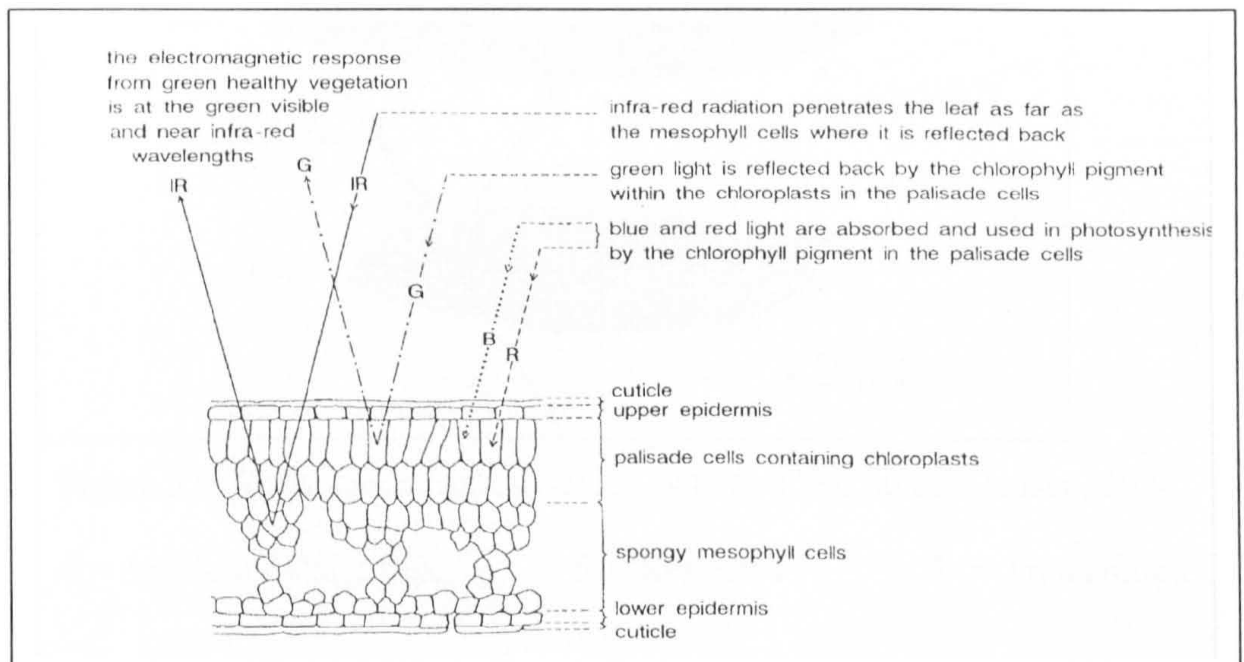
Figure 3.8: Spectral responses from different cell layers. (Campbell, 1996)
