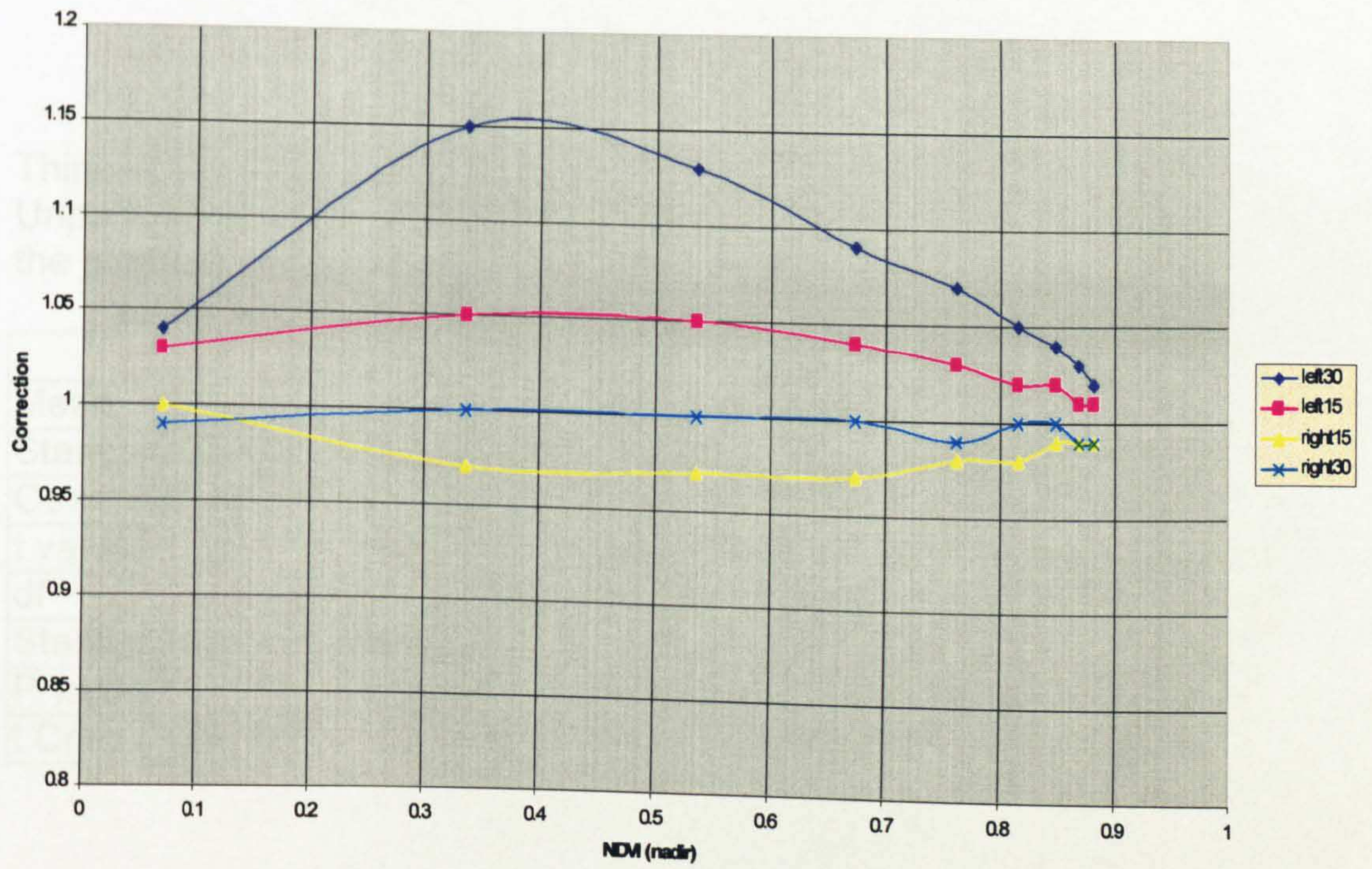
Figure FII: Correction values of NDVI
