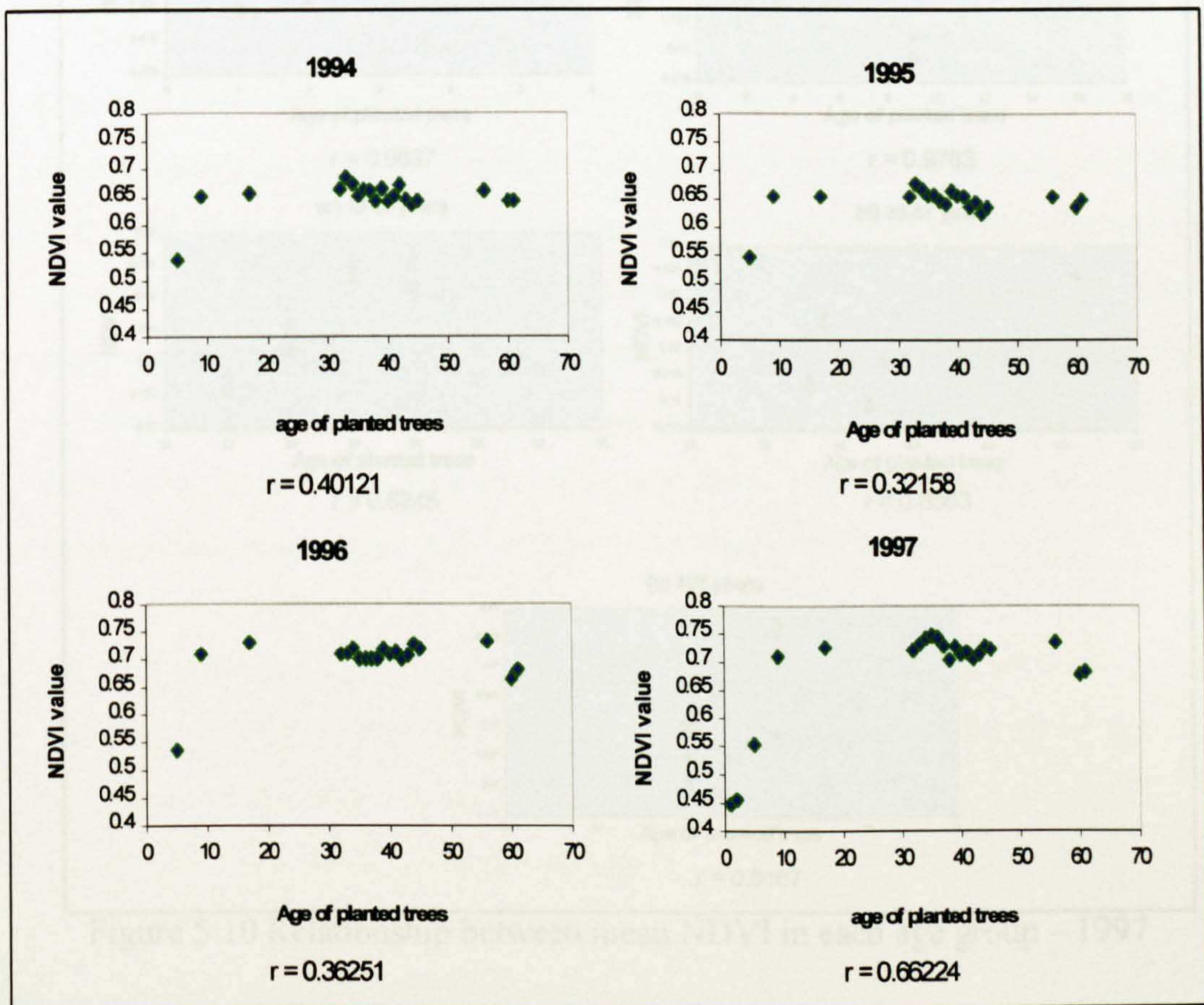
Figure 5.9 Relationship between NDVI and age (1994-1997)
