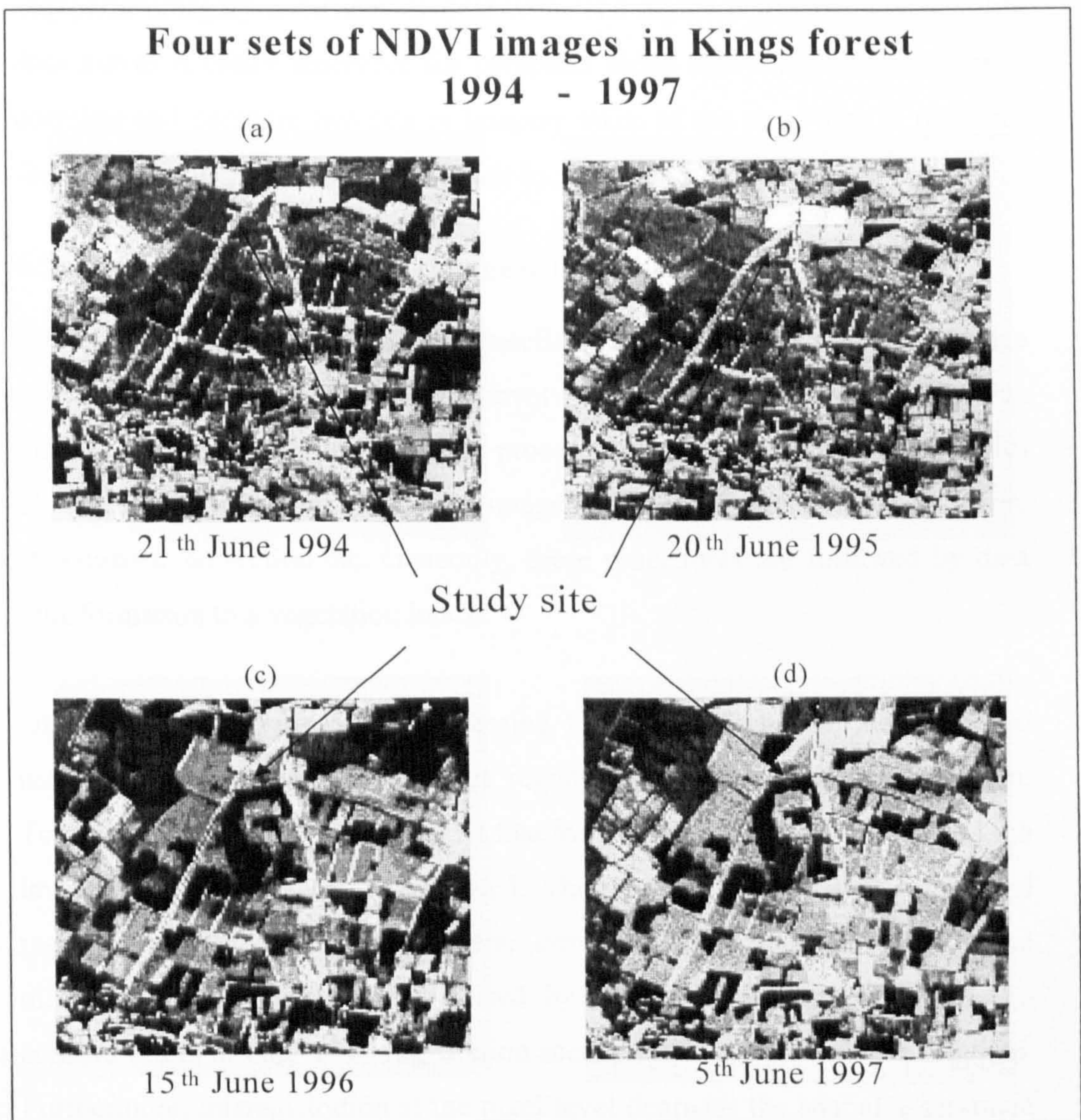
Figure 4.15: Four sets of NDVI images of the Kings Forest
