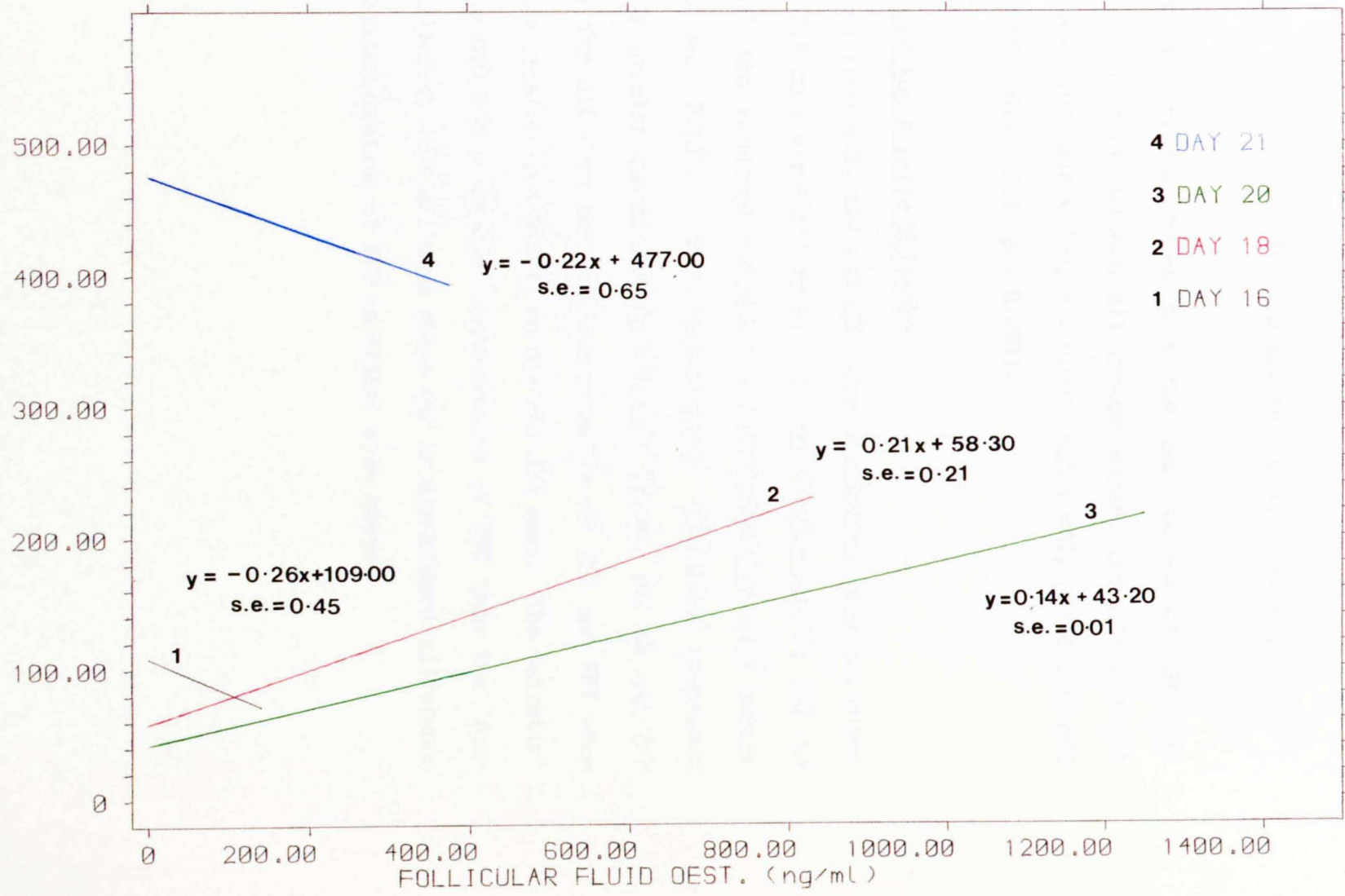
EXPT1:REGRESSION ANALYSIS. FF E2 (ng/ml) v FF P (ng/ml)
