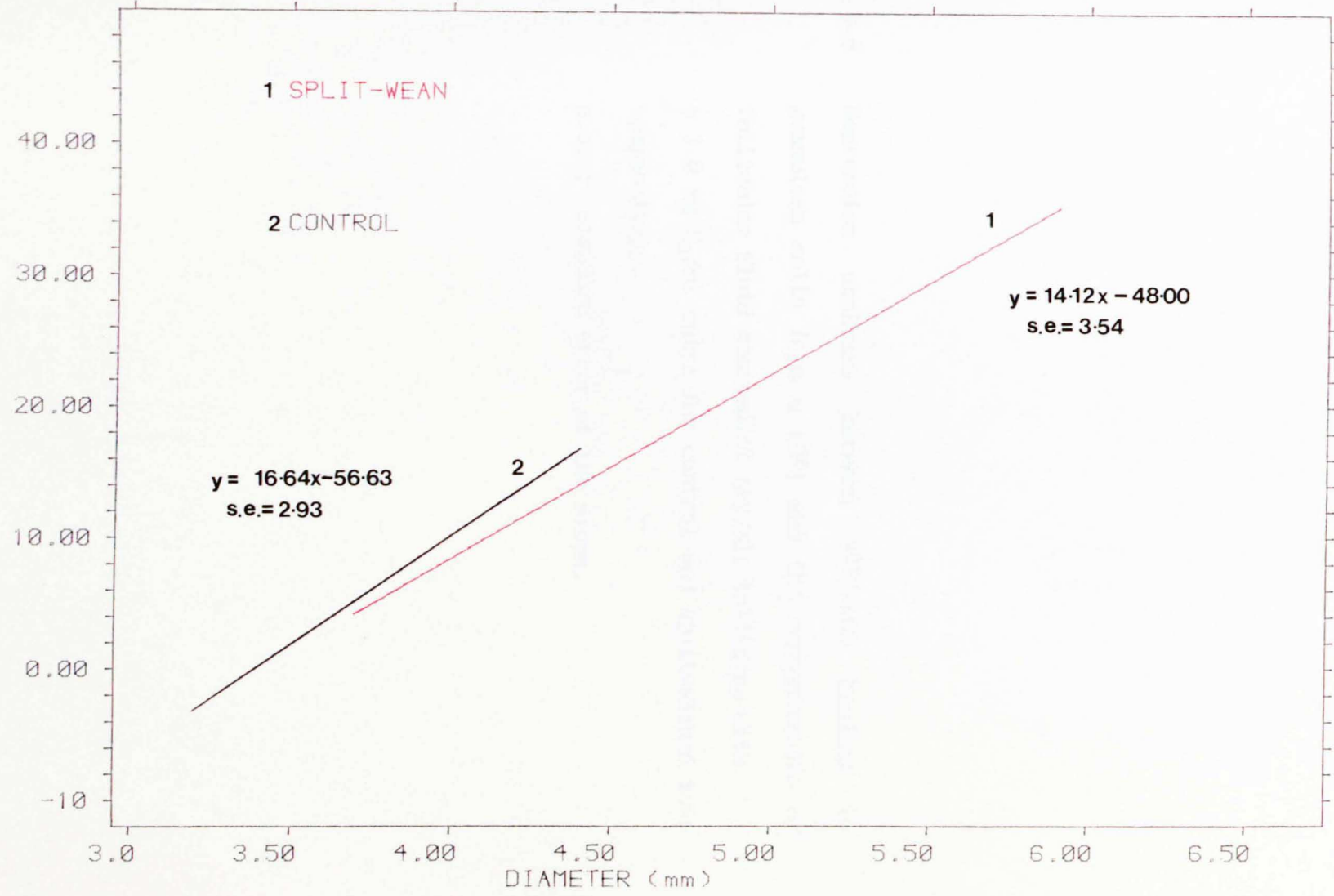
EXPT3:REGRESSION ANALYSIS DIAMETER(mm) v GRAN.BIND.(cpm x 10 3 /POLL)
