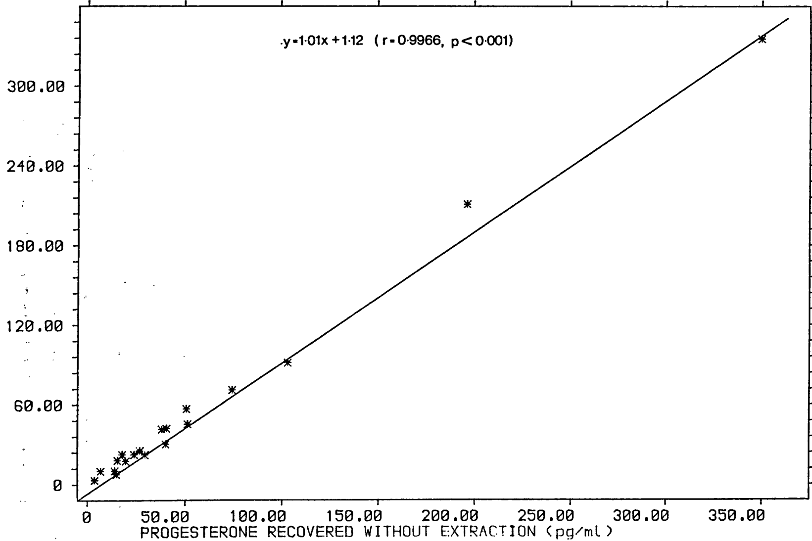
PROGESTERONE RECOVERED WITH AND WITHOUT EXTRACTION (pg/ml)
