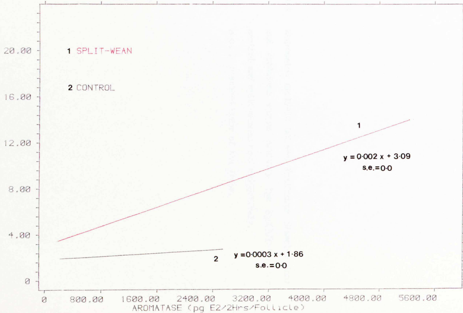
EXPT3:REGRESSION ANALYSIS AROM (pgE2/2Hrs/Follicle) v FF E2 (ng/ml)
