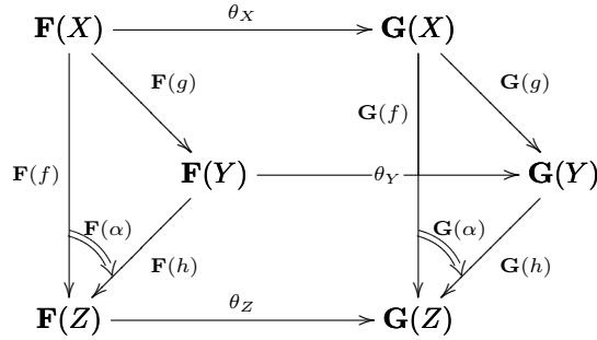
Figure 2.9: A 2-natural transformation \theta : \mathbf{F} \Longrightarrow \mathbf{G}
