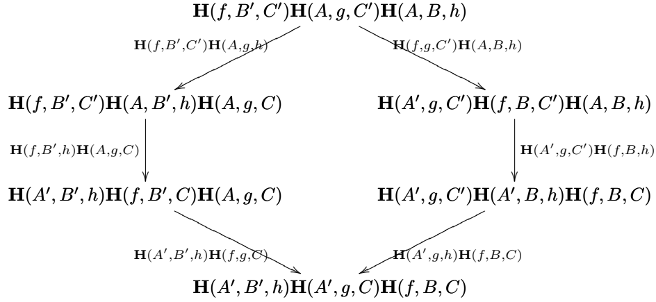
Figure 4.4: Yang-Baxter equation
