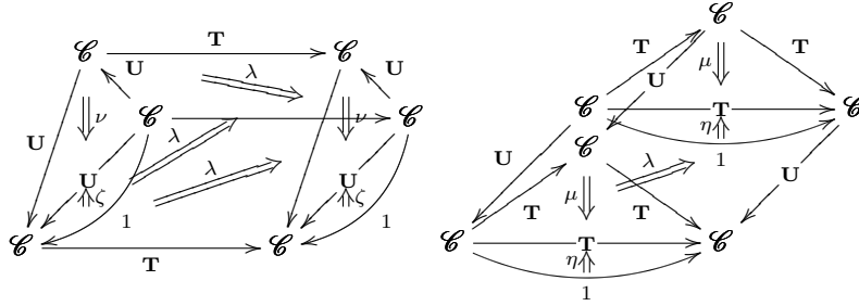
Figure 4.2: Distributive law \lambda : M \otimes M \rightarrow \text{Cat} of a monad over a monad.
