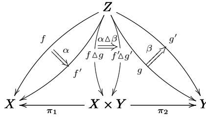
Figure 2.8: Product X \times Y of X, Y , in \mathcal{H}
