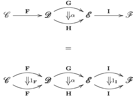
Figure 2.2: Horizontal composition and identities
