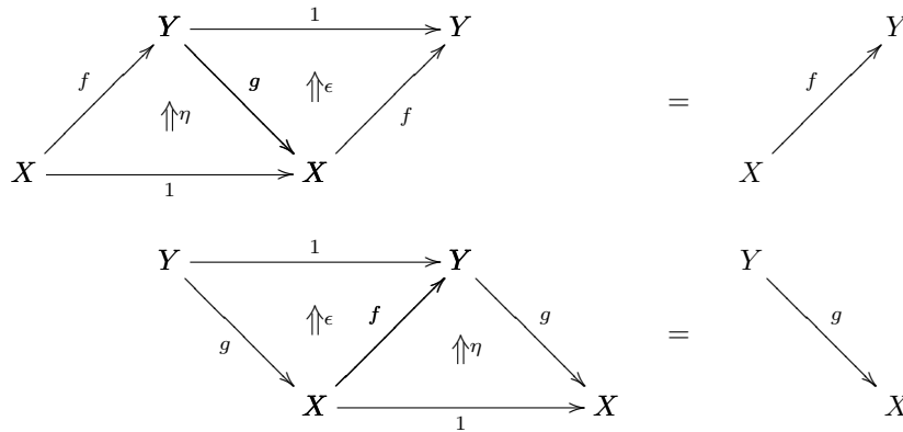
Figure 2.7: The triangle identities in a 2-category
