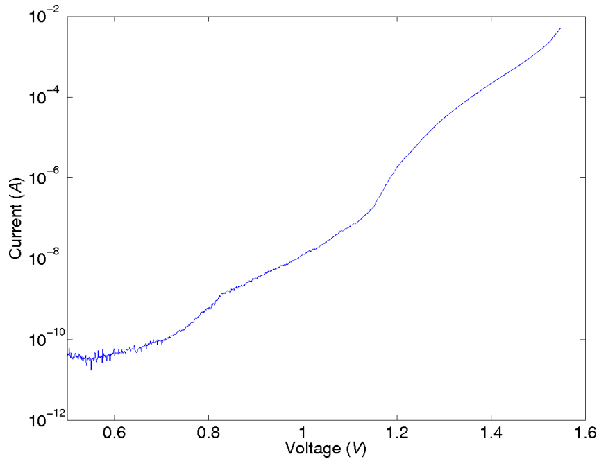
Figure 6.1: I(V) plot for sample B1 device at T=1.8 K.
