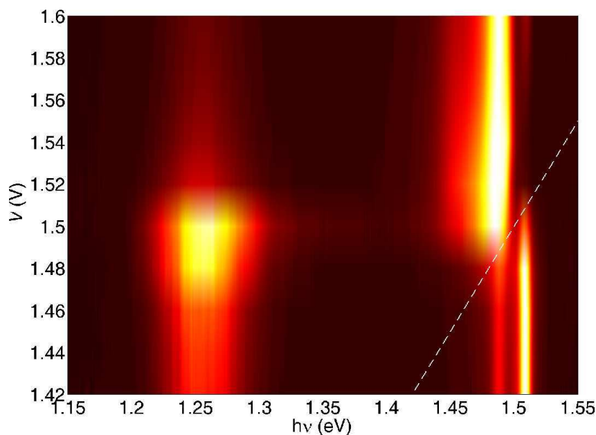
Figure 6.9: Colour-scale plot of the EL intensity vs V and h\nu for a device based on sample B1 at T=3.6\text{K} . The dashed white line represents the condition h\nu=eV .
