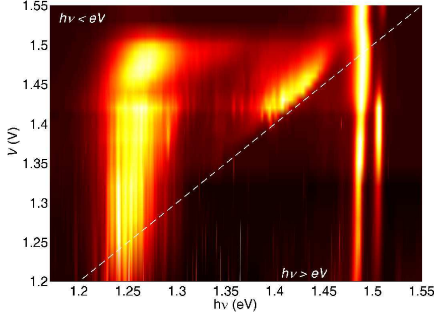
Figure 6.4: Colour-scale plot of the EL intensity vs V and emitted photon energy ( h\nu ) for sample B1 at T=3.6 K. The dashed white line represents where condition h\nu=eV .
