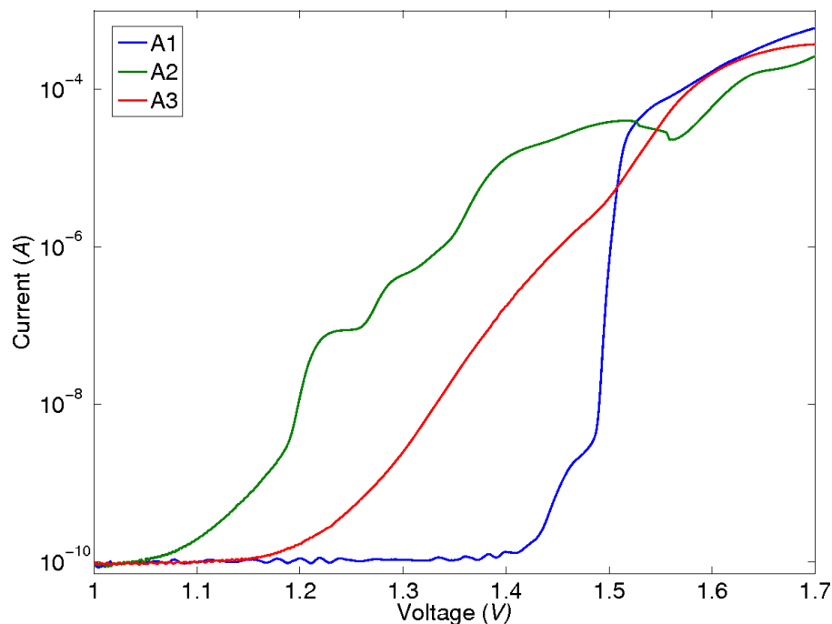
Figure 4.4: I(V) curves at 4.2K for sample A1 (blue), A2 (green) and A3 (red). The noise level in the experiment was \sim 100 pA.
