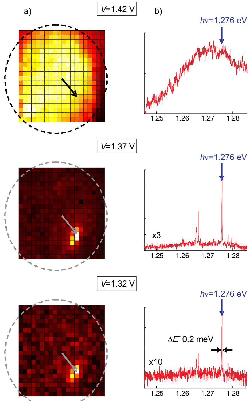
Figure 5.9: a) \mu EL images for sample B3 at T \sim 15 K. Each pixel has length l=10 \mu\text{m} and the dashed circular line illustrates the mesa boundary. b) EL spectra from the pixel indicated by the arrow. The applied bias is shown for each figure.
