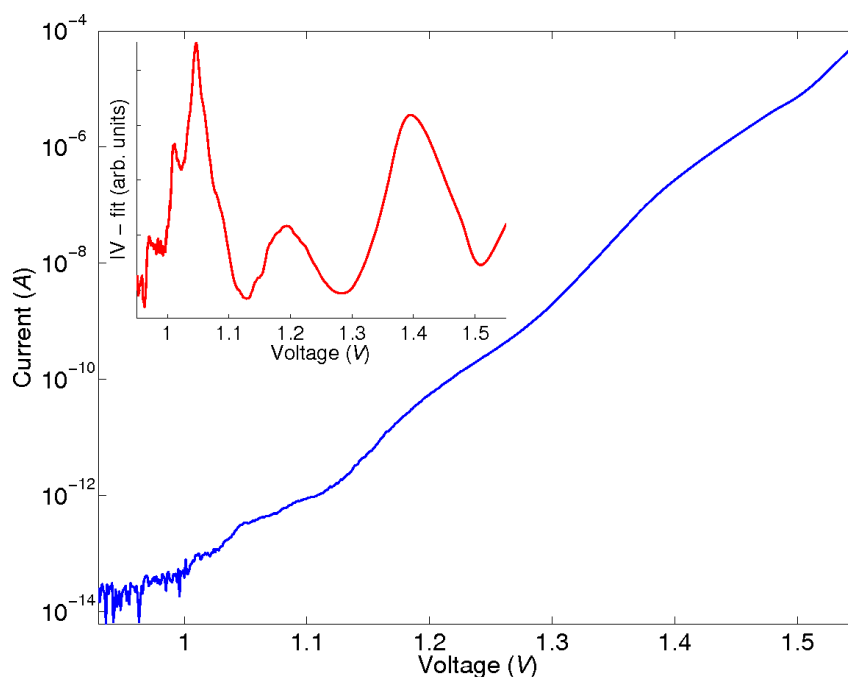
Figure 4.7: 1.8K high sensitivity I(V) curve for sample A3. The inset shows the same I(V) data with an fitted exponential, I_f = A e^{\beta V} , subtracted. The data is then scaled by the current of the fitted I(V) .
