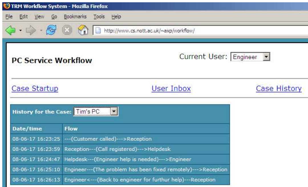
Figure 7-7: A sample Case History screen in TWM
