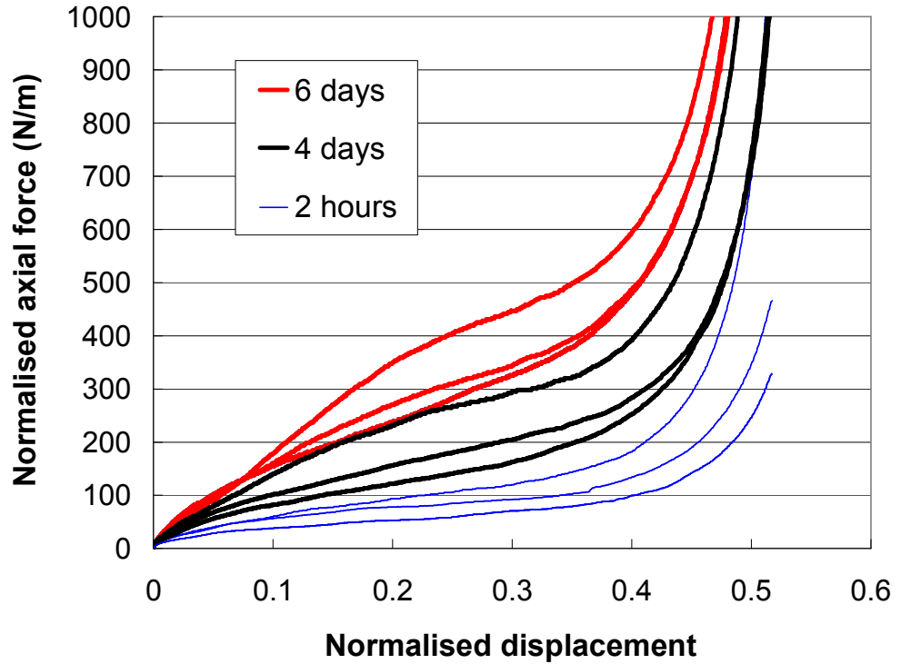
Figure 5.5. Aging tests with three different aging times, 2 hours, 4 days and 6 days respectively, in PF tests for automotive prepregs. Tests were performed at room temperature with a displacement rate of 0.11 \text{ min}^{-1} .
