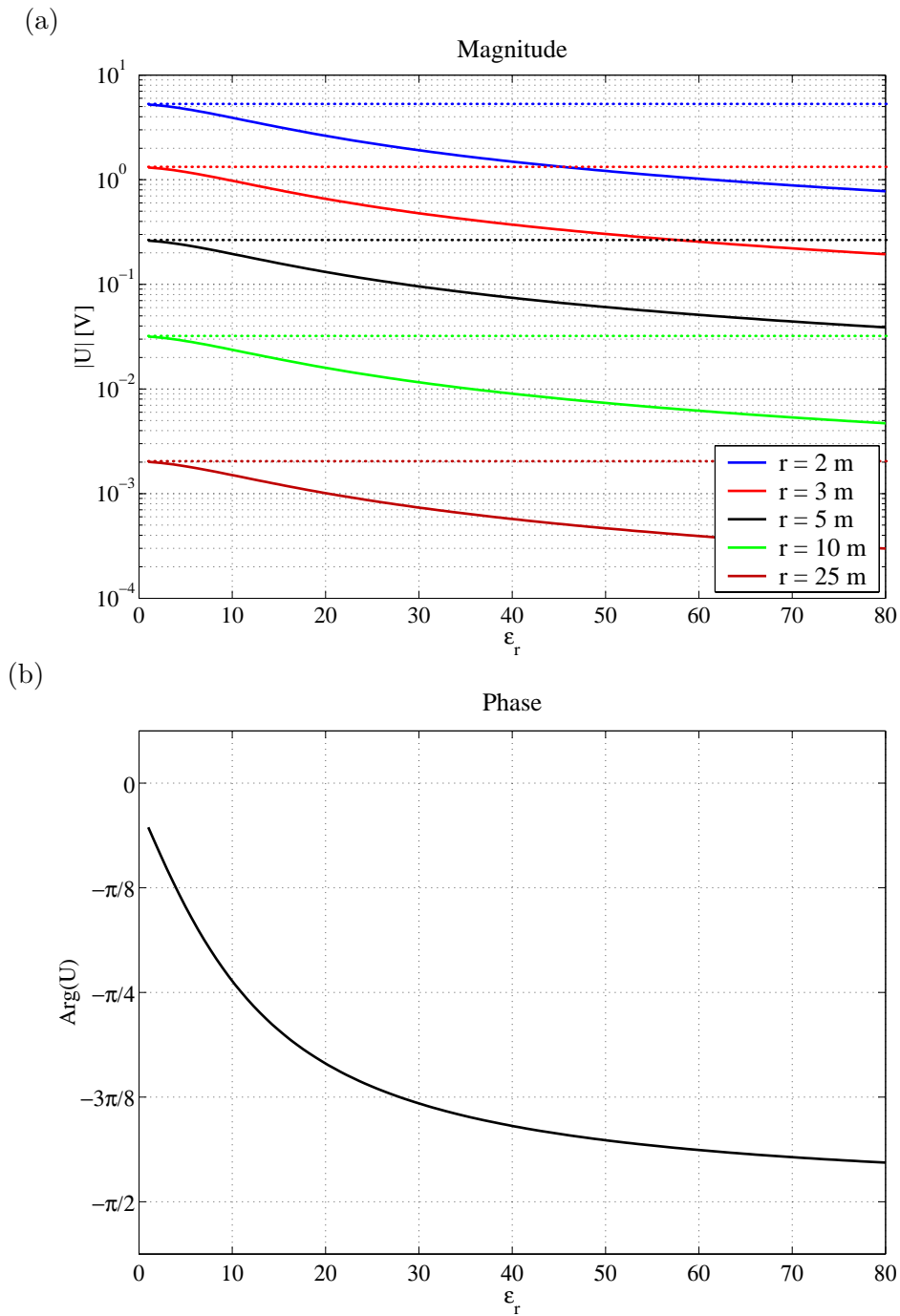
Figure 5.9: Variation of the complex potential with relative permittivity for a capacitive array in inline configuration. Parameter: dipole separation r . Dipole length l = 1\text{m} , array elevation h = 1\text{mm} , \rho = 10^5 \Omega\text{m} , f = 15 \text{kHz} , I = 1 \text{mA} . (a) magnitude, (b) phase. Values for an equivalent DC array are shown as dotted lines.
