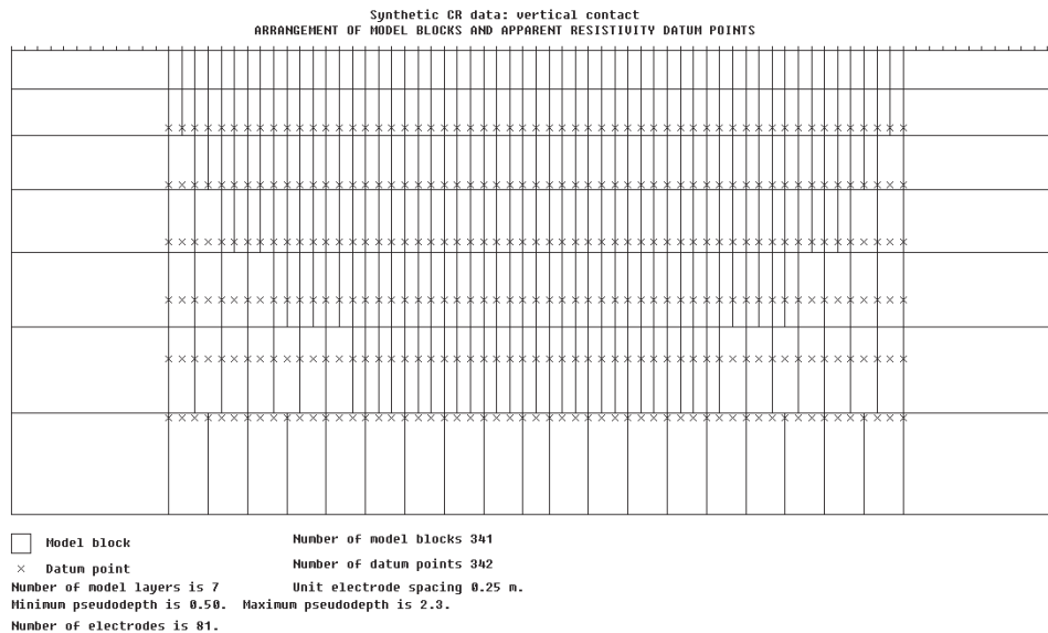
Figure 8.10: Example of model discretisation for the 2D inversion of towed-array CR data.
