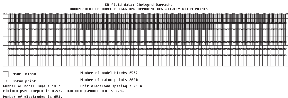
Figure 8.12: Example of model discretisation for the 2D inversion of CORIM™ field data, Chetwynd Barracks.
