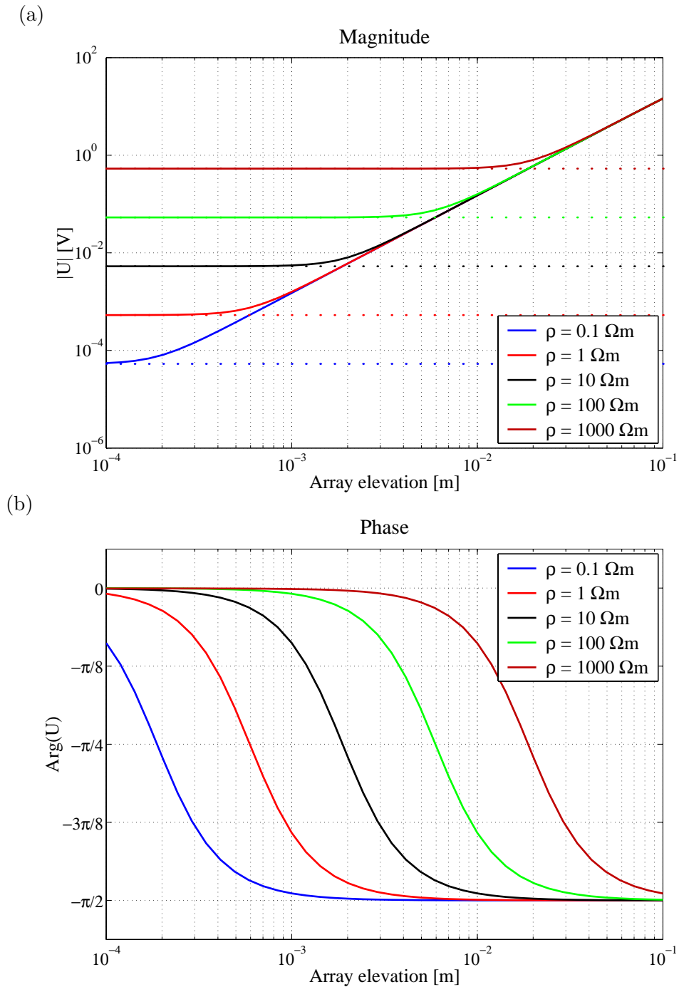
Figure 5.5: Variation of the complex potential with array elevation for a capacitive array in inline configuration. Parameter: resistivity. Dipole length l = 1\text{m} , dipole separation r = 2\text{m} , \varepsilon_r = 1 , f = 15\text{kHz} , I = 10\text{mA} . (a) magnitude, (b) phase. Values for an equivalent DC array are shown as dotted lines.
