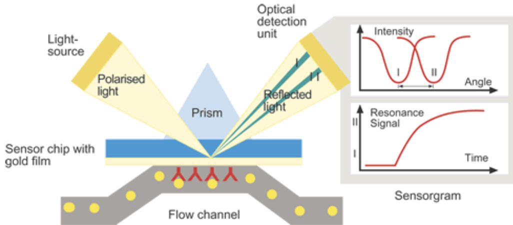
Figure 2.12 (from www.biocore.com , accessed June 2004). A schematic of the setup of a typical SPR instrument. The ligand, shown by a red inverted Y is attached to the thin gold layer of the sensor chip. Plane polarised light is directed at the gold film and due to SPR there is a decrease in reflected light intensity at angle 1. When the ligand is exposed to analyte molecules shown in yellow circles, the change in mass at the surface due to the interaction between the ligand and the analyte causes a local refractive index change at the sensor surface, causing a change in the angle reflected light with reduced intensity from angle 1 to angle 2.
