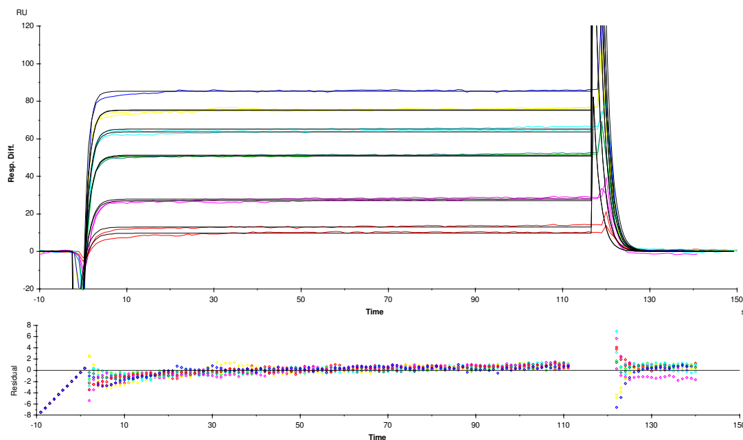
Figure 3.22 Corrected sensorgrams and residual plots for titration of 2 \mu\text{M} (red), 5 \mu\text{M} (magenta), 10 \mu\text{M} (green), 20 \mu\text{M} (cyan), 30 \mu\text{M} (yellow) and 40 \mu\text{M} (blue) N43A ColE9/Im9 against TolB at 25°C are shown. The fitted kinetic data for binding are superimposed onto each sensorgram in black. Residual plots highlight deviation of the experimental data from the theoretical fit.
