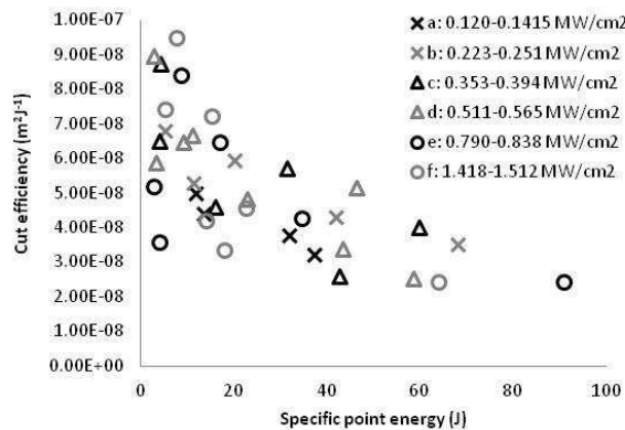
Figure 8 Variation of cutting efficiency with SPE for all thicknesses, markers indicate power density range of data.
