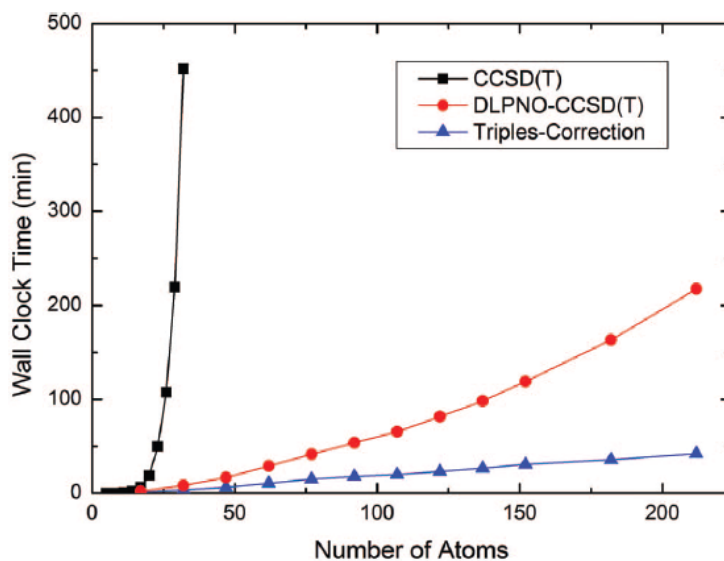
Figure 4. (a) Rotational barrier of ethane-1,2-diphenyl. The structures from a relaxed surface scan with the PBE functional and TZVP basis set with van der Waals corrections. All calculations were done with TZVP basis set. (b) Scaling behavior of the CCSD(T) and DLPNO-CCSD(T) method. The calculations were carried out on linear hydrocarbon chains \text{H}_3\text{C}-(\text{CH}_2)_{n-2}-\text{CH}_3 . All calculations were done with the SVP basis set. The time required for triples-correction is part of the entire DLPNO-CCSD(T) calculation time. Figure taken from Ref. 26. Reprinted with permission from [Riplinger, C.; Sandhoefer, B.; Hansen, A.; Neese, F. Natural Triple Excitations in Local Coupled Cluster Calculations with Pair Natural Orbitals. J. Chem. Phys. 139, 134101 (2013)]. Copyright [2013], AIP Publishing LLC.
