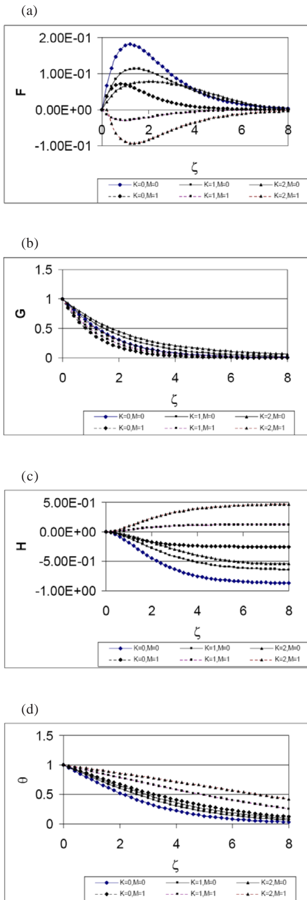
Fig. 3 Effect of the porosity parameter M and the non-Newtonian parameter K on the profile of: (a) radial velocity F ; (b) azimuthal velocity G ; (c) axial velocity H ; (d) temperature \theta ( S=0, P_r=0.7 )
