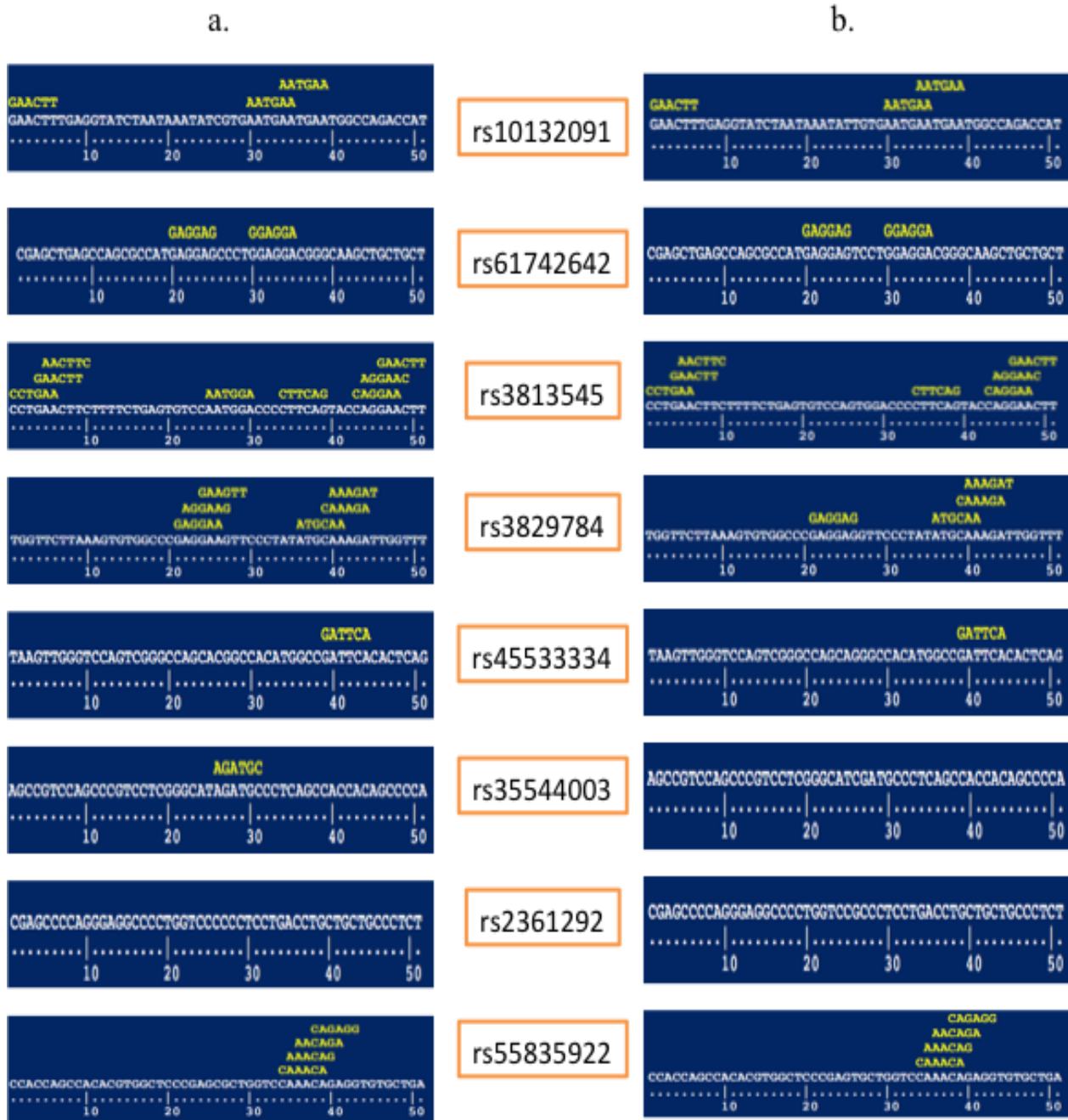
Figure 4. Output of RESCUE-ESE showing exonic splicing enhancer of SNPs. Column “a” includes the wildtype sequences for each of the SNPs. Column “b” includes sequences with the changed alleles, showing how the exonic splicing activity changes as well.
