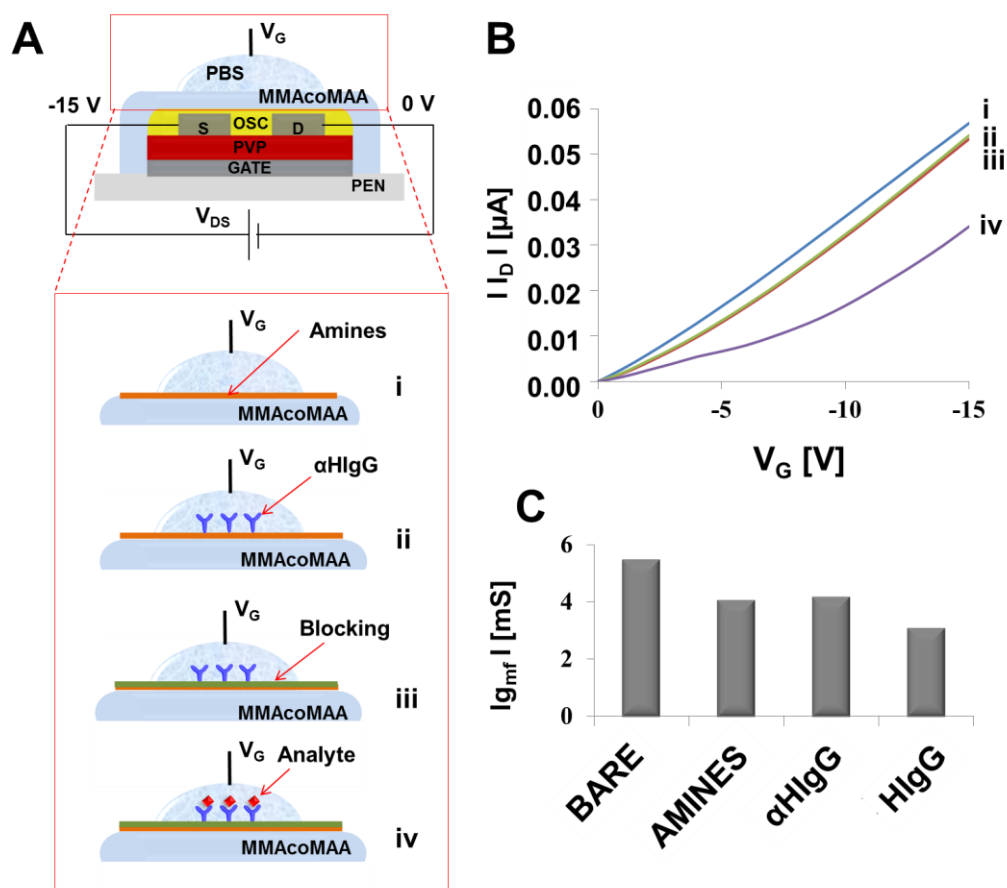
Figure 8. (A) Schematic of the stepwise functionalization of the insulator (MMAcoMAA) in the BioFET: (i) amino-functionalization (with 1% APTES); (ii) immobilization of capture antibodies; (iii) blocking to prevent non-specific absorption; and (iv) analyte conjugation. (B) Corresponding current normalized transfer-curve plots for the MMAcoMAA BioFET gate after each of the conjugation steps. (C) Transconductance (transistor gain) for each functionalization step.
