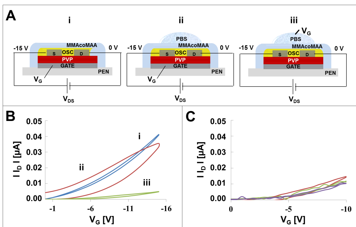
Figure 7. (A) Schematics for the OTFT in three configurations: bottom gate (i); with electrolyte (on the MMAcoMAA layer) (ii); and with electrolyte (on the MMAcoMAA layer) plus reference electrode (iii). (B) The corresponding I-V plots for all three configurations. (C) Repeatability plot for the third configuration (electrolyte plus reference electrode).
