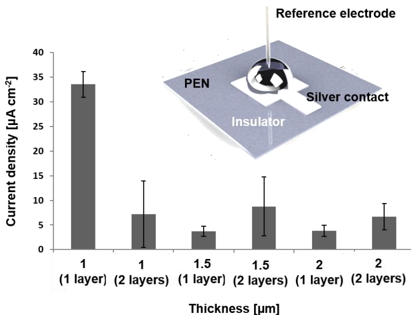
Figure 2. Electrical characterization of MMAcoMAA insulator layers according to the number and thickness of each: current density measurements at -30 V.
