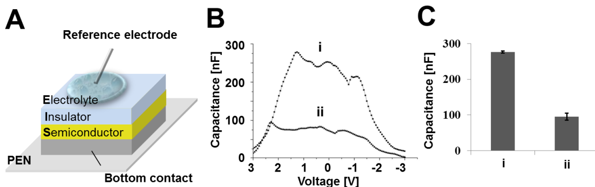
Figure 6. (A) Schematic of the EIS (from bottom to top): conductor (Ag nanoparticle ink); semiconductor (FS-0027); insulator (MMAcoMAA); electrolyte (PBS, 2 \mu L); and reference electrode. (B) Capacitance-voltage measurements with electrolyte (PBS) on the EIS in two structures: with amino-functionalized (1% APTES) insulator (i) or BSA-functionalized (1 \mu g mL -1 ) insulator (ii). (C) Capacitance measurements for two different EIS structures: with amino-functionalized (i) or BSA-functionalized (ii) insulator.
