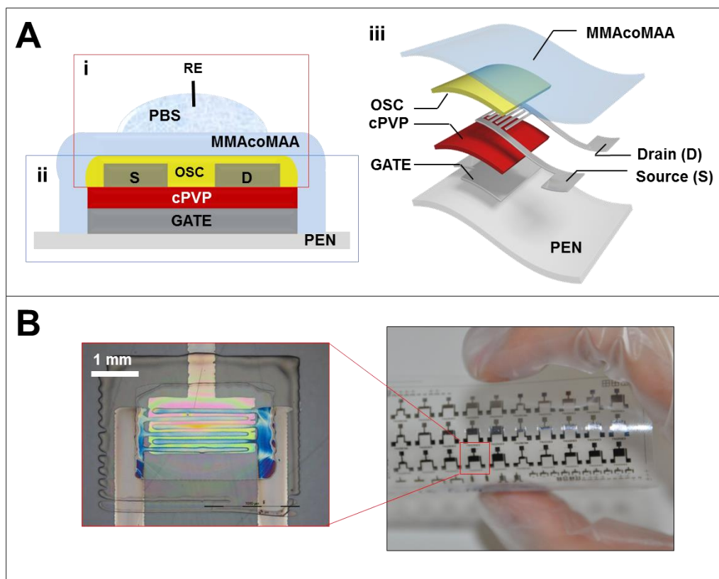
Figure 1. (A) Structure of the BioFET: (i) the top OFET; (ii) the bottom OFET and (iii) each layer of the BioFET. The OFET channel dimensions ( W : channel width; L : channel length; in \mu\text{m} ) were: W \times L = 20,000 \times 40 or 40,000 \times 40 . OSC: organic semiconductor; MMAcoMAA: methyl methacrylate copolymer; PEN: polyethylene-naphthalate; cPVP: cross-linked poly-4-vinylphenol; and RE: reference electrode. (B) Photographs of the printed OFETs.
