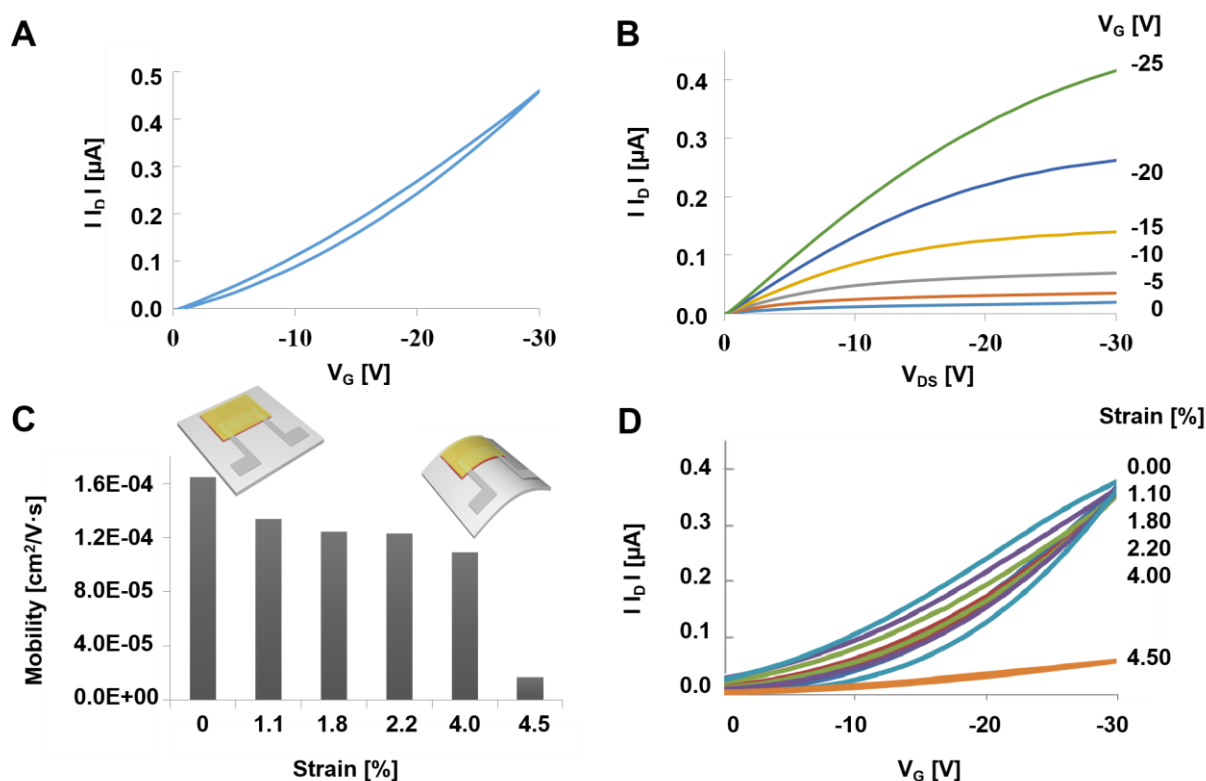
Figure 4. Transfer curves for the FS0027 semiconductor layer at room temperature: (A) OFET transfer curve in saturation mode ( V_{DS} = -30V ), (B) OFET output plot for a W/L ratio of 250, (C) Mobility of the OFET in function of bending radii, and (D) Transfer curve characteristics at different strains.
