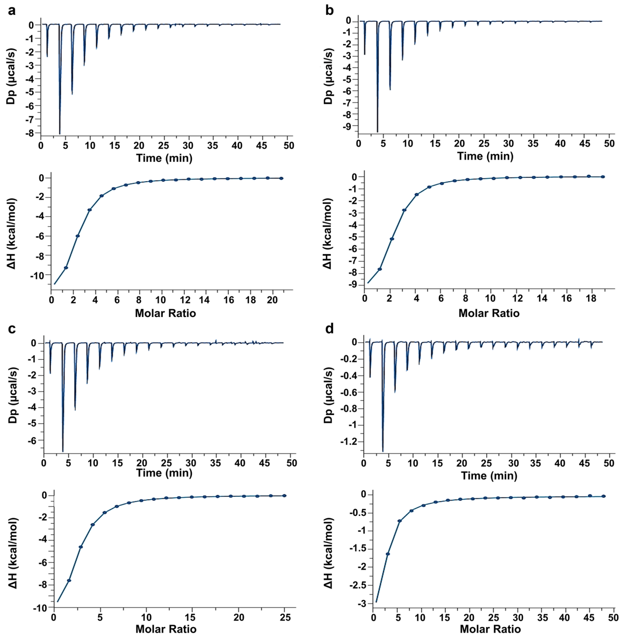
Fig. 3 ITC titration profile of LacNAc (6.0 mM) binding to a Gal-3-Gal-3 (55 \mu\text{M} ), b Gal-3-8S-Gal-3 (61 \mu\text{M} ), c Gal-3-Gal-1 (46 \mu\text{M} ), and d Gal-3-8S-Gal-1 (24 \mu\text{M} ) in phosphate-buffered saline (pH 7.2) containing 20 mM phosphate, 10 mM NaCl and 2 mM \beta -mercaptoethanol. Lectins are prepared by lyophilization ( b , d ) or precipitation by ammonium sulfate ( a , c ). Injections of ligand
