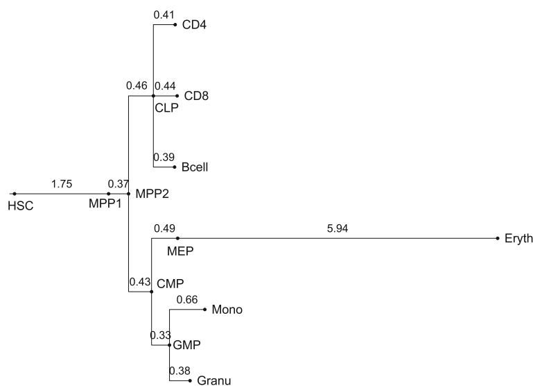
Fig. 4 Estimates without IWEs. Tree resulting from estimates without modeling IWEs. The logarithmic branch lengths are the means of the MCMC samples after a burn in phase of 10^6 steps
