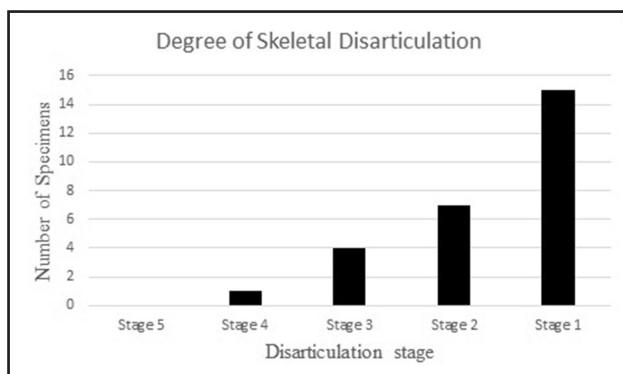
Figure 3: Results of disarticulation of fishes. Data shows that articulated skeletons are much rarer than disarticulated ones.
