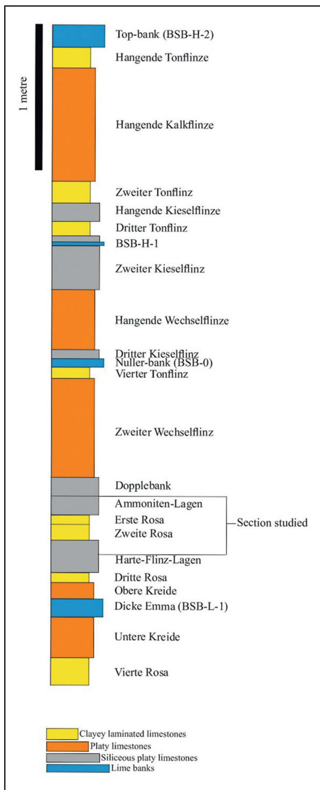
Figure 1: The Mörnsheim Formation at the quarry, showing the extent of the studied section.
