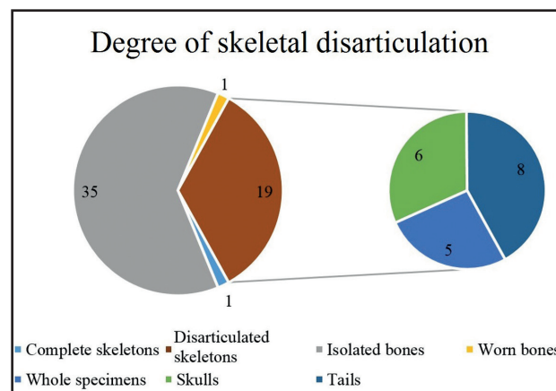
Figure 2: Results of disarticulation of fishes. Data clearly shows that complete specimens are much rarer than disarticulated ones. Demonstrating that carcasses were exposed at the surface long enough for soft tissues to disaggregate and taphonomic processes to manipulate skeletal elements.
