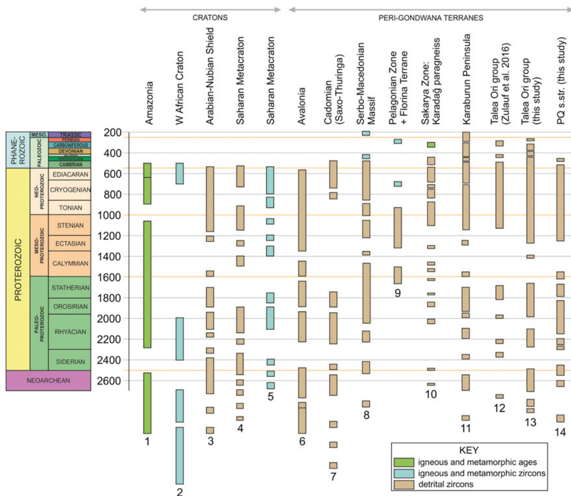
Fig. 13. (Colour online) Distribution of detrital/igneous/metamorphic zircon ages and igneous/metamorphic events known from major cratons and peri-Gondwana terranes, modified after Ustaömer et al. (2013), in comparison to data from the Talea Ori (12–14). Data sources: 1, Friedl et al. (2004), Nance et al. (2008); 2, Friedl et al. (2004), Linnemann et al. (2004), Murphy et al. (2004 a,b); 3, Drost et al. (2011) and references therein; 4, Drost et al. (2011) and references therein, Meinhold et al. (2011); 5–7, Drost et al. (2011) and references therein; 8, Himmerkus et al. (2007, 2009), Meinhold et al. (2010), Pirgadiikia and Vertiskos Terranes belonging to the Serbo-Macedonian Massif; 9, Himmerkus et al. (2007) and references therein; 10, Ustaömer et al. (2013); 11, Löwen et al. (2017); 12, Zulauf et al. (2016); 13–14, this study.
