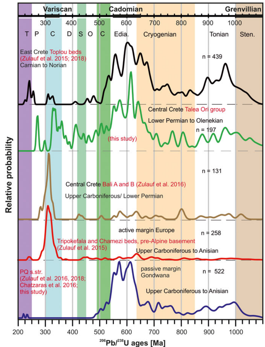
Fig. 14. (Colour online) Comparison of probability curves from different units exposed on Crete.
