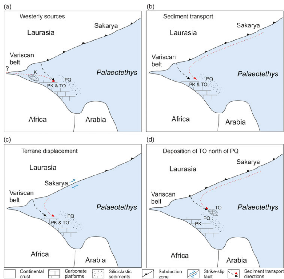
Fig. 15. (Colour online) Alternatives for the palaeogeographic configurations of the lower tectonic nappes of the Cretan nappe pile from Late Carboniferous / Early Permian to Olenekian times. Dashed arrows indicate directions of sediment transport (black dashed arrows = transport of euhedral Variscan-aged zircons; red dotted arrows = transport of rounded zircons with Silurian, Devonian and Early Carboniferous U–Pb ages). (a) Distal sediment transport from westerly yet unspecified sources, modified after Ustaömer et al. (2019). (b) Distal sediment transport from the Sakarya Zone. (c) Eastward terrane displacement of the Sakarya Zone after deposition of the lower Talea Ori group. Blue/grey arrows indicate dextral displacement that should have happened after Olenekian times. (d) Deposition of the Talea Ori group north of the PQ s.str. Abbreviations are: Sakarya Zone (Sk), Phyllite–Quartzite unit s.str. (PQ), Plattenkalk unit (PK), Talea Ori (TO), Karaburun sediments (K).
