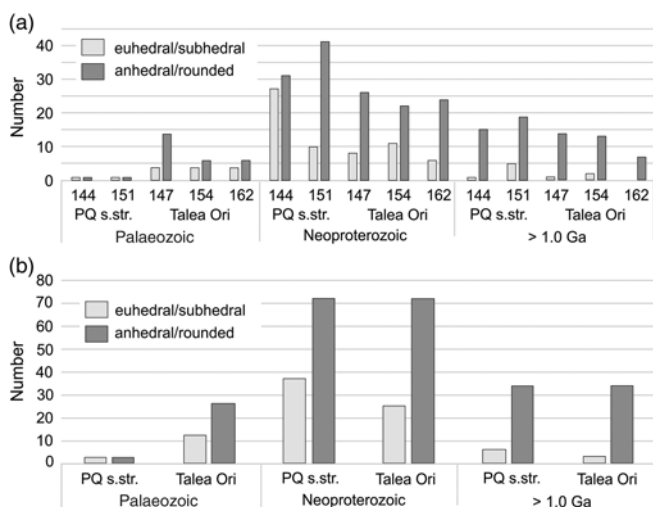
Fig. 6. Number of euhedral and subhedral vs anhedral and rounded zircons within (a) each of the five different samples LS 144, LS 151, LS 162, LS 147, LS 154 and (b) the PQ s.str. (LS144 + LS151) and the Talea Ori group (LS162, LS147, LS154).
