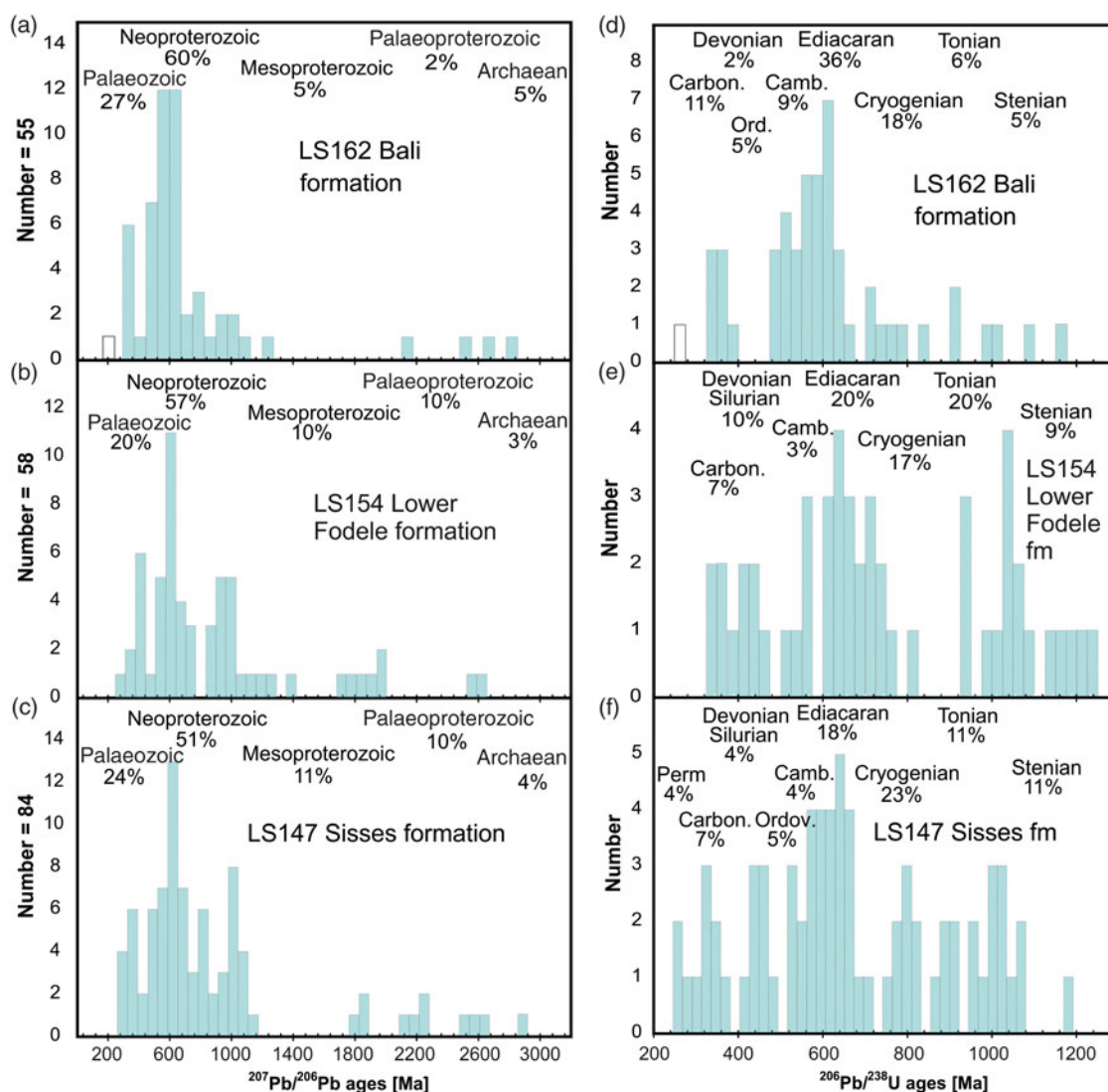
Fig. 7. (Colour online) Density plots of detrital zircons separated from the Bali formation (LS162), lower Fodele formation (LS154) and Sisses formation (LS147) of the Talea Ori group. Complete ranges are plotted against the ^{207}\text{Pb}/^{206}\text{Pb} age, and for younger zircons the ^{206}\text{Pb}/^{238}\text{U} age is shown. Bin width = 40, concordance 90% to 110%.
