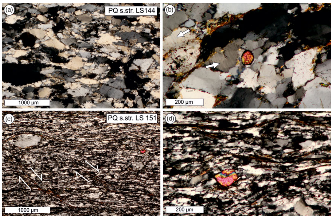
Fig. 10. (Colour online) Photomicrographs of samples from the PQ s.str. collected for U–Pb dating of detrital zircons (crossed polarizers). (a, b) Quartzite LS144 (Skilarmi) shows irregular-shaped elongate quartz grains with sutured grain boundaries. Close-up (b) shows deformation lamellae in quartz grain, left to euhedral zircon. (c, d) Albite-gneiss NW of Fodele shows layers with fine-grained quartz and larger albite clasts as well as subhedral to euhedral zircon grains (d).
