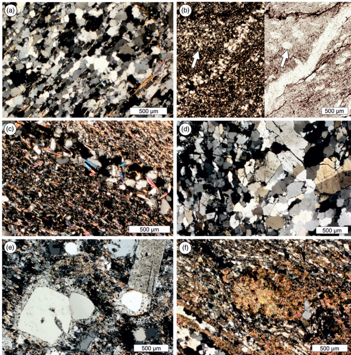
Fig. 3. (Colour online) Photomicrographs of the components of the Bali quartz metaconglomerate and metasandstones. (a) Quartzite with mica flakes (crossed polarizers CT785). (b) Metachert with coarser quartz veins and ellipsoidal components visible mainly with plane polarized light (white arrows) (CT785i, left: crossed polarizers, right: plane polarizers). (c) Metapelite with psammitic layer (LS70 crossed polarizers). (d) Albite–quartz aggregates; here also the finer-grained matrix largely consists of small isometric grains of albite (LS261G crossed polarizers). (e) Felsic volcanic rock (LS261A crossed polarizers): euhedral quartz with resorption embayments and plagioclase with sericitization in fine-grained quartz–plagioclase–sericite matrix; quartz shows overgrowth rims. (f) Retrograde mica schist with aggregate of fine-grained phyllosilicates (LS261F crossed polarizers).
