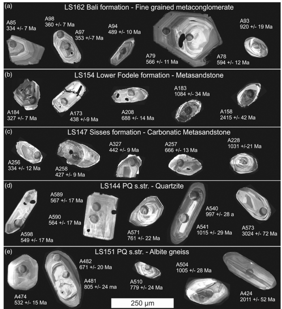
Fig. 5. Representative cathodoluminescence (CL) images of analysed zircons. Apparent ^{206}\text{Pb}/^{238}\text{U} ages are reported with 2\sigma uncertainty.
