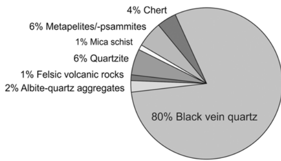
Fig. 4. Abundance of different pebbles of the Bali quartz metaconglomerate.
