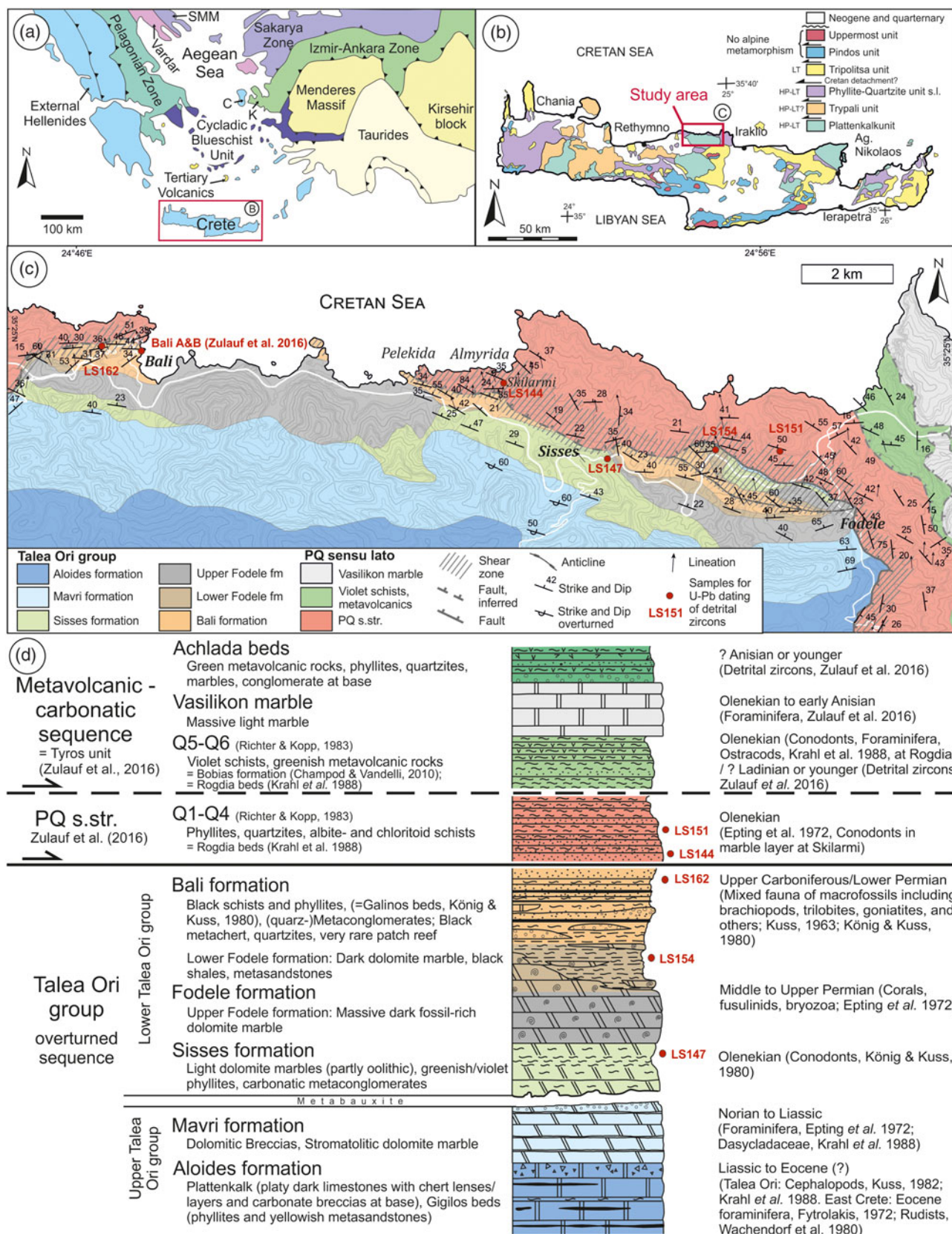
Fig. 1. (Colour online) Geologic map of (a) the Eastern Mediterranean, modified after Zulauf et al. (2007), abbreviations: C = Chios, K = Karaburun; (b) the island of Crete, modified after Creutzburg & Seidel (1975); and (c) the Talea Ori, central Crete, modified after Epting et al. (1972). The structural data and location of the shear zone are based on Seybold et al. (2019). (d) Stratigraphic column of the different tectonostratigraphic units cropping out in the Talea Ori, modified after Epting et al. (1972). The given ages are biostratigraphic ages based on the macro- and microfossil records of the rocks.
