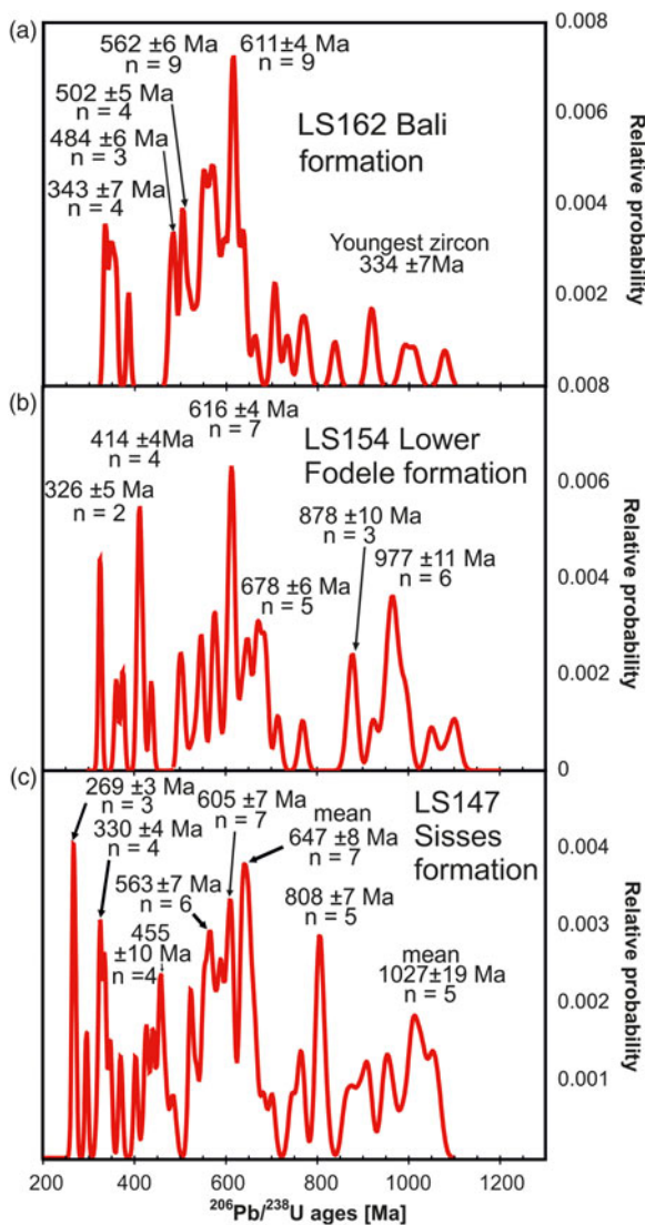
Fig. 8. (Colour online) Probability curves with age peaks of Bali formation, lower Fodele formation and Sisses formation of the Talea Ori group.
