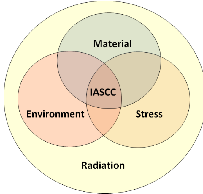
Figure 1. Venn diagram of IASCC pre-requisite conditions. Note that the radiation environment tends to enhance the three conditions related to material, environment and stress state.
