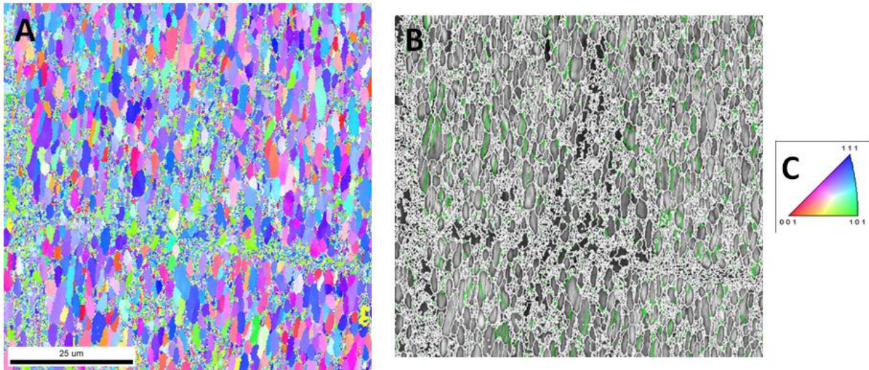
Figure 23 – (a) EBSD-OIM representation and (b) strong link map of the 316L chip deformed at a tool velocity of 25 cm/s follow a heat treatment of 800°C for 5 minutes; (c) OIM legend
