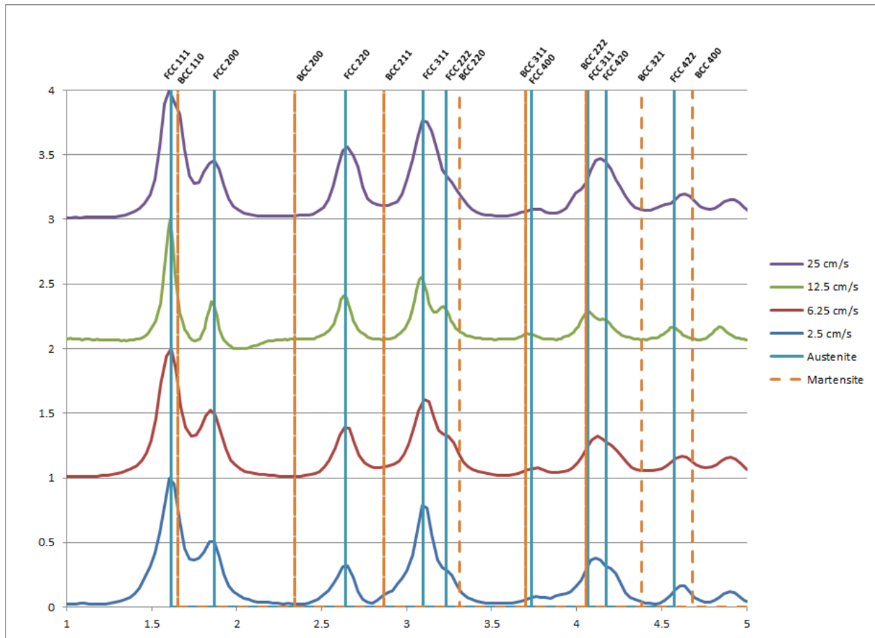
Figure 7 – PASAD data plot for the 4 different tool velocities of the 316L chips
