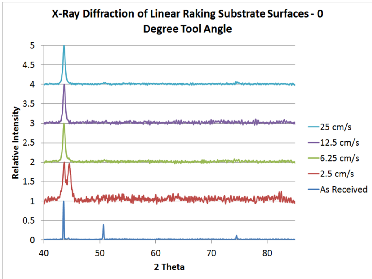
Figure 11 – XRD line scan for the four different tool velocities of the surface substrate
