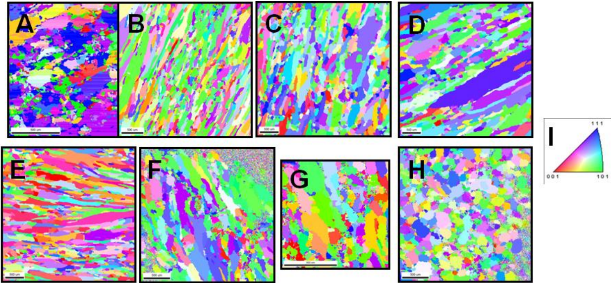
Figure 18 – PED-OIM representations of the 316L chips deformed at a tool velocity of 12.5 cm/s follow heat treatments (a) none, (b) 350°C, (c) 400°C, (d) 450°C, (e) 500°C, (f) 550°C, (g) 600°C, and (h) 650°C for one hour; (i) OIM legend
