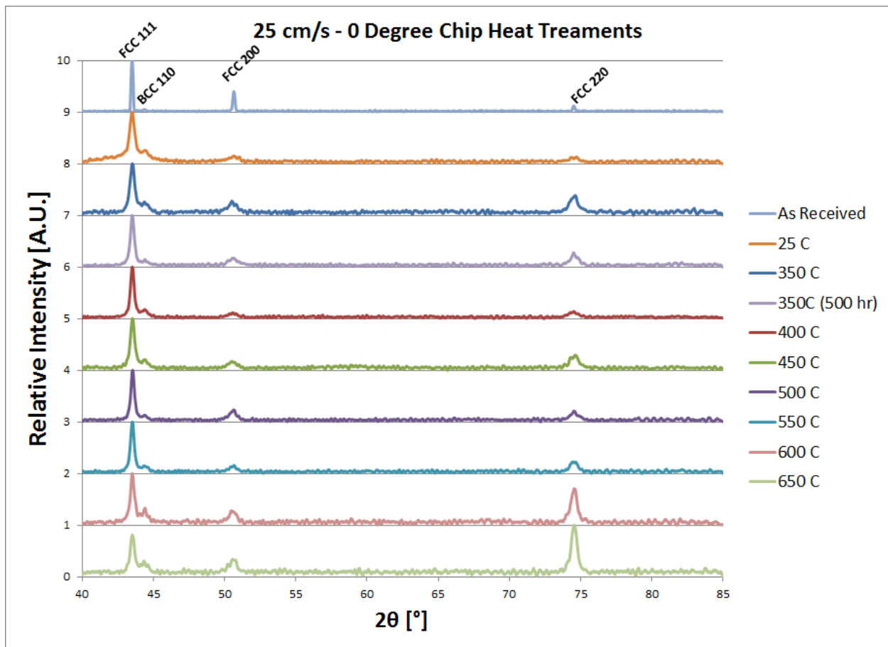
Figure 21 - XRD line scans of the 316L chips deformed at a tool velocity of 25 cm/s follow heat treatments from 350°C to 650°C at 50°C intervals for one hour and 350°C for 500 hours
