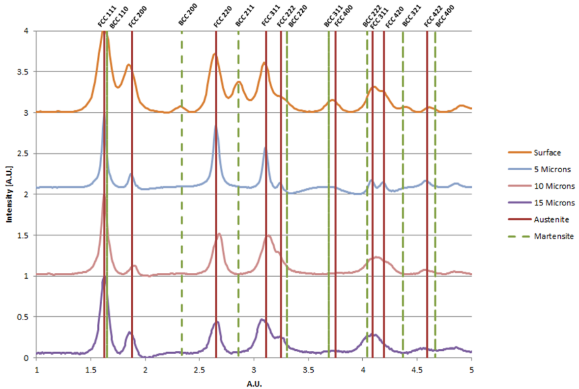
Figure 15 - PASAD data plot for the surface substrate deformed at 12.5 cm/s at the surface, 5 \mu\text{m} , 10 \mu\text{m} , and 15 \mu\text{m} in depth
