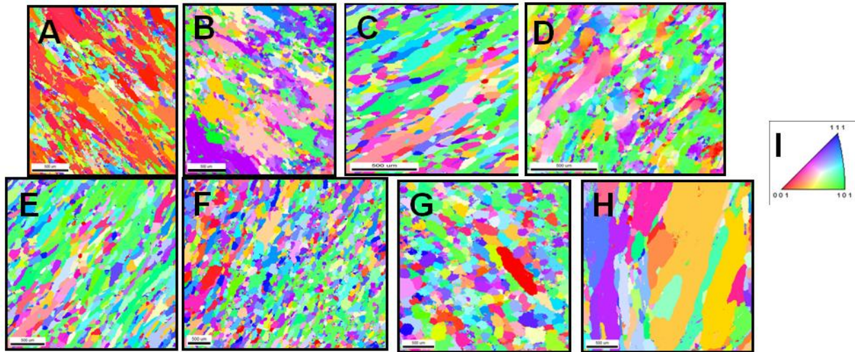
Figure 19 - PED-OIM representations of the 316L chips deformed at a tool velocity of 25 cm/s follow heat treatments (a) none, (b) 350°C, (c) 400°C, (d) 450°C, (e) 500°C, (f) 550°C, (g) 600°C, and (h) 650°C for one hour; (i) OIM legend
