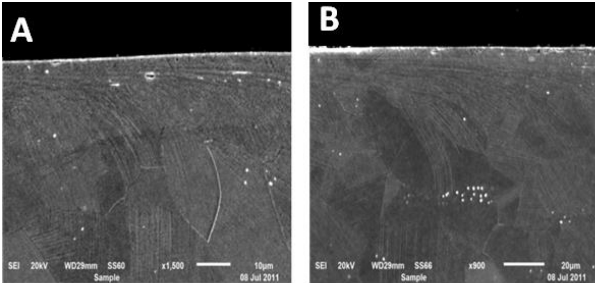
Figure 12 – Cross-sectional SEM micrographs in SE mode imaging at (a) high and (b) low magnification. The machining tool traversed from right to left.
