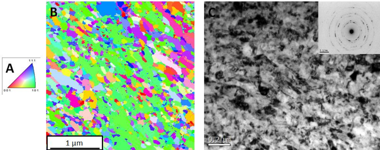
Figure 22 – (b) PED-OIM representation and (c) BF micrograph along with associated SADP of the 316L chip deformed at a tool velocity of 25 cm/s follow a heat treatment of 350°C for 500 hours; (a) OIM legend
