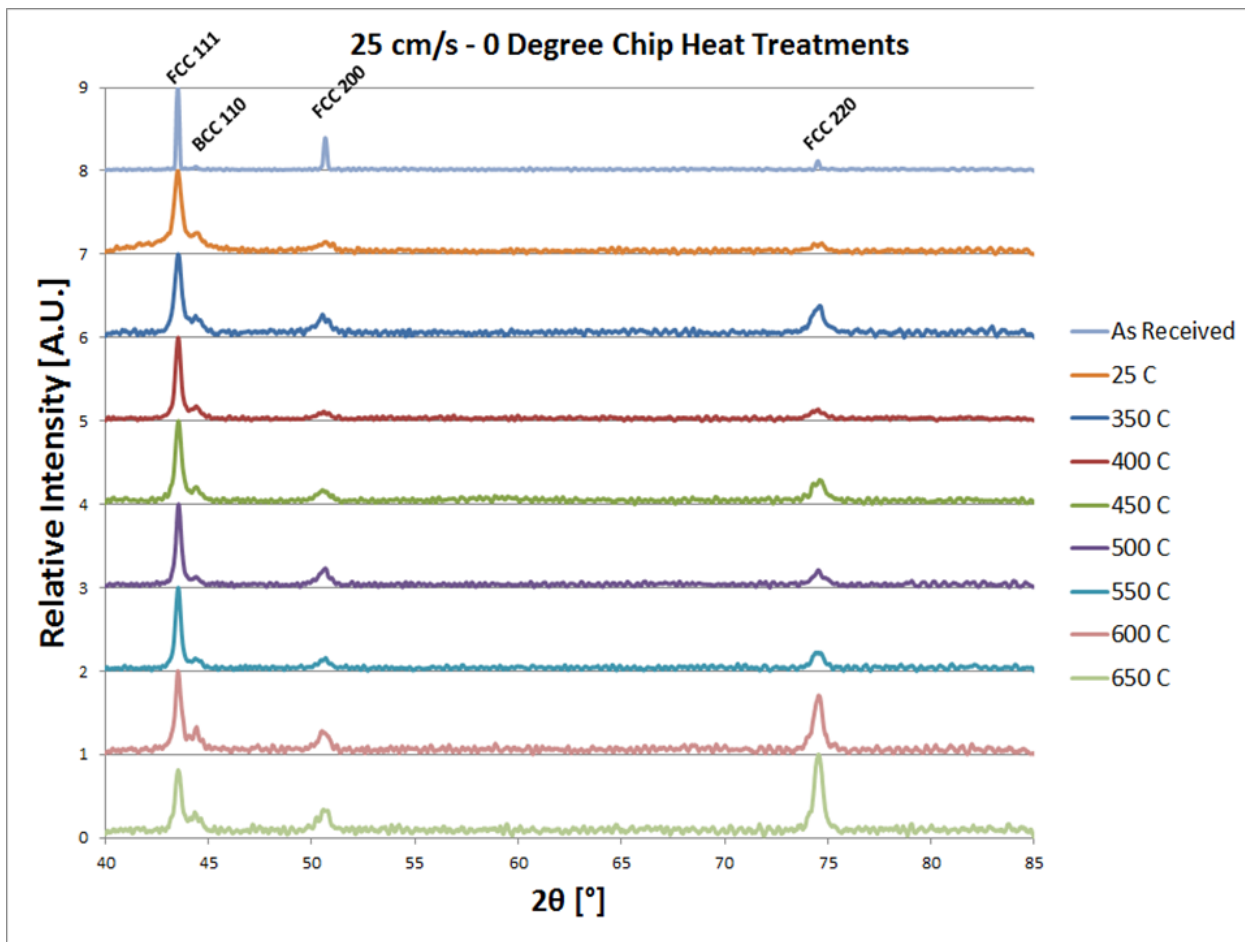
Figure 17 - XRD line scans of the 316L chips deformed at a tool velocity of 25 cm/s follow heat treatments from 350°C to 650°C at 50°C intervals for one hour
