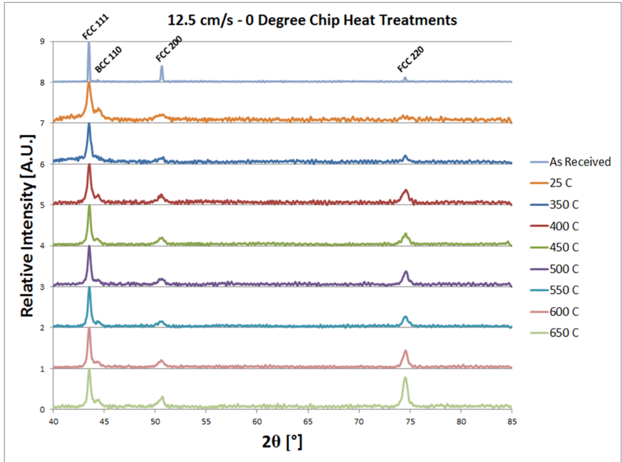
Figure 16 – XRD line scans of the 316L chips deformed at a tool velocity of 12.5 cm/s follow heat treatments from 350°C to 650°C at 50°C intervals for one hour
