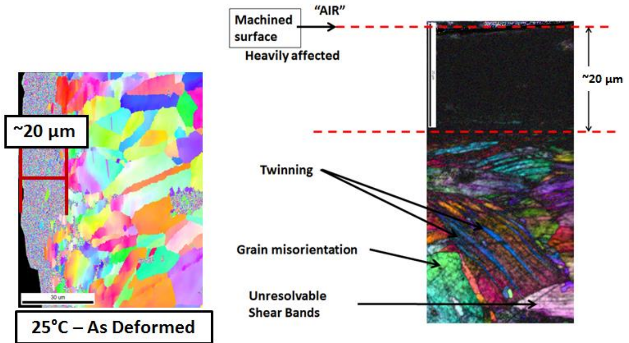
Figure 13 – Cross-sectional surface substrate following deformation with a tool velocity of 12.5 cm/s with the (a) inverted pole figure and (b) inverted pole figure map overlaid with the image quality map
