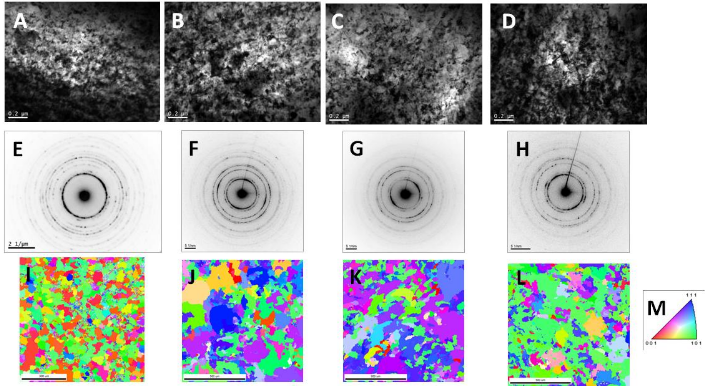
Figure 14 – TEM BF and associated SADP and PED-OIM representation for the surface substrate deformed with a tool velocity of 12.5 cm/s at (a, e, i) the surface, (b, f, j) 5 \mu\text{m} , (c, g, k) 10 \mu\text{m} , and (d, h, l) 15 \mu\text{m} ; (m) OIM legend
