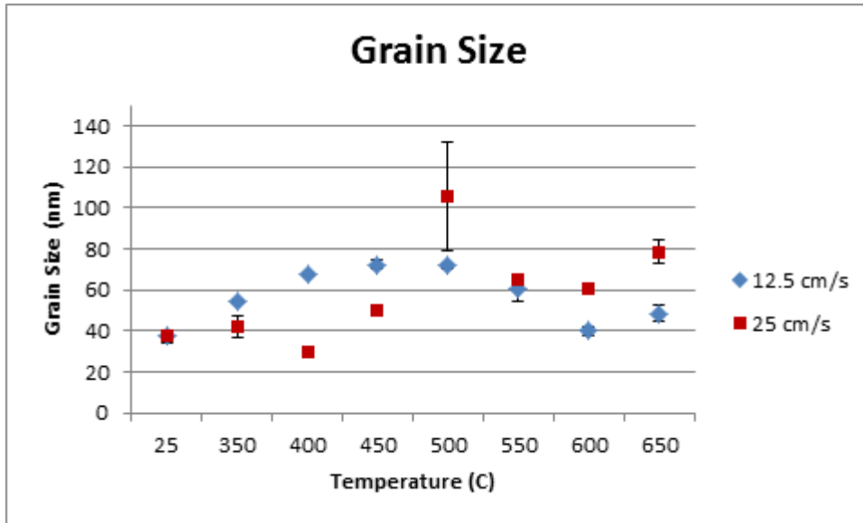
Figure 20 – Grain size measurements as determined by PED-OIM of the 316L chips deformed at a tool velocity of 12.5 cm/s and 25 cm/s follow heat treatments from 350°C to 650°C at 50°C intervals for one hour
