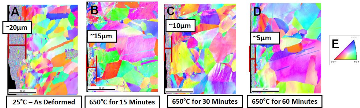
Figure 24 – Cross-sectional inverted pole figure representations of the 316L surface substrate deformed at tool velocity of 12.5 cm/s following heat treatment 650°C for (a) 0 minutes, (b) 15 minutes, (c) 30 minutes, and (d) 60 minutes; (e) OIM legend
