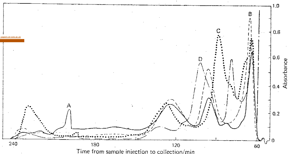
Fig. 1. Separation of four polyene antibiotics using the coil planet centrifuge. Coil volume, 110 ml; sample load, 600 \mu\text{g} ; solvent system, chloroform-methanol-borate buffer (4+4+3). Material completely soluble in mobile phase ( P=1.0 ) would be eluted at 60 min. A, Candicidin; B, levorin; C, trichomyacin; and D, hamycin.
