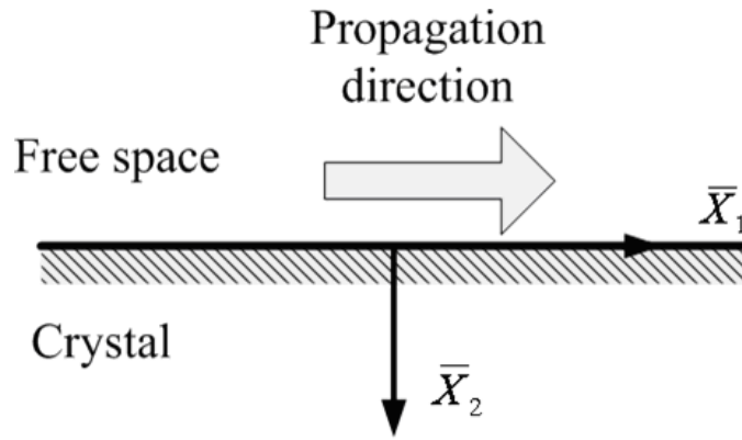
Figure 3. 4 SAWs propagating along top surface of an elastic half space
