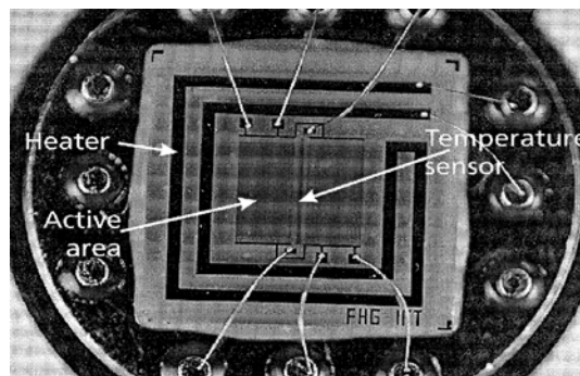
Figure 2. 5 [15] Structure of capacitor type CO 2 sensor.
