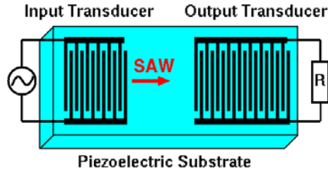
Figure 2. 6 [20] Structure of SAW sensor.
