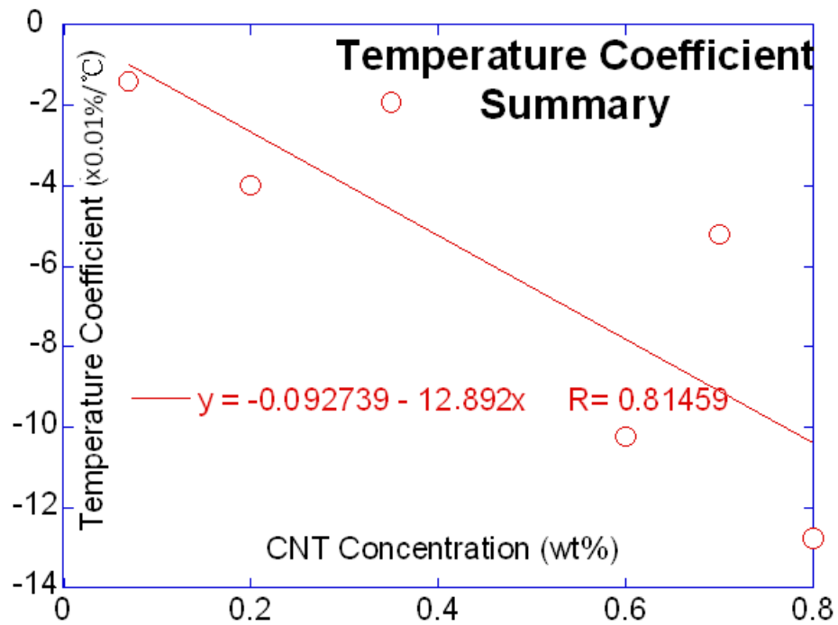
Figure 4. 21 Temperature Coefficient for nanocomposites with different CNT concentration.
