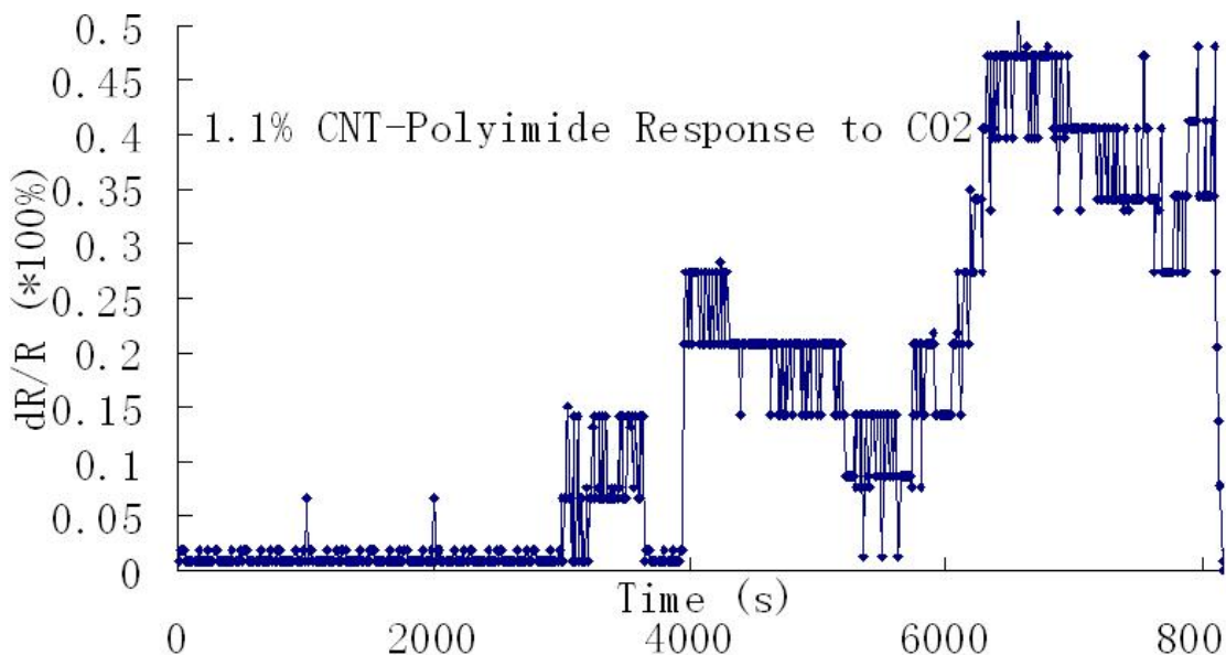
Figure 5. 14 Relative resistivity change of CNT-PI nanocomposite thin films with 1.1% CNT.
