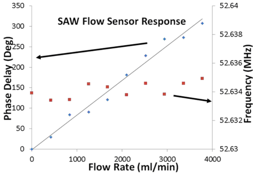
Figure 3.12 SAW flow sensor response
