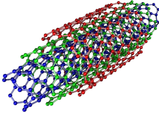
Figure 2. 8 [21] Typical three layer mwCNT with armchair structure.
