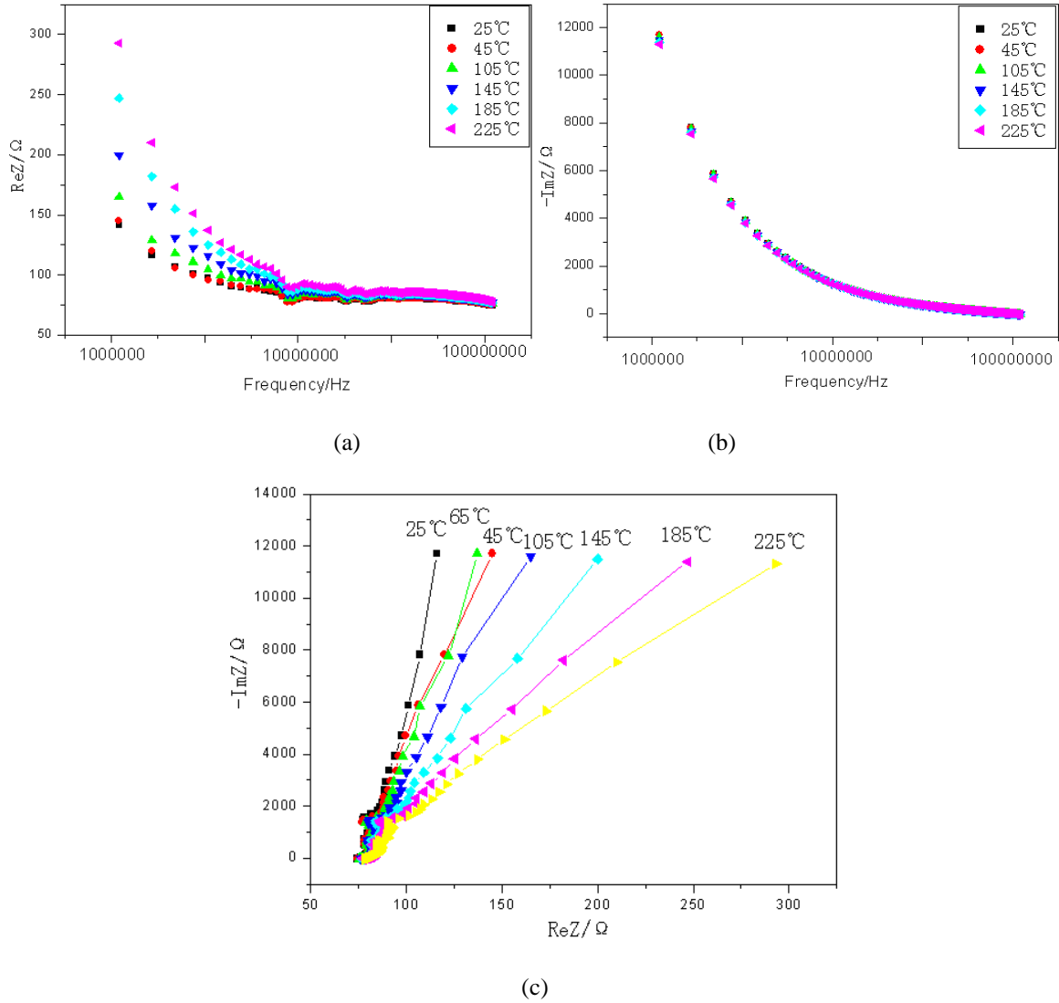
Figure 4. 6 Impedance of swCNT-polyimide composites(0%swcnt) at different temperature.
