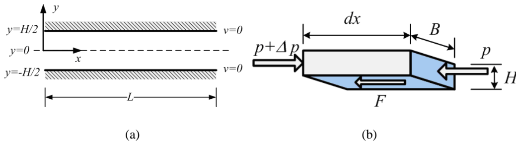
Figure 3. 2 (a) Two plate Couette problem. (b) Short Segment of flow chamber under pressure and dragging force.
