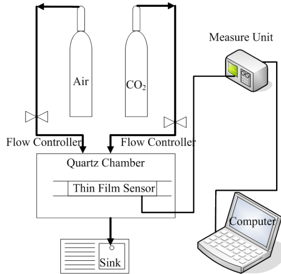
Figure 5. 1 Gas testing system schematic view.
