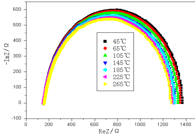
Figure 4. 11 Impedance of swcnt-polyimide composites(0.2%swcnt) at different temperature.
