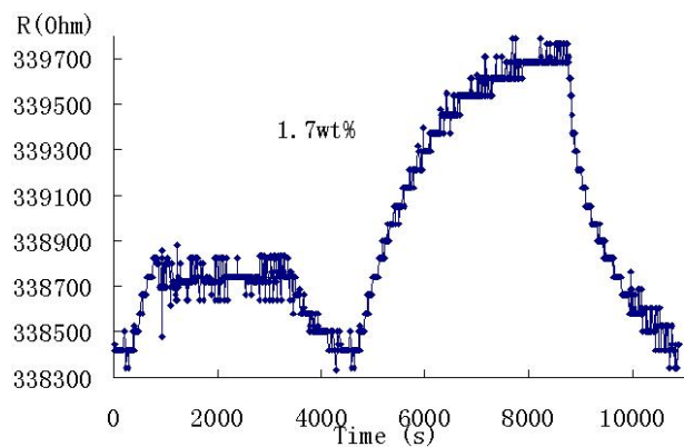
Figure 5. 11 Real time CO 2 response for nanocomposite thin film with 1.7wt% CNT concentration.
