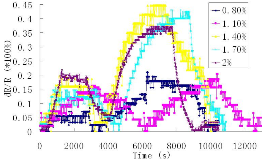
Figure 5. 13 Relative resistivity change of nanocomposite thin films.
