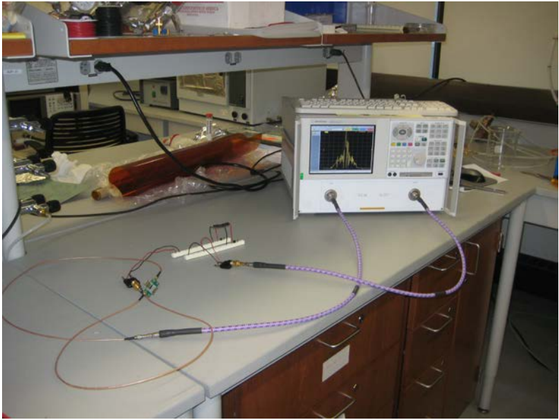
Figure 6. 5 Sample sensor connected with wireless module under measurement.
