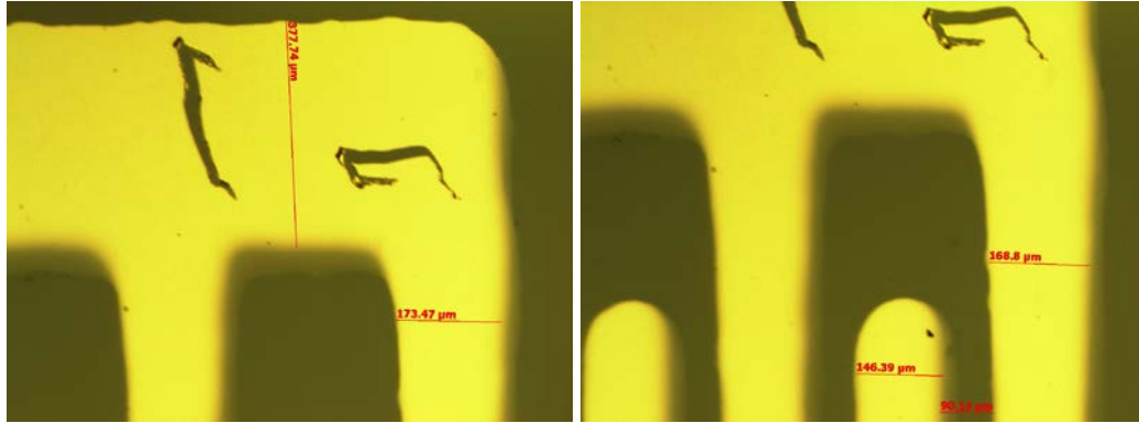
Figure 5. 23 IDT after shadow mask process.
