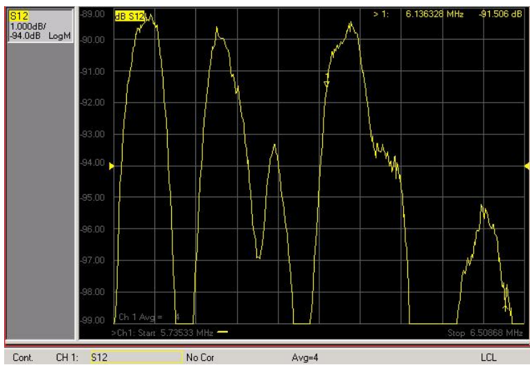
Figure 6. 20 Sensor response with antenna in parallel configuration at 40mm distance.
