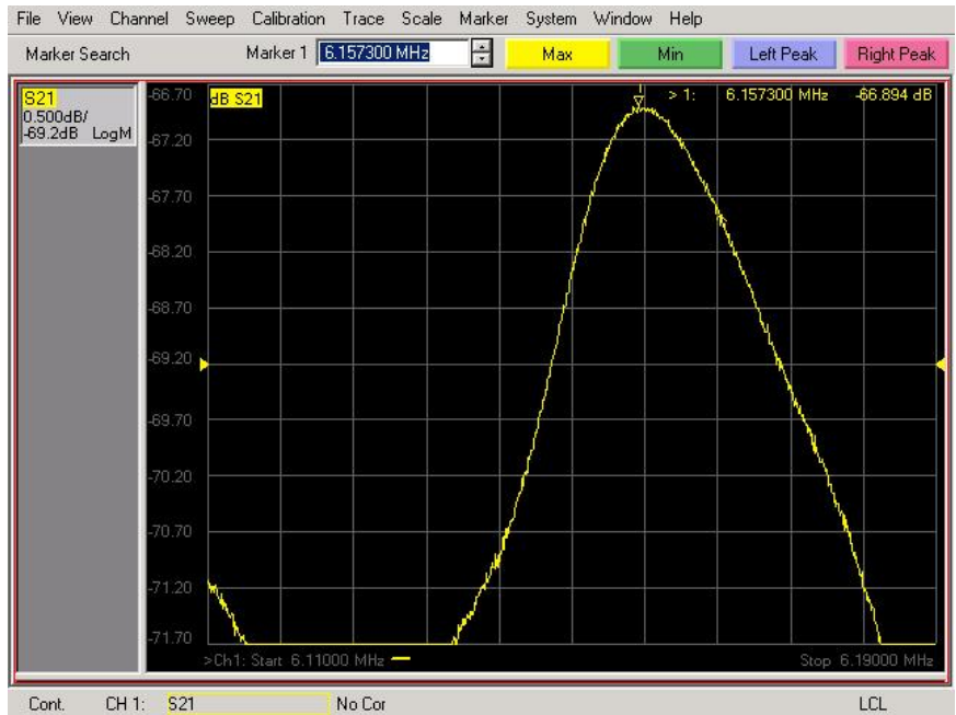
Figure 5. 29 Sensor Response 11.3%RH.
