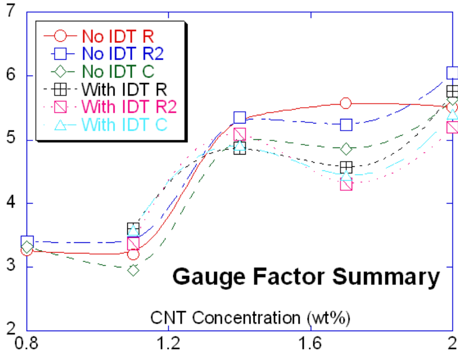
Figure 4. 40 Gauge Factor summary.
