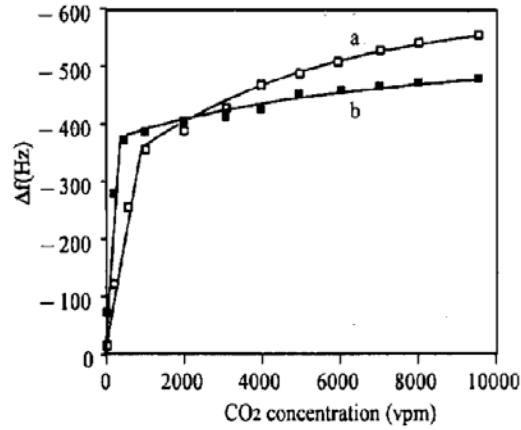
Figure 2. 4 [14] Response of Micro balance type CO 2 sensor with (a) 65nm (b) 62nm PAPO coating.
