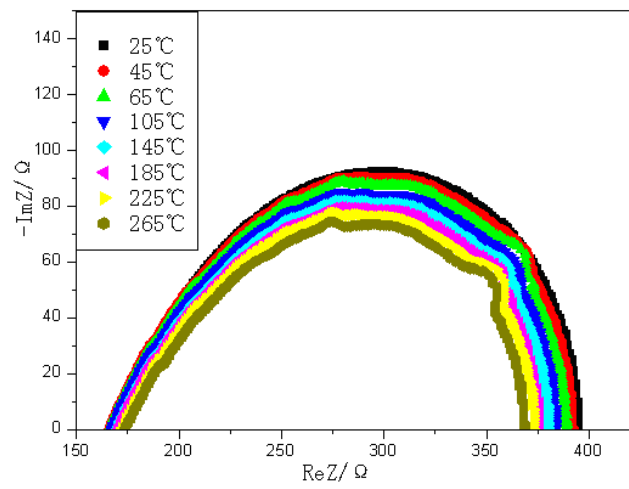
Figure 4. 14 Impedance of swcnt-polyimide composites(0.7%swcnt) at different temperature.
