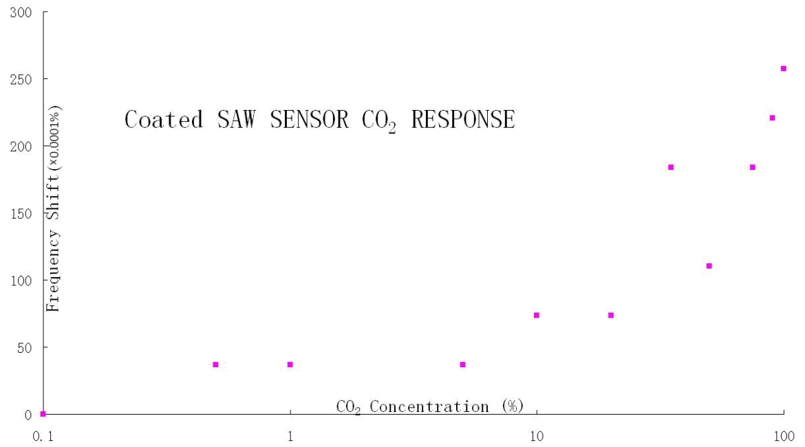
Figure 5. 38 Coated SAW Sensor gas response in log scale.
