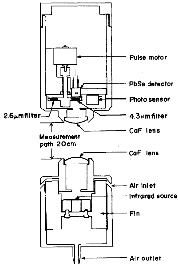
Figure 2. 3 [12] Typical NDIR CO 2 sensor structure.
