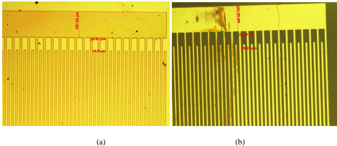
Figure 5. 22 (a) LiNbO 3 substrate right after patterning. (b) LiNbO 3 substrate after gold etching and RIE cleaning.
