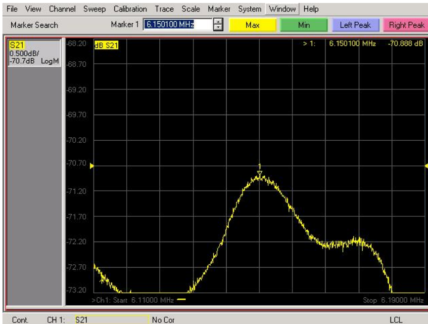
Figure 5. 34 Sensor Response 84.3%RH.
