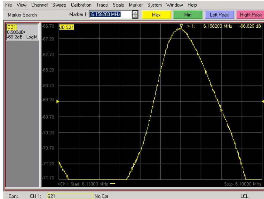
Figure 5. 28 Sensor Response at dry air with 0%RH.
