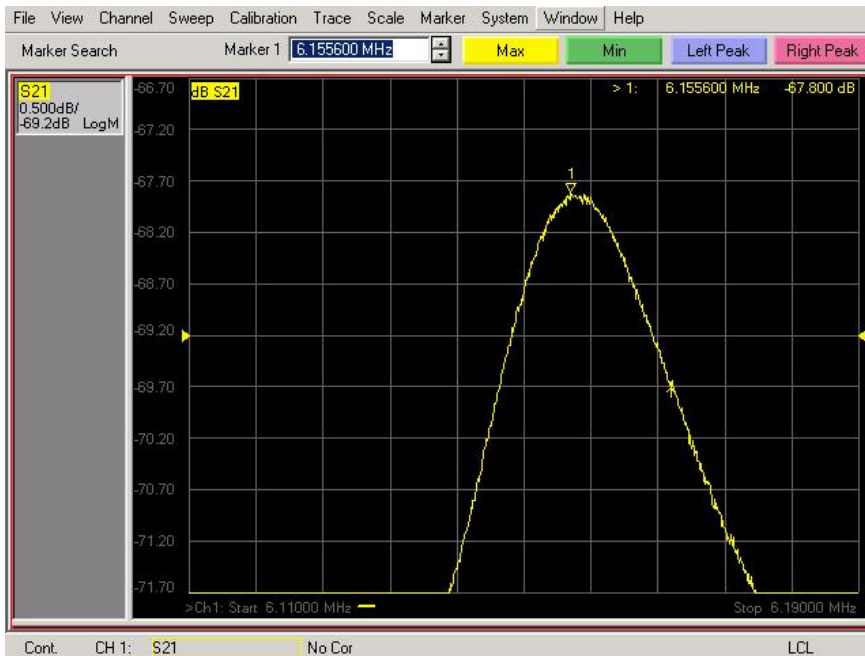
Figure 5. 32 Sensor Response 57.6%RH.
