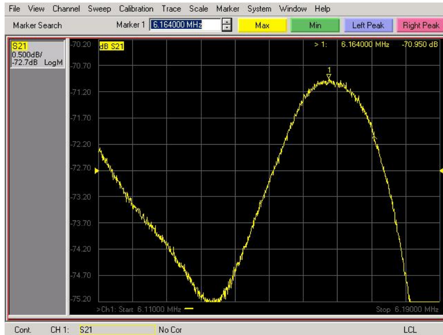
Figure 5. 35 Sensor Response 97.3%RH.
