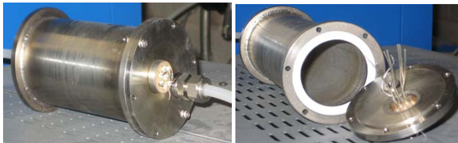
Figure 5. 5 Supplemental testing chamber for faster response.
