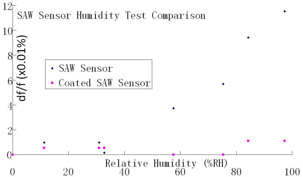
Figure 5. 36 SAW Sensor Humidity Response comparison after Parylene Coating.
