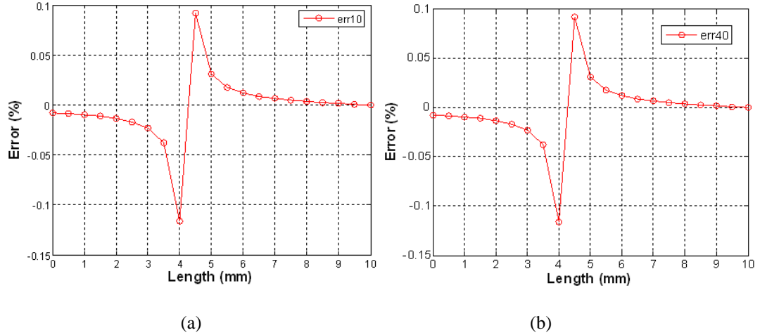
Figure 3. 5 Theoretical relative error of neglecting the shear stress (a) Error at 10kPa. (b) Error at 40kPa.
