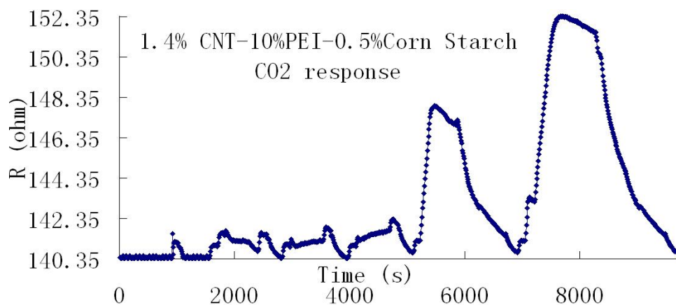
Figure 5. 15 Relative resistivity change of CNT-PEI nanocomposite thin films with 1.4% CNT and 0.5% corn starch.
