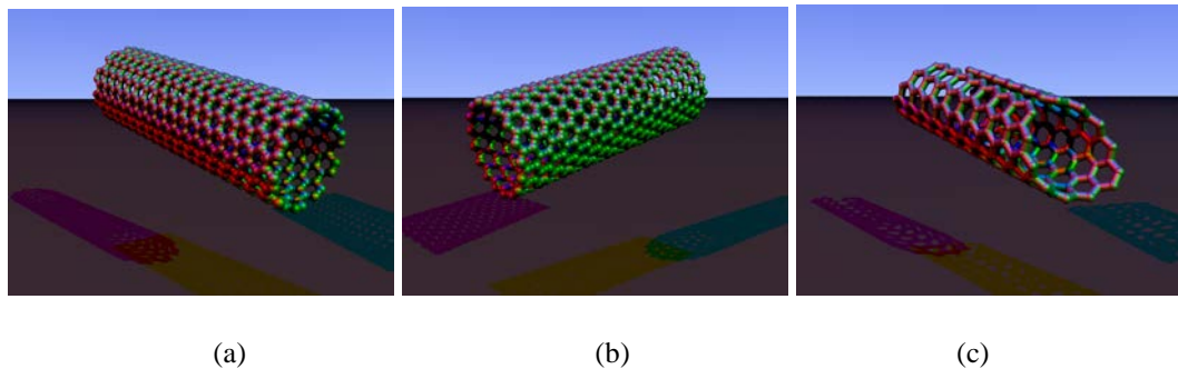
Figure 2. 7 [21] Typical swCNT structure. (a) Armchair (n, n) . (b) Zigzag (n, 0) . (c) Chiral (n, m) .
