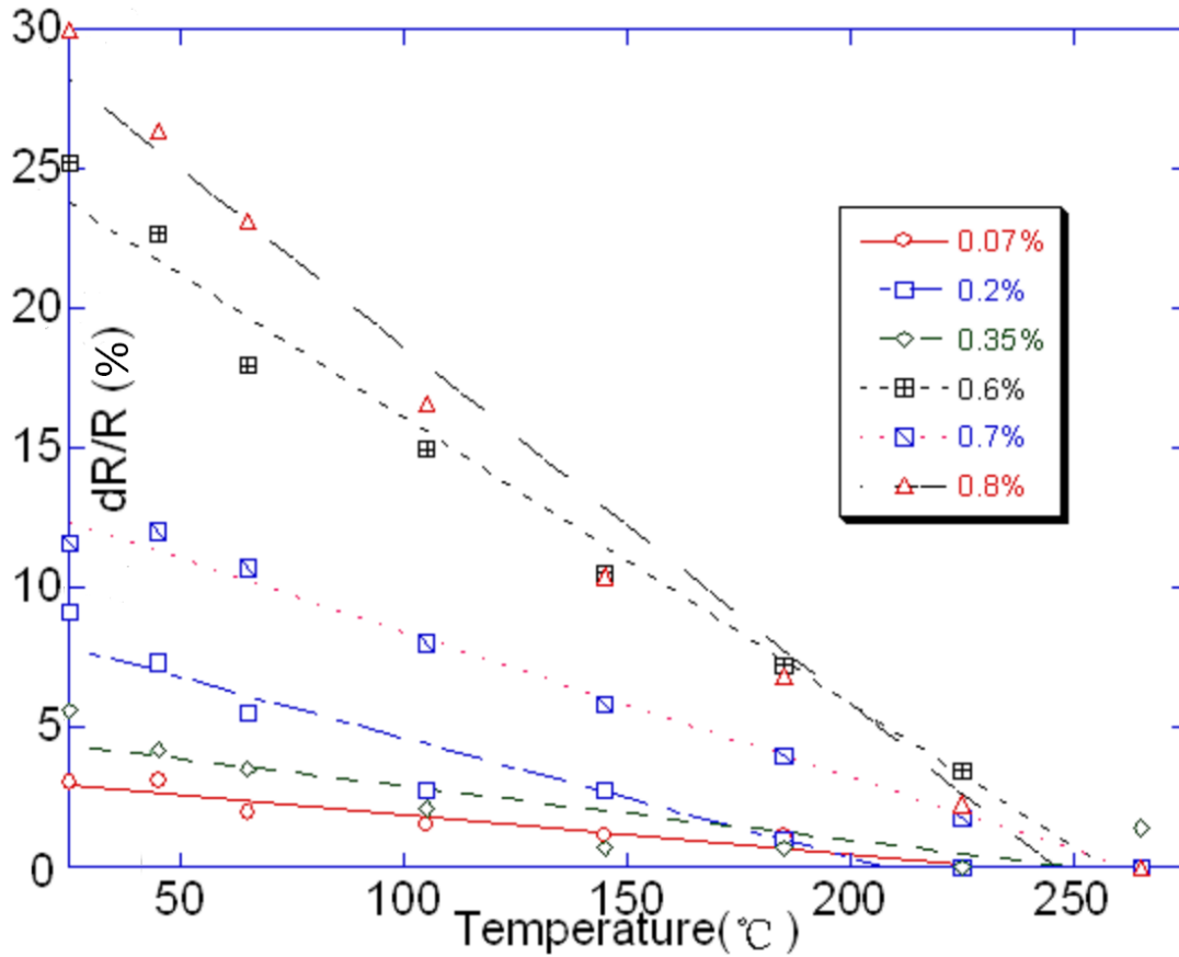
Figure 4. 20 Resistance change with temperature for nanocomposites with different CNT concentration.
