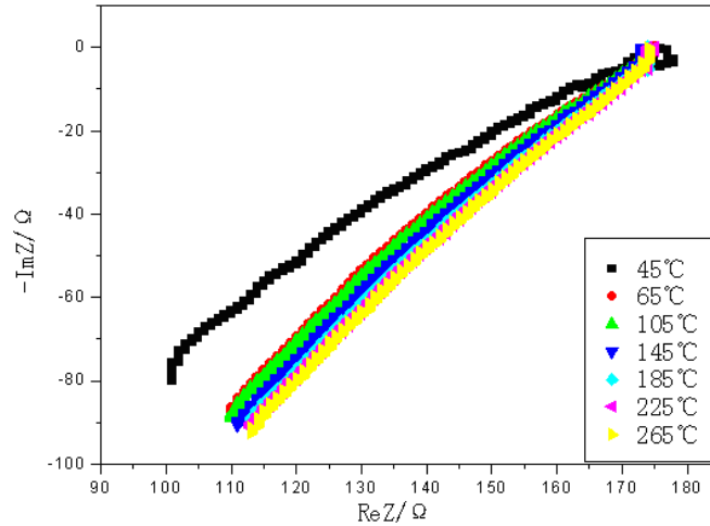
Figure 4. 17 Impedance of swcnt-polyimide composites(1.1%swcnt) at different temperature.
