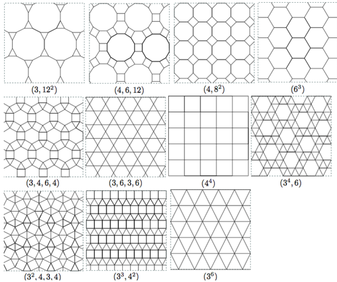
Figure 4. 1 [73] Some of the regular and Archimedean lattices.
