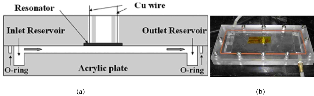
Figure 3. 11 (a) Crossessectional view of the designed experiment setup. (b) Integrated experiment setup.
