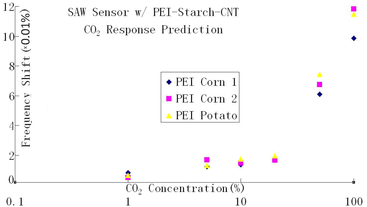
Figure 5. 21 SAW frequency shift prediction at different CO 2 concentration in log scale.
