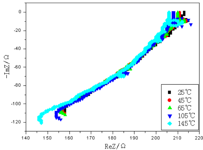
Figure 4. 18 Impedance of swCNT-polyimide composites(1.2%swCNT) at different temperature.
