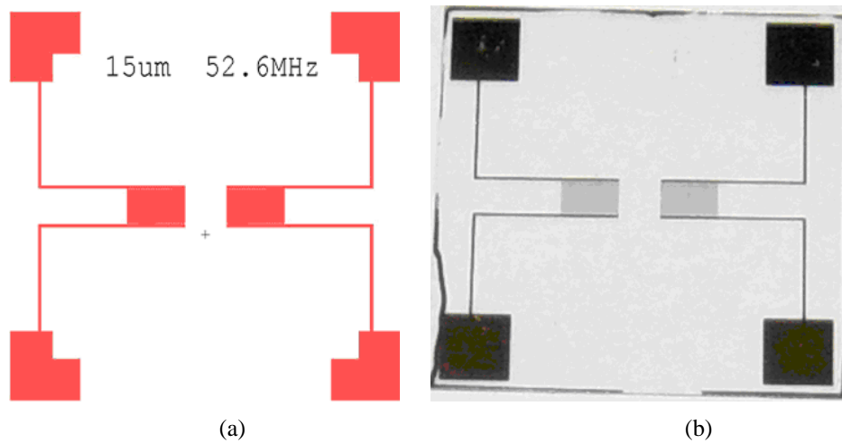
Figure 3. 10 (a) Designed SAW sensor with 15um IDT finger and space. (b) Fabricated SAW sensor on 3\text{cm} \times 3\text{cm} quartz crystal substrate
