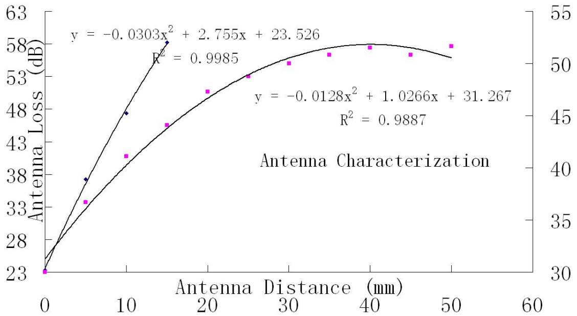
Figure 6. 23 Antenna performance summary.
