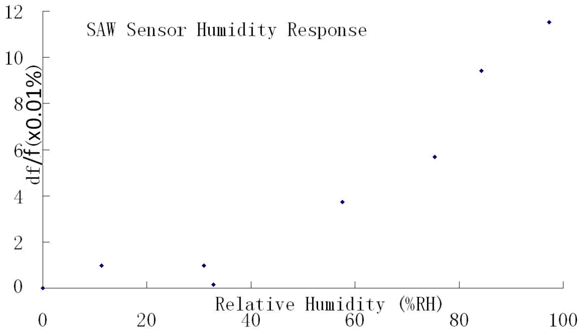
Figure 5. 27 Sensor Response to humidity.
