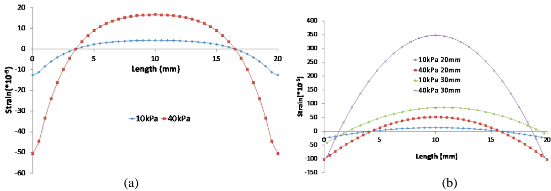
Figure 3. 7 The strain S_{11} on the central line of plate bottom from simulation and calculation. (a) FEM result for 20mm \times 20mm \times 0.3mm sensor. (b) Calculation results for 20mm \times 20mm \times 0.3mm and 30mm \times 30mm \times 0.3mm sensors.
