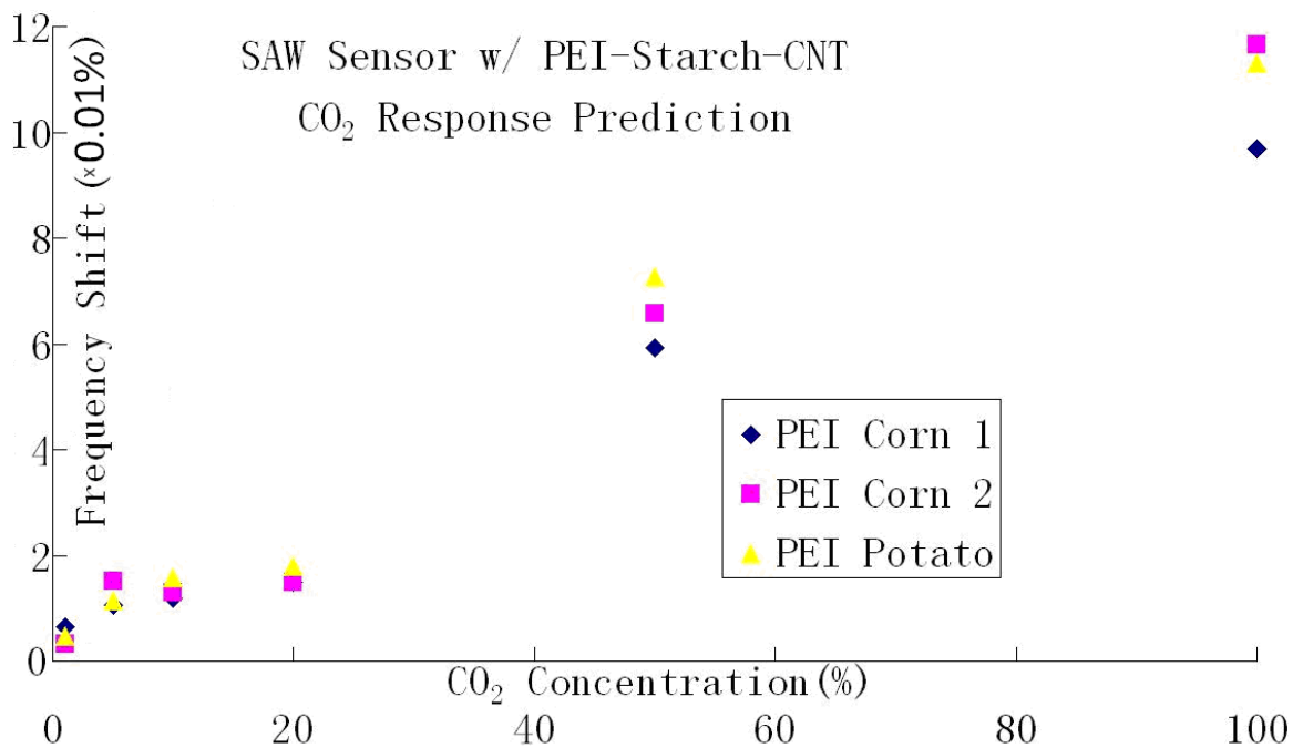
Figure 5. 20 SAW frequency shift prediction at different CO 2 concentration.
