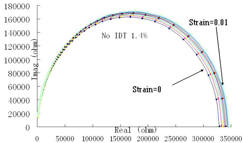
Figure 4. 26 Impedance of test sample without IDT, and with CNT concentration of 1.4%.
