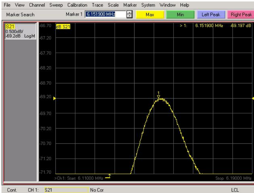
Figure 5. 33 Sensor Response 75.3%RH.
