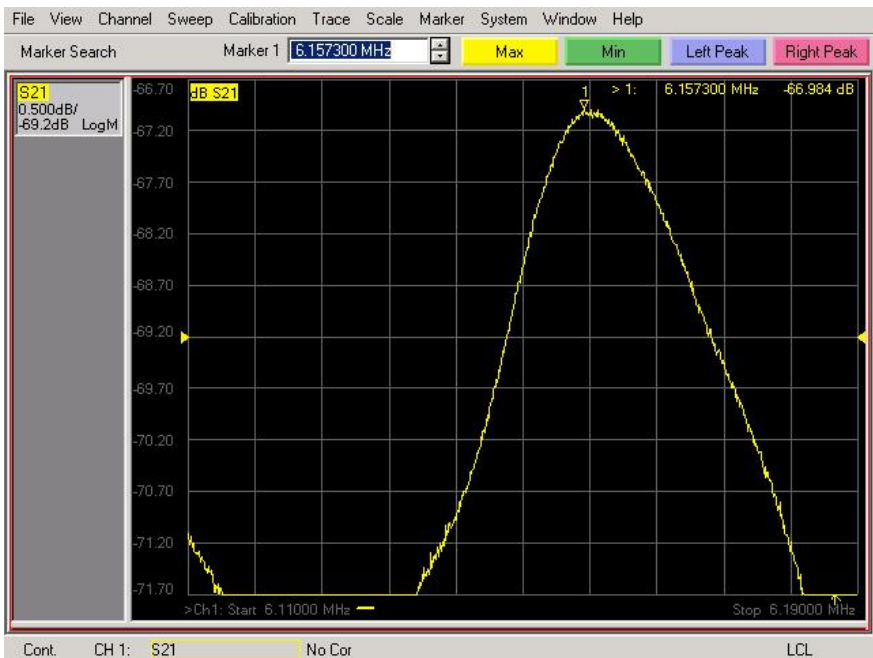
Figure 5. 30 Sensor Response 31%RH.
