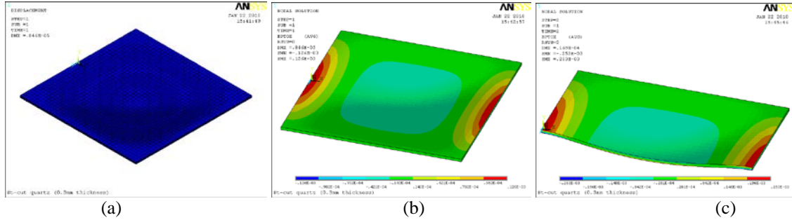
Figure 3. 6 FEM results about ST-X cut substrate under pressure. (a) Deformation under 10kPa pressure. (b) Strain S_{11} under 10kPa pressure. (c) Strain S_{11} of half plate under 20kPa pressure.
