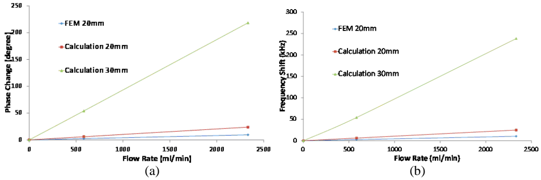
Figure 3. 8 (a) Simulated and calculated phase change versus flow rate of the chamber. (b) Simulated and calculated frequency shift versus flow rates of the chamber.
