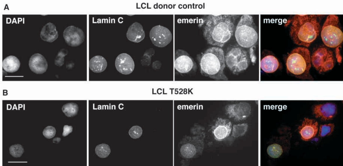
Fig. 5. The distribution of lamin C and emerin in lymphoblastoid cell lines. EBV-transformed lymphoblastoid cell lines were obtained from a donor control (row A) and from an AD EDMD patient with a single point mutation giving rise to an amino acid substitution at position T528K (row B). Each cell line was co-stained with rabbit anti-lamin C (Lamin C) and MANEM5 (emerin). The distribution of DNA in each sample was detected with DAPI. Panels show individual black and white micrographs or three-colour merged images (merge) in which the distribution of DAPI is shown in blue, lamin C in green and emerin in red/orange. In merged images, 'yellow' indicates spectral overlap between red and green signals. Bar, 10 \mu m.
