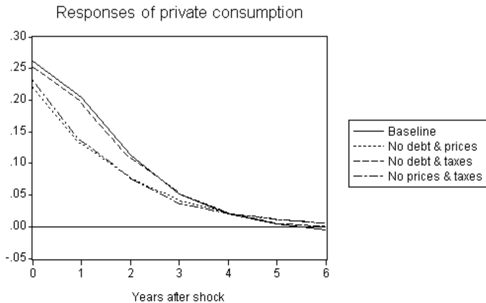
Fig. 7: robustness check, private consumption and investment responses (shock in public spending - point estimates only),
