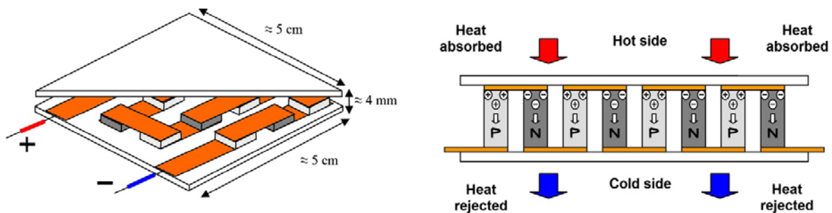
Figure 3 Seebek Cell (2).
