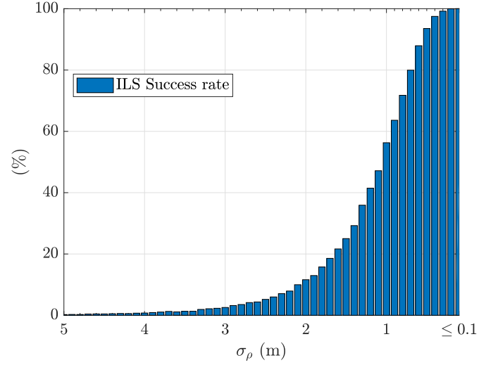
Fig. 3. Success rate for the integer parameter estimation of the RTK positioning problem.
