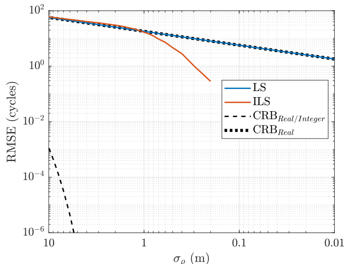
Fig. 4. Ambiguity RMSE and square-root of CRBs as a function of the standard deviation of observation noise \sigma_\rho .
