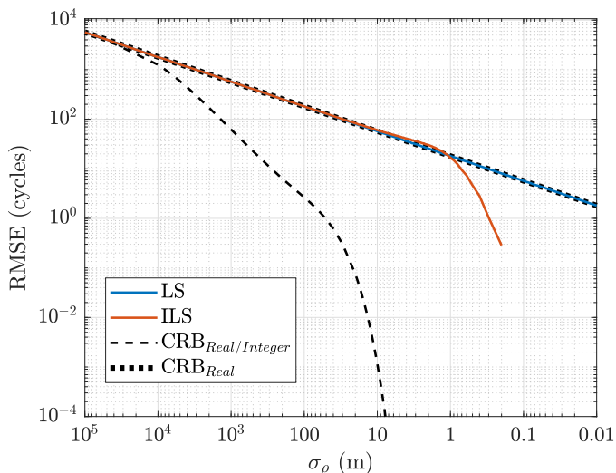
Fig. 4. Ambiguity RMSE and square-root of CRBs as a function of the standard deviation of observation noise \sigma_\rho .
