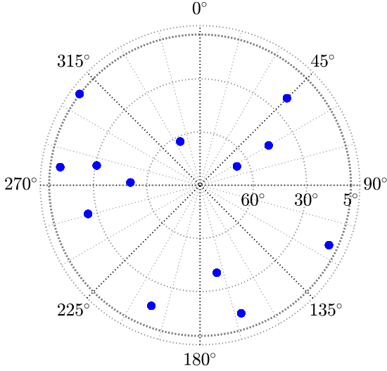
Fig. 1. Skyplot of the simulated GNSS receiver-satellite geometry.
