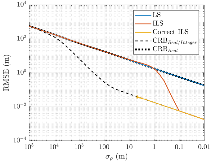
Fig. 2. Positioning RMSE and square-root of CRBs as a function of the standard deviation of observation noise \sigma_\rho .
