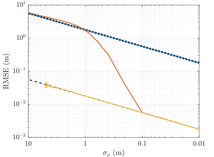
Fig. 2. Positioning RMSE and square-root of CRBs as a function of the standard deviation of observation noise \sigma_\rho .
