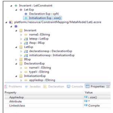
FIG. 2 – SOURCE MODEL
