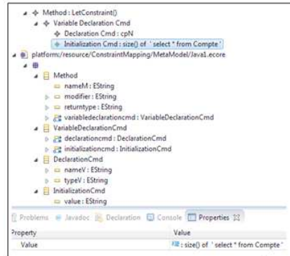
FIG. 3 – TARGET MODEL
