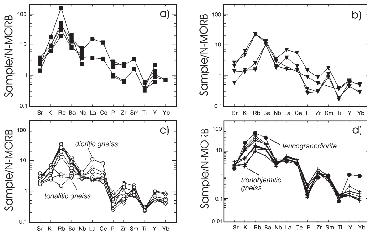
Fig. 9. Trace and incompatible element geochemical spidergrams for Nooitgedacht rocks, normalized to N-MORB, 16 showing (a) mafic dykes, (b) amphibolites, (c) dioritic and tonalitic gneisses, and (d) trondhjemites and late leucogranodiorite. Symbols as indicated in Fig. 3 caption. Note that REE data are not available for some samples in each diagram.
