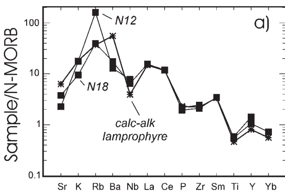
Fig. 11. NMORB-normalized spidergram (a) and REE profile (b) for selected mafic dykes and average calc-alkaline lamprophyre. 19 See text for discussion.
