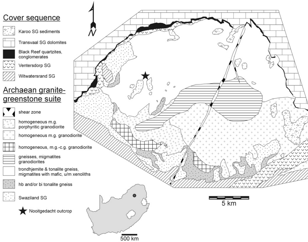
Fig. 1. General geological map of the Johannesburg Dome, modified after Poujol and Anhaeusser. 12 The location of the Nooitgedacht Migmatite Platform (Fig. 2) is indicated with a star. SG, Supergroup.
