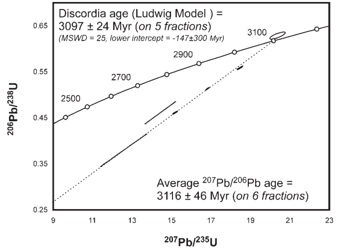
Fig. 10. U–Pb concordia diagram for pink translucent zircons only, from trondhjemitic gneiss sample location N14. 12
