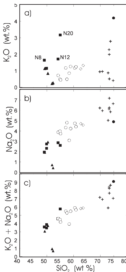
Fig. 3. Harker diagrams showing alkali compositions from Nooitgedacht. SiO 2 vs (a) K 2 O, (b) Na 2 O, and (c) K 2 O + Na 2 O. Symbols are as used by Anhaeusser: 11 filled squares, mafic dykes; filled triangles, amphibolites; open circles, dioritic gneisses; open diamonds, tonalitic gneisses; plus signs, trondhjemites; filled circles, leucogranodiorite.
