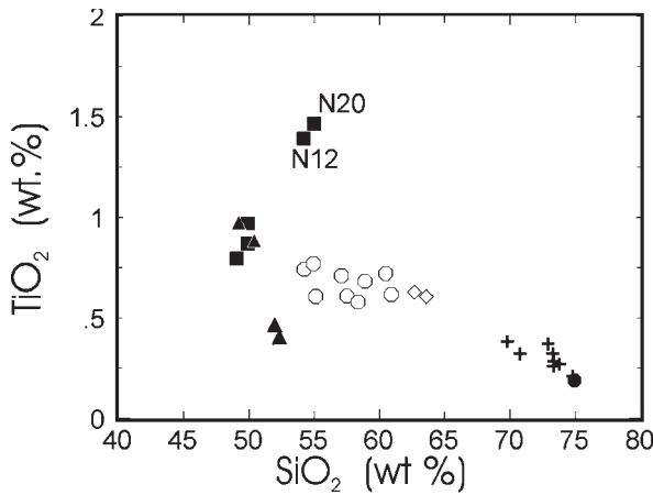
Fig. 4. SiO 2 vs TiO 2 for Nooitgedacht samples. Symbols as indicated in Fig. 3 caption.
