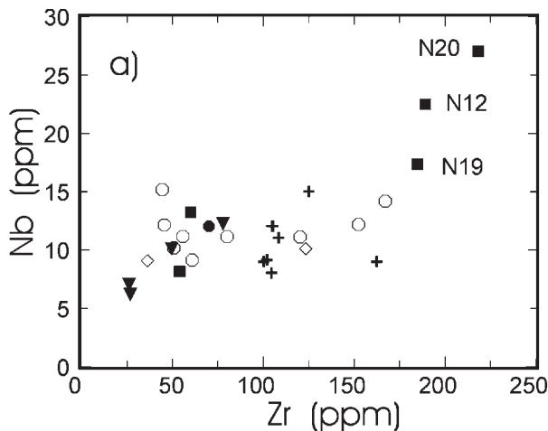
Fig. 7. HFSE variation, showing (a) Zr vs Nb, and (b) silica vs Zr/Nb ratio. Symbols as indicated in Fig. 3 caption.
