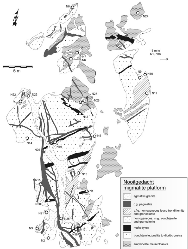
Fig. 2. Detailed geological relationships and sample locations on the Nooitgedacht Migmatite Platform. 11
