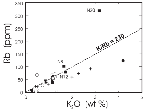
Fig. 5. K 2 O vs Rb distribution for Nooitgedacht samples. Symbols as indicated in Fig. 3 caption.
