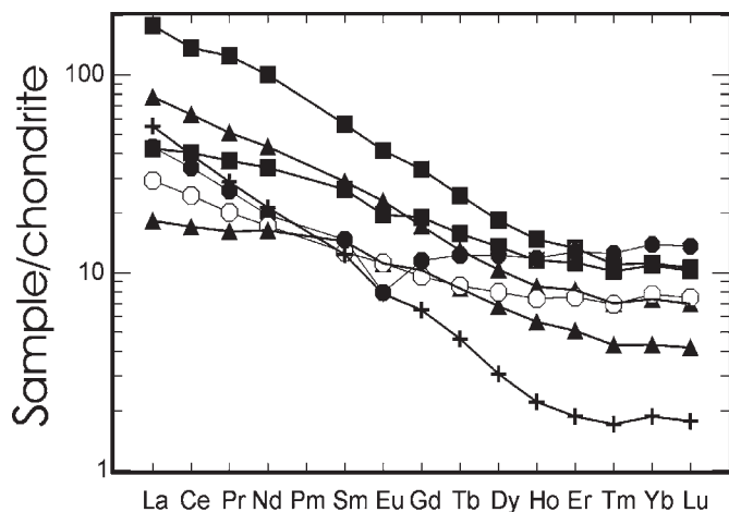
Fig. 8. Chondrite-normalized REE profiles for representative samples, 11 comparing mafic dykes (squares) with their host rocks. Symbols as indicated in Fig. 3 caption.
