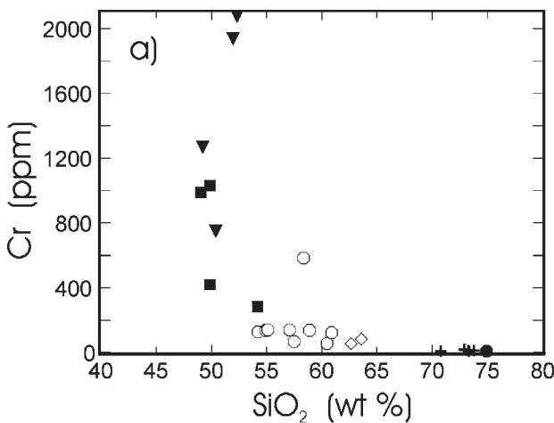
Fig. 6. Compatible transition element variation in the Nooitgedacht samples using silica vs (a) Cr and (b) V. Symbols as indicated in Fig. 3 caption.
