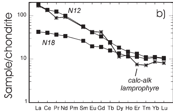
Fig. 11. NMORB-normalized spidergram (a) and REE profile (b) for selected mafic dykes and average calc-alkaline lamprophyre. 19 See text for discussion.
