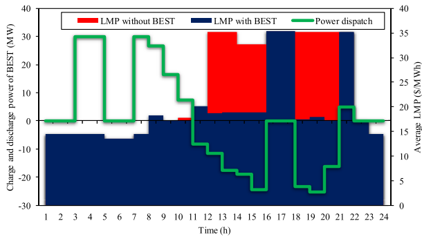
FIGURE 8. The impact of optimal hourly scheduling of the BEST system on LMP.
