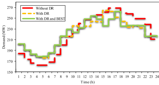
FIGURE 10. The effect of shiftable load on the hourly demand considering the carbon emission limit.
