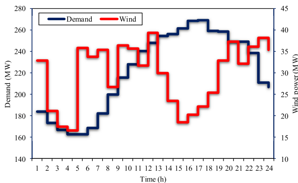
FIGURE 7. The forecasted demand and wind power.
