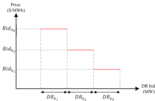
FIGURE 3. Price-sensitive shiftable demand bidding model.
