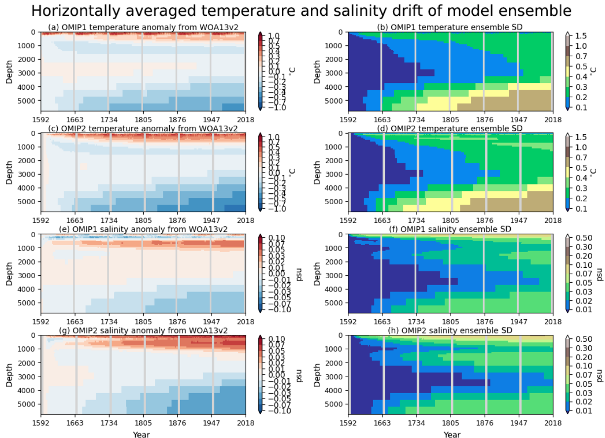
Figure 3. Globally averaged drift of multi-model mean horizontal mean (a, c) temperature ( ^{\circ}\text{C} ) and (e, g) salinity (psu) as a function of depth and time. The drift is defined as the deviation from the annual mean of the initial year of the simulation by each model. For each, time evolution of the standard deviation of the model ensemble is depicted to the right. (a, b) OMIP-1 temperature, (c, d) OMIP-2 temperature, (e, f) OMIP-1 salinity, and (g, h) OMIP-2 salinity. See Figs. S3–S6 for results of individual models.
