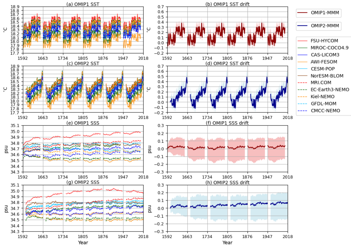
Figure 1. Drift of annual mean, global mean sea surface temperature (units in °C), and salinity (units in practical salinity units (psu)). Sea surface temperature for (a) OMIP-1 and (c) OMIP-2. Sea surface salinity for (e) OMIP-1 and (g) OMIP-2. (b, d, f, h) Multi-model ensemble mean (lines) of deviations from the annual mean of the initial year of the simulation by each model and spread defined as the range between maximum and minimum (shades) for (b) OMIP-1 and (d) OMIP-2 sea surface temperature and (f) OMIP-1 and (h) OMIP-2 sea surface salinity. The spin-up behavior of the multi-model ensemble mean in Figs. 1 to 5 is based on the following eight models which performed the full six-cycle simulations for both OMIP-1 (6 × 62 years) and OMIP-2 (6 × 61 years): AWI-FESOM, CAS-LICOM3, CESM-POP, CMCC-NEMO, EC-Earth3-NEMO, Kiel-NEMO, MRI.COM, NorESM-BLOM. See Fig. 21 for a closer look at sea surface temperature of the last cycle from individual models.
