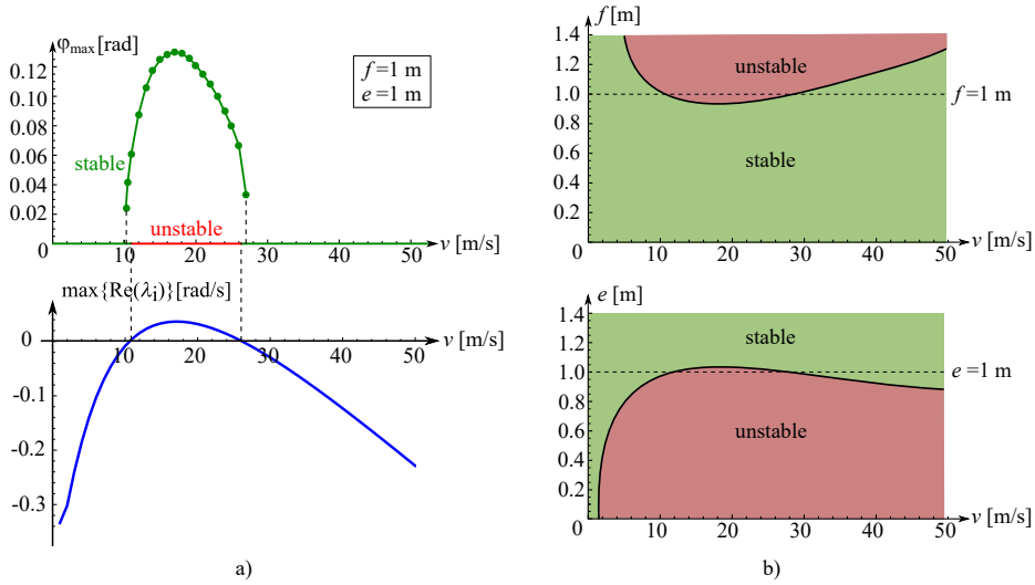
Fig. 7. a) The bifurcation diagram of the four degree-of-freedom system, in case of k = 75\,000\text{ N/m} (top panel) and the real part of the rightmost characteristic root of the linearised system (bottom panel). b) The effects of parameters f and e on the linear stability of the rectilinear motion. The green areas correspond to linearly stable, the red areas correspond to linearly unstable motion.
