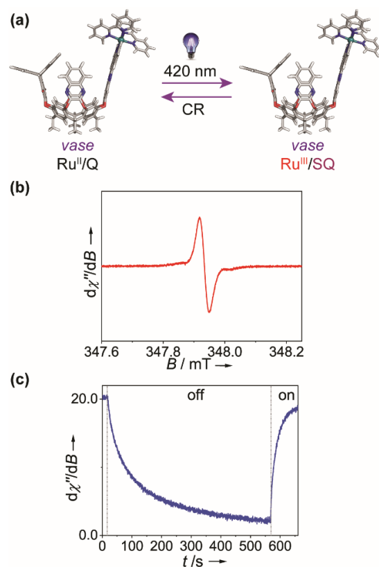
Figure 10. (a) Irradiation of 4 ( vase ) in DMF. CR: charge recombination. (b) EPR spectrum ( 2 \times 10^{-3} M in CH 2 Cl 2 , T = 298 K) after 10 min of irradiation with unfiltered light of the visible light lamp. (c) Decay and rise of the SQ signal after turning off and on the lamp.
