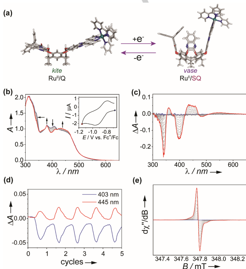
Figure 7. Electrochemical activation of cavitant 4 . (a) Schematic of the switching. (b) UV-Vis-NIR spectroelectrochemistry in the potential region of the first reduction step in 0.2 M n\text{-}(Bu)_4PF_6/CH_2Cl_2 measured at T = 293 K with a scan rate of 0.01 Vs^{-1} . (c) Differential UV-Vis-NIR spectra. (d) Difference absorbance at selected wavelengths showing the redox switching over five successive CV cycles. (e) EPR spectra. Inset in (b) shows the cyclic voltammogram and the potential (colored circles) at which the EPR and UV-Vis-NIR spectra were taken.
