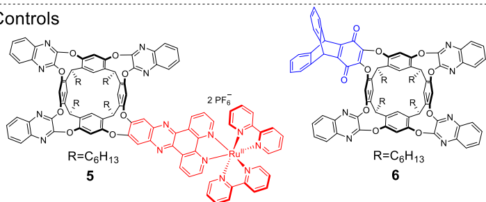
Figure 2. (a), (b) Chemical structures of \text{Ru}^{\text{II}} -based resorcin[4]arene cavitants 1-5 and control 6 . *Only for cavitants 3 and 4 . (c) Redox equilibrium between quinone ( Q ) and semiquinone radical anion ( SQ ).
