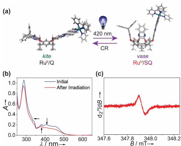
Figure 9. Light-activation of cavitant 4 in CH 3 CN without sacrificial donor. (a) Schematic of the kite-vase switching. CR: charge recombination. (b) UV-Vis absorption spectra of 4 ( 1 \times 10^{-5} M in CH 3 CN) before and after 15 min of irradiation at 420 nm in photoreactor at T = 298 K. (c) EPR spectrum of 4 ( 2 \times 10^{-3} M in CH 2 Cl 2 ) after 10 min of in-situ irradiation with unfiltered light of the visible light lamp at T = 298 K.
