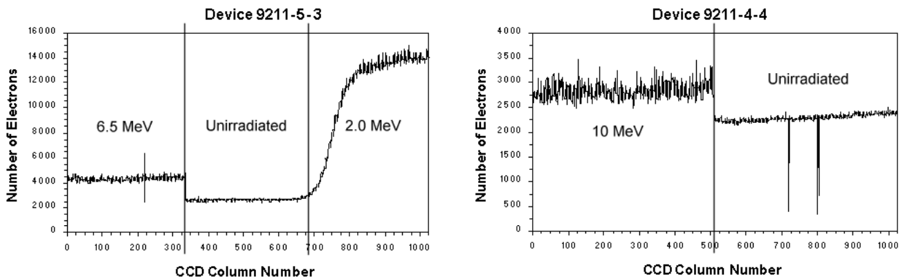
Fig. 3: Plots of the sum average of 1000 rows in the image section of each CCD showing the increase in dark current and generation of bright pixels as a result of each irradiation.
