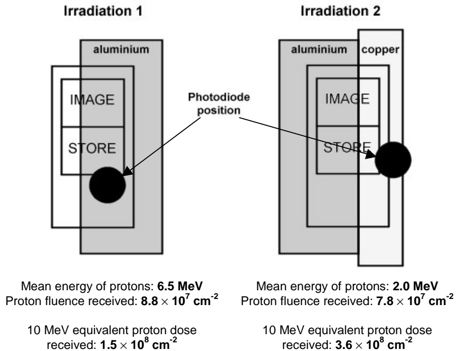
Fig. 1: This diagram shows the irradiated areas of the CCD47-20 (9211-5-3) and the dose each area received. Also shown is the position of the photodiode for each irradiation.
