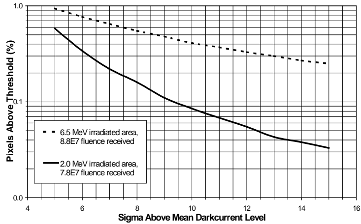
Fig. 4: The percentage of CCD pixels in each irradiated area with a charge level greater than a given threshold level above the mean background dark current.
