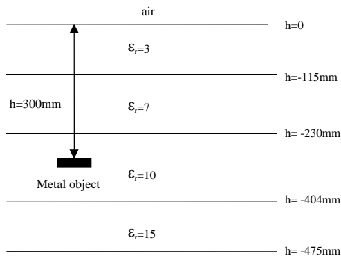
Fig. 4. Stratified media model
