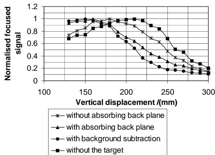
Fig. 2. Vertical focusing through target location
