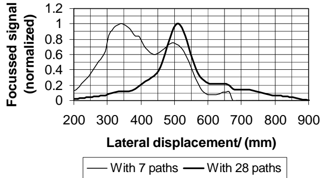
Fig. 5. Lateral focusing with 7 and 28 paths
