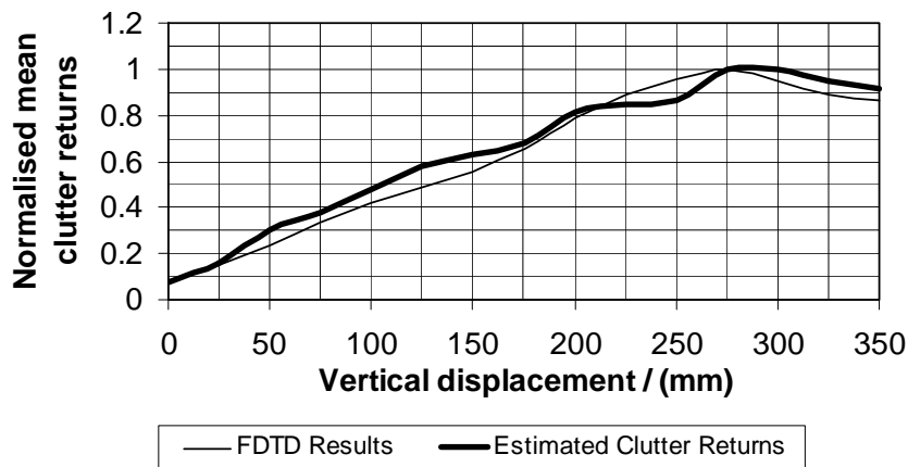
Fig. 3. Comparison of FDTD clutter echoes with the estimated clutter
