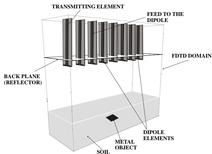
Fig. 1. FDTD Model of a PRSF-SPR system
