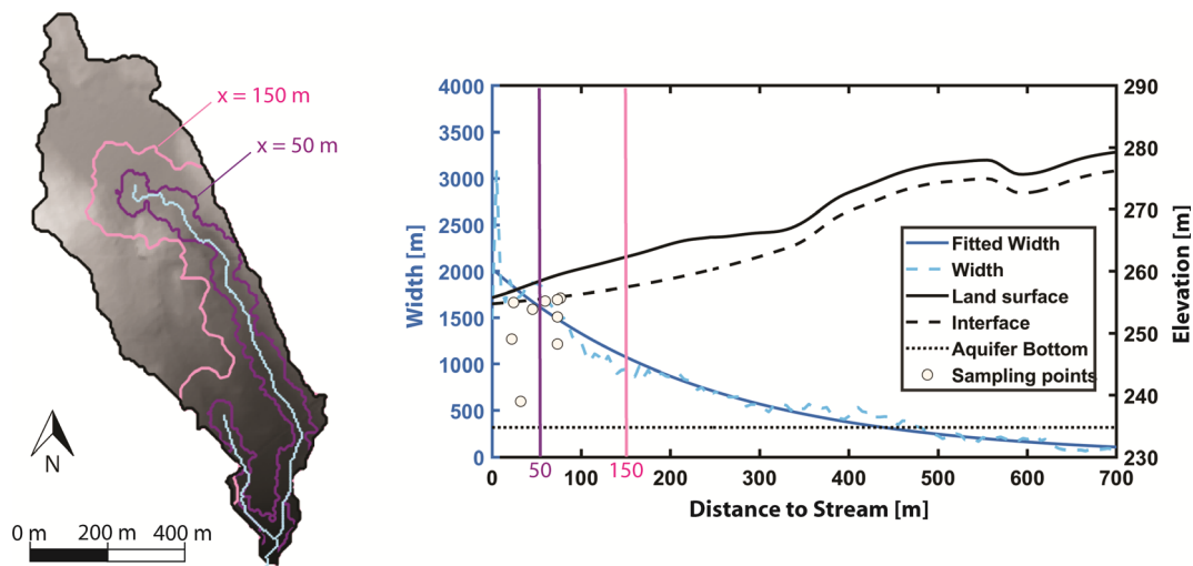
FIGURE 2 From the Svartberget catchment (inset to the left), we extracted a representative hillslope with elevation (solid black line) plotted against the distance to the stream. Also plotted are the interface between the shallow permeable and deeper less permeable layer (black, dashed line), the bottom of the aquifer (black, dotted line) as well as the width of the hillslope (blue, dashed line) and the fitted width (blue solid line). The elevations of sampling locations are marked with open circles at the respective distances of the sampling from the stream
