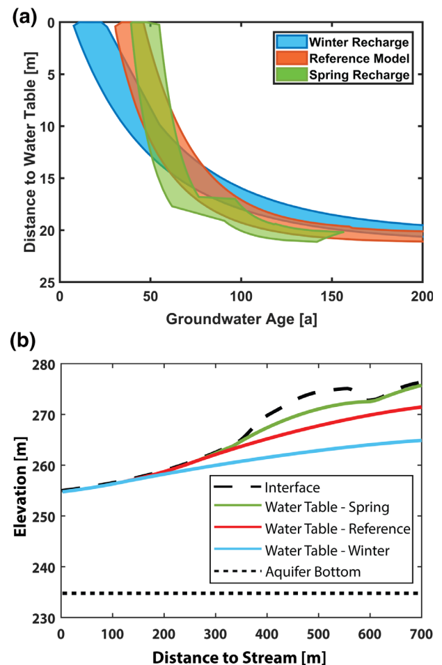
FIGURE 7 (a) Groundwater age stratifications within the distances of 80 to 20 m to the stream are shown for different recharge rates (blue: winter model, red: reference model, green: spring model). (b) Water table locations for the winter model (blue), the reference model (red) and spring model (green). The dashed line represents the interface between the shallow permeable layer and the deep less permeable layer. The dotted line shows the aquifer bottom
