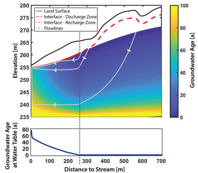
FIGURE 5 Distribution of groundwater ages within the representative hillslope. The red line shows the interface between the shallow permeable layer and deeper less permeable layer. The red dashed line indicates the locations at which recharge to the aquifer takes place. The red continuous line indicates the extent of the subsurface discharge zone
