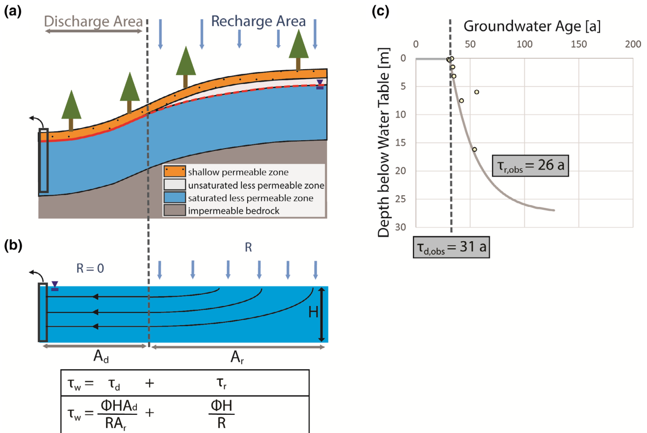
FIGURE 6 (a) Graphical presentation of the representative hillslope and generation of the discharge zone in the discharge area. (b) Presentation of the idealized aquifer and mean groundwater ages. (c) Measured groundwater ages versus depth and derived mean groundwater ages
