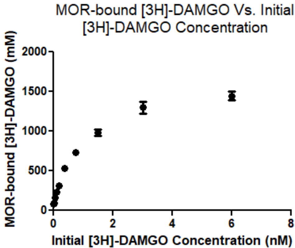
Figure 10: Saturation Binding Assay Curve. Binding curve of Initial [3H]-DAMGO Concentration vs [3H]-DAMGO bound to Mu Opioid Receptors (MOR).
