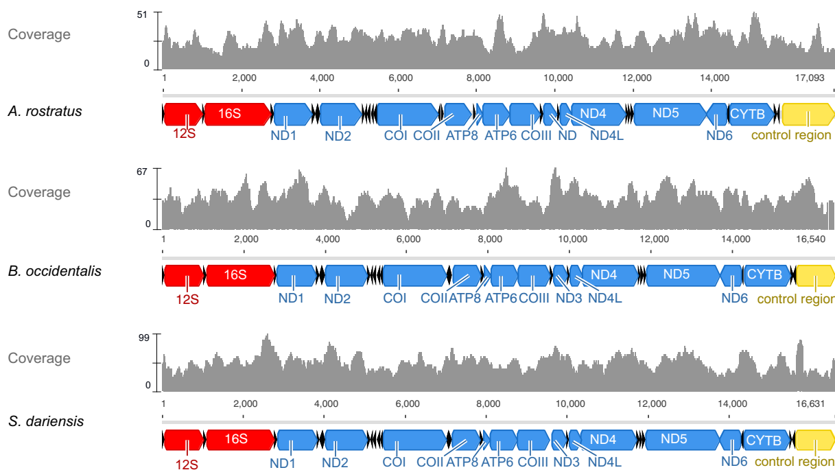
Fig. 1. Structure and read coverage of the assembled mitogenomes of A. rostratus , B. occidentalis and S. dariensis . Gray (Coverage) plots show the read depth across the complete mitogenomes. Direction of gene transcription for each species is indicated by the arrows: rRNA genes (red), PCGs (blue), tRNA genes (black) and the control region (yellow). PCG and rRNA genes are shown with standard abbreviations. (For interpretation of the references to colour in this figure legend, the reader is referred to the web version of this article.)
