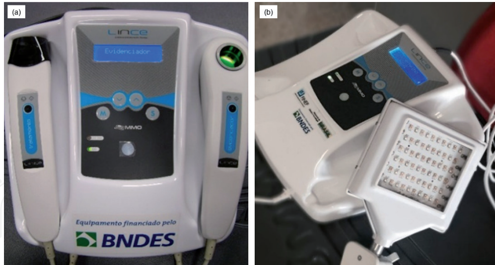
Figure 1. (a) LINCE® equipment (MMOptics – Brazil): left - treatment system emitting at 630 nm; right - diagnostic system emitting at 405 \pm 10 nm. (b) Square illumination of the LINCE® accessory emitting at 630 \pm 10 nm.
