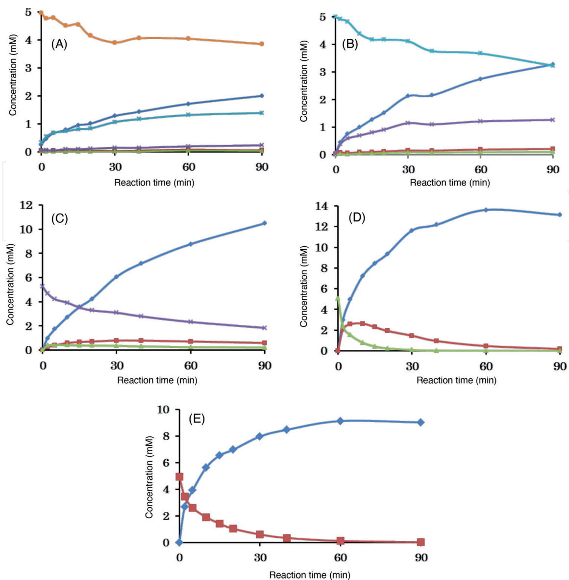
Figure 4. HPLC analysis of products of hydrolysis of chitin oligosaccharides ( (GlcNAc)_3 to (GlcNAc)_6 ) by recombinant Pb-GlcNAcase . The degradation products of (A) (GlcNAc)_6 , (B) (GlcNAc)_5 , (C) (GlcNAc)_4 , (D) (GlcNAc)_3 , and (E) (GlcNAc)_2 by the enzyme were detected by HPLC, as described in the materials and methods. Lines: GlcNAc (dark-blue line), (GlcNAc)_2 (red line), (GlcNAc)_3 (yellowish olive-green line), (GlcNAc)_4 (purple line), (GlcNAc)_5 (light-blue line), (GlcNAc)_6 (mustard-yellow line).
