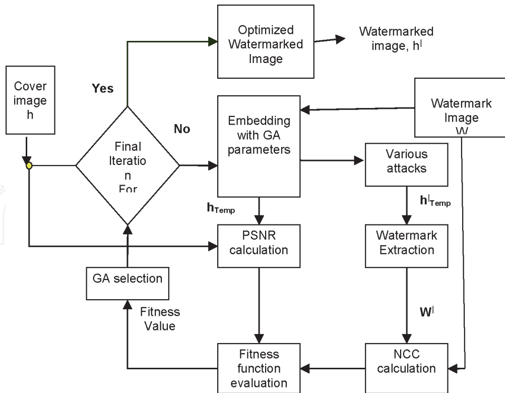
Figure 1. Flow chart for GA based watermark embedding.
