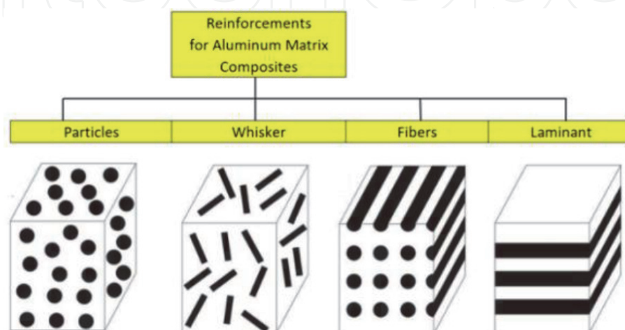
Figure 2. Reinforcement types.
