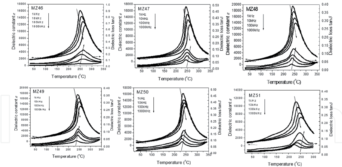
Figure 13. Temperature dependence of relative dielectric constant \epsilon and dielectric loss \tan \delta of samples at different frequencies: MZ46 (Zr/Ti = 46/54), MZ47 (Zr/Ti = 47/53), MZ48 (Zr/Ti = 48/52), MZ49 (Zr/Ti = 49/51), MZ50 (Zr/Ti = 50/50), and MZ51 (Zr/Ti = 51/49).
