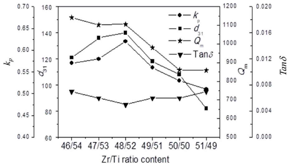
Figure 16. The values of k_p , d_{31} , Q_m , and \text{tan } \delta of the PZT-PZN-PMnN ceramic samples.
