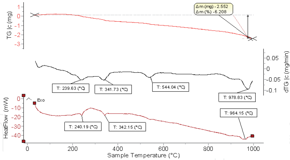
Figure 2. TG and DTA curves of (Zn,Mn)Nb_2(Zr,Ti)O_6 power at 10^\circ\text{C}/\text{min} heating rate.
