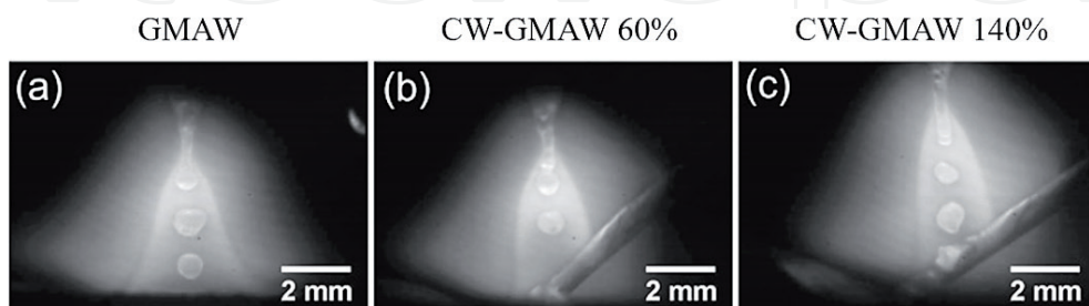
Figure 14. Influence of the addition of additional wire on the cathode point of the arc: (a) represents the GMAW process, and (b) and (c) represent CW-GMAW welding with the addition of 60 and 140% additional wire, respectively.
