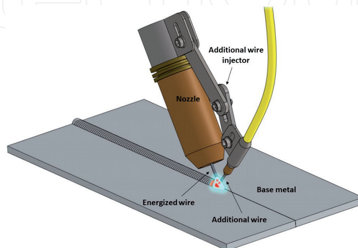
Figure 9. CW-GMAW process scheme.
