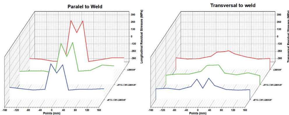
Figure 11. Comparative between longitudinal and transverse RS with GMAW and CW-GMAW measuring by XRD.
