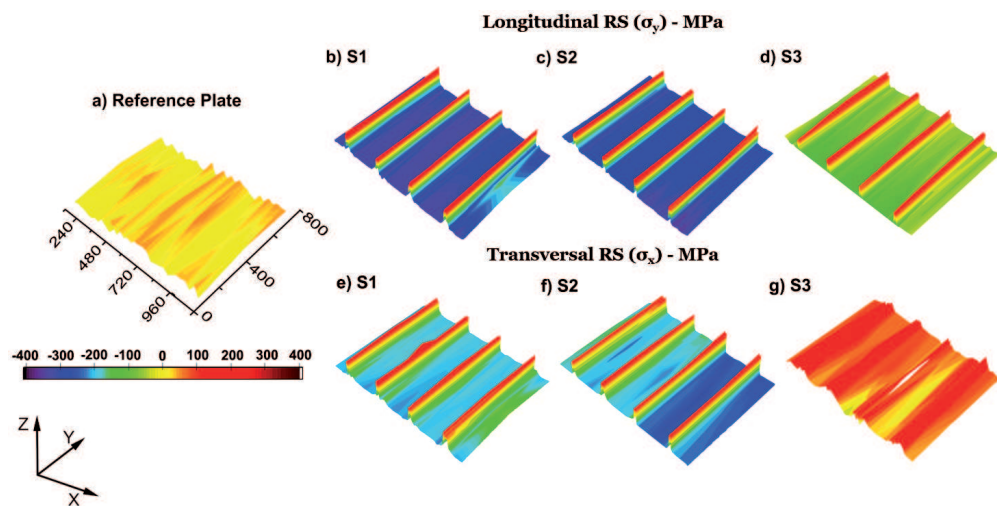
Figure 6. TRs values in the 3D perspective for (a) reference plate; (b) sequence 1; (c) sequence 2; (d) sequence 3 in the longitudinal direction; (e) sequence 1; (f) sequence 2; and (g) sequence 3 in the transverse direction.
