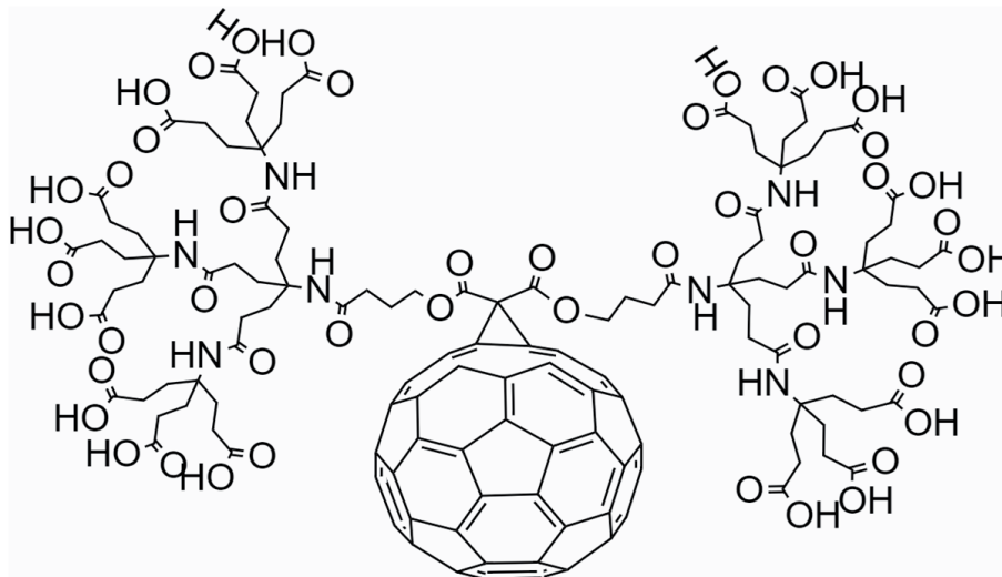
Figure 2. Poly-carboxylated (18) Fullerene.
