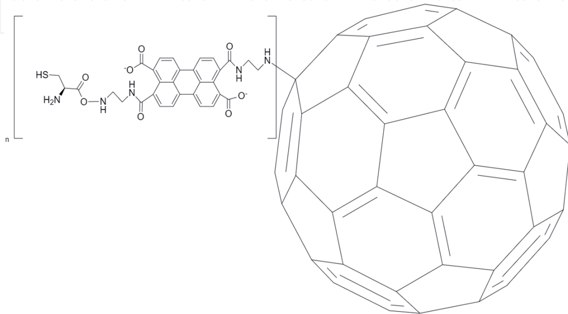
Figure 7. SH and \text{NH}_2 modified PTC- \text{NH}_2 - C_{60} .
