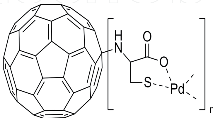
Figure 4. Palladium nanoparticles and cysteine modified fullerene particles (Pd@Cys-C 60 ).
