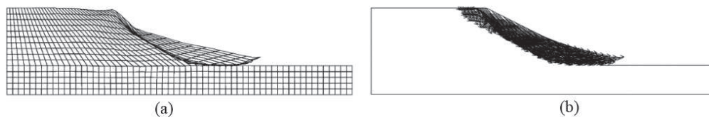
Figure 3. (a) Deformed mesh of a homogeneous slope with a foundation layer; (b) nodal displacement vectors.
