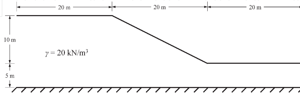
Figure 1. Homogeneous slope with a foundation layer.
