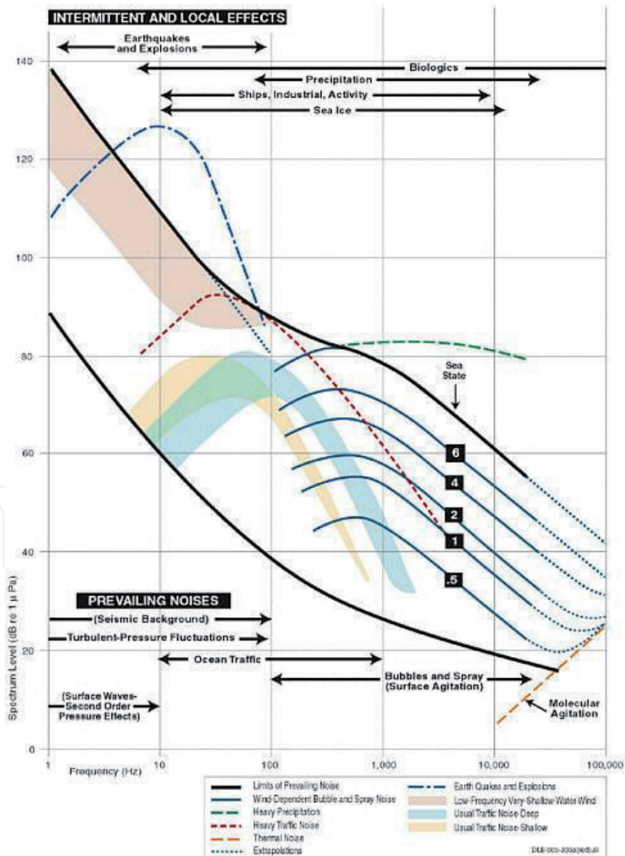
Figure 1. Wenz curve [11].
