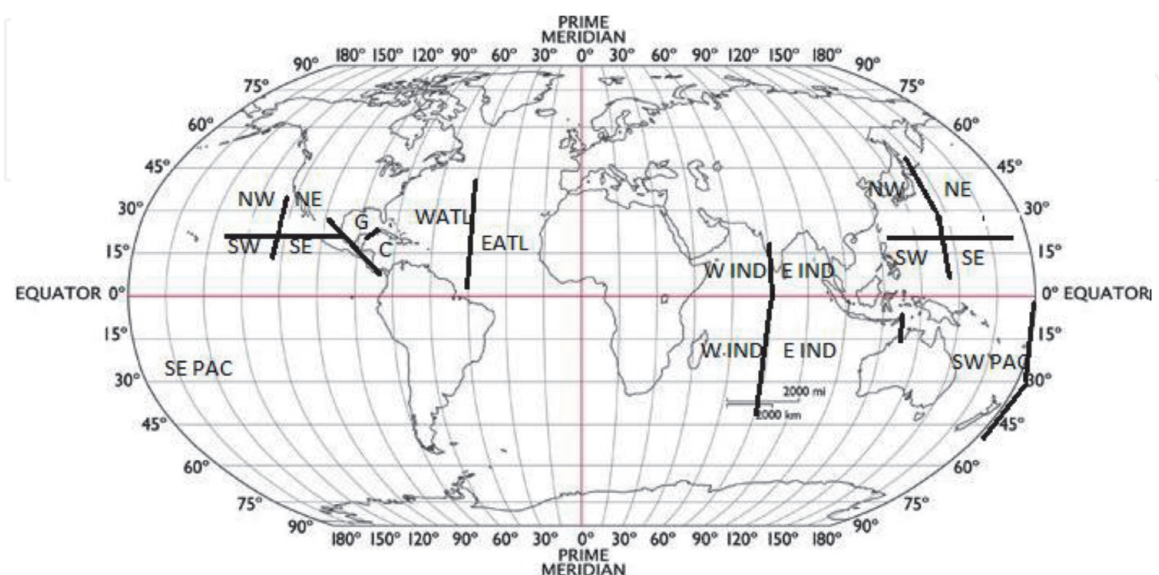
Figure 1. The globe with the borders of each subregion for the North Atlantic (G = Gulf of Mexico, and C = Caribbean), East Pacific ( 125^{\circ}\text{W} 20^{\circ}\text{N} ), West Pacific ( 140^{\circ}\text{E} 20^{\circ}\text{N} ), northern Indian ( 75^{\circ}\text{E} ), and southern hemisphere ( 75^{\circ}\text{E} in the Indian and 180^{\circ} in the Pacific).
