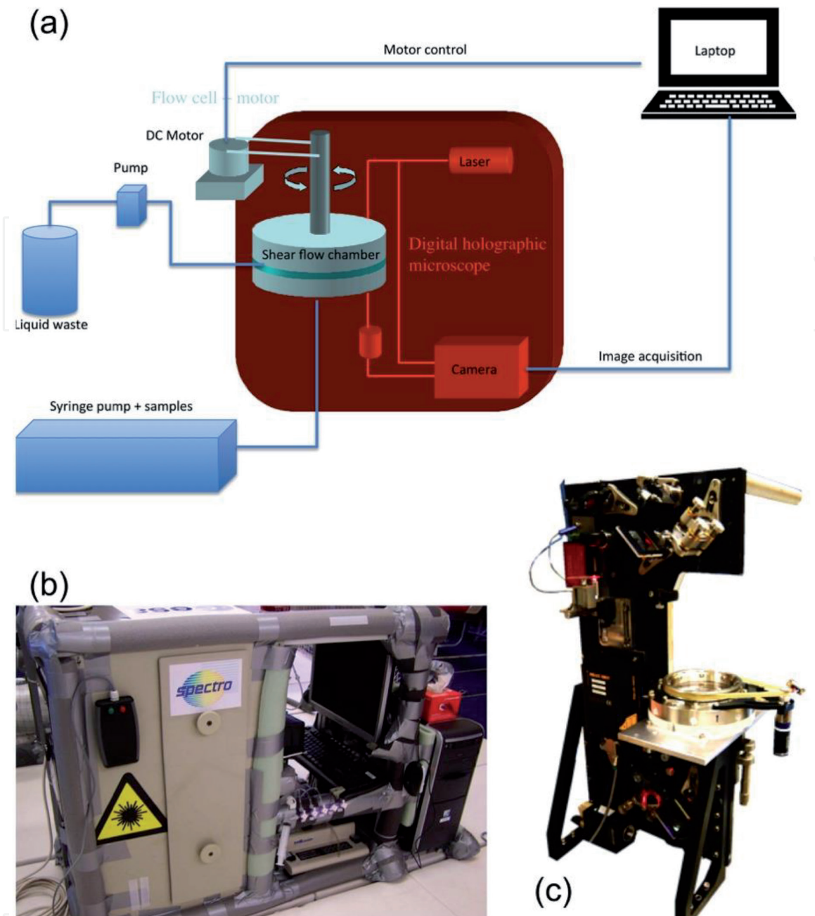
Figure 3. (a) Design principle of the parabolic flight setup used for BIOMICS experiments. The shear flow chamber is installed on a digital holographic microscope that allows 3D reconstruction of vesicle and red blood cell suspensions in flow. Samples are injected thanks to a multi-channel syringe pump; (b) parabolic flight experimental rack, 2006 version; (c) digital holographic microscope designed and developed at MRC, ULB.
