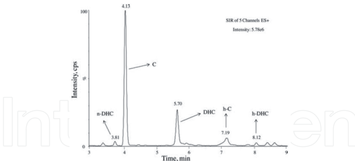
Figure 8. UPLC-MS chromatogram showing different capsaicinoids extracted from red chili.
