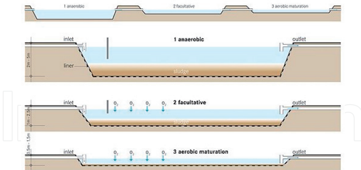
Figure 3. Layout of typical waste stabilization pond system showing design of all three treatment stages.
