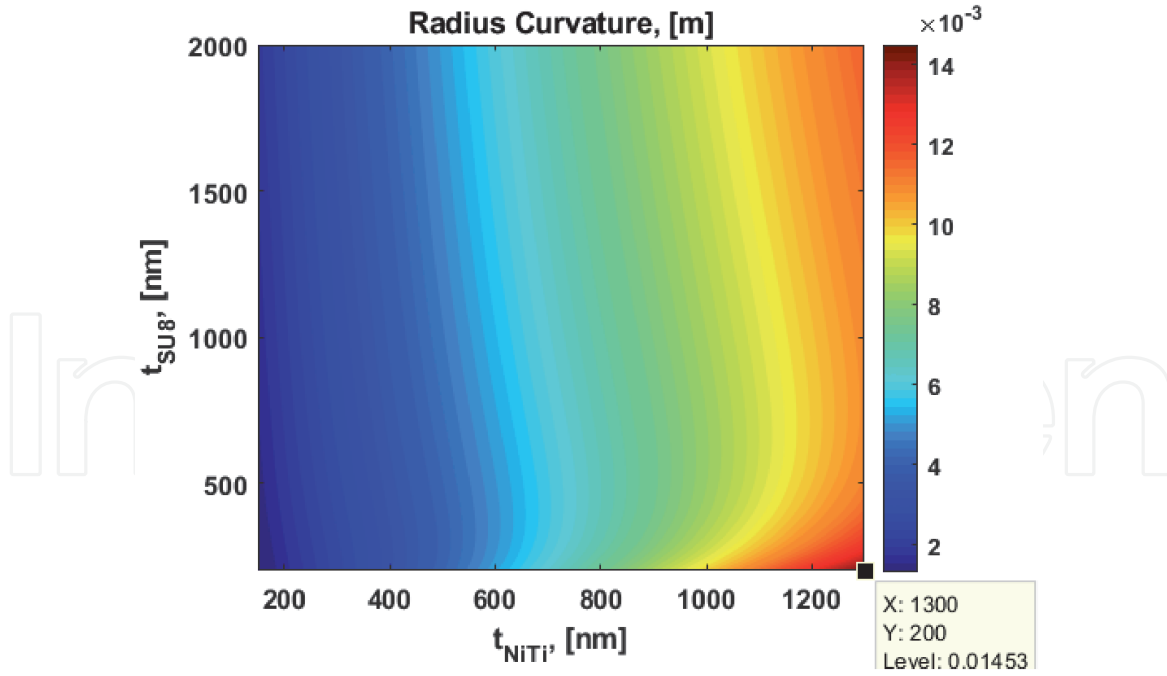
Figure 5. MATLAB-generated contour plot of curvature radius (m), against the primary design variables (i.e., t_{NiTi} and t_{SU-8} ). Curvature radius is maximized for the thickest values of NiTi and thinnest values of SU-8. The result is intuitive because this is the stiffest beam (from the perspective of thickest NiTi with much larger Young's modulus compared to SU-8). Thinner SU-8 means the effect from strain differential and CTE mismatch is minimized and contributes less to curvature radius. Overall, this means that upper bound on NiTi thickness and lower bound on SU-8 thickness are active constraints for objective function 2.
