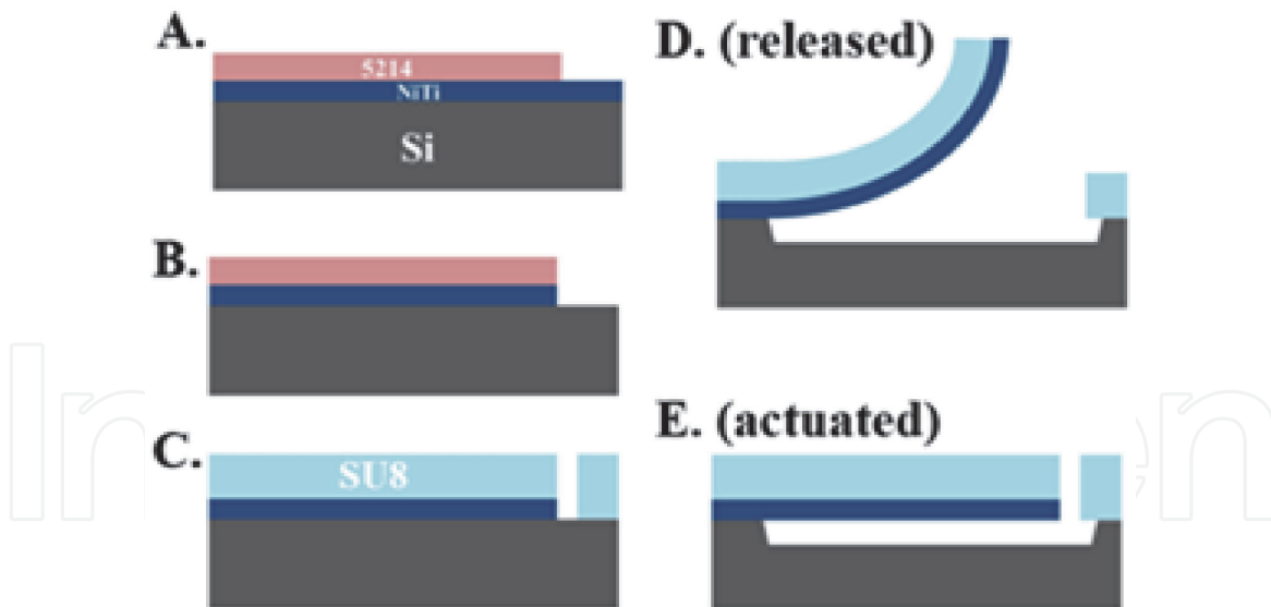
Figure 2. SMA MEMS fabrication process for SU-8 on NiTi bimorph.
