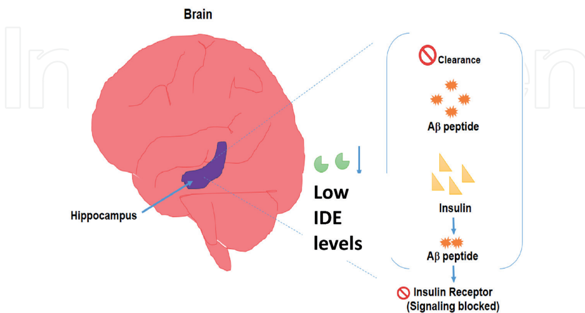
Figure 2. Abnormal clearance of toxic species of \beta -amyloid by insulin degrading enzyme. Hippocampus with decreased levels of insulin degrading enzyme (IDE) leads to A\beta accumulation, which blocks the insulin receptor signaling, altering synaptic plasticity and architecture of dendritic spines.
